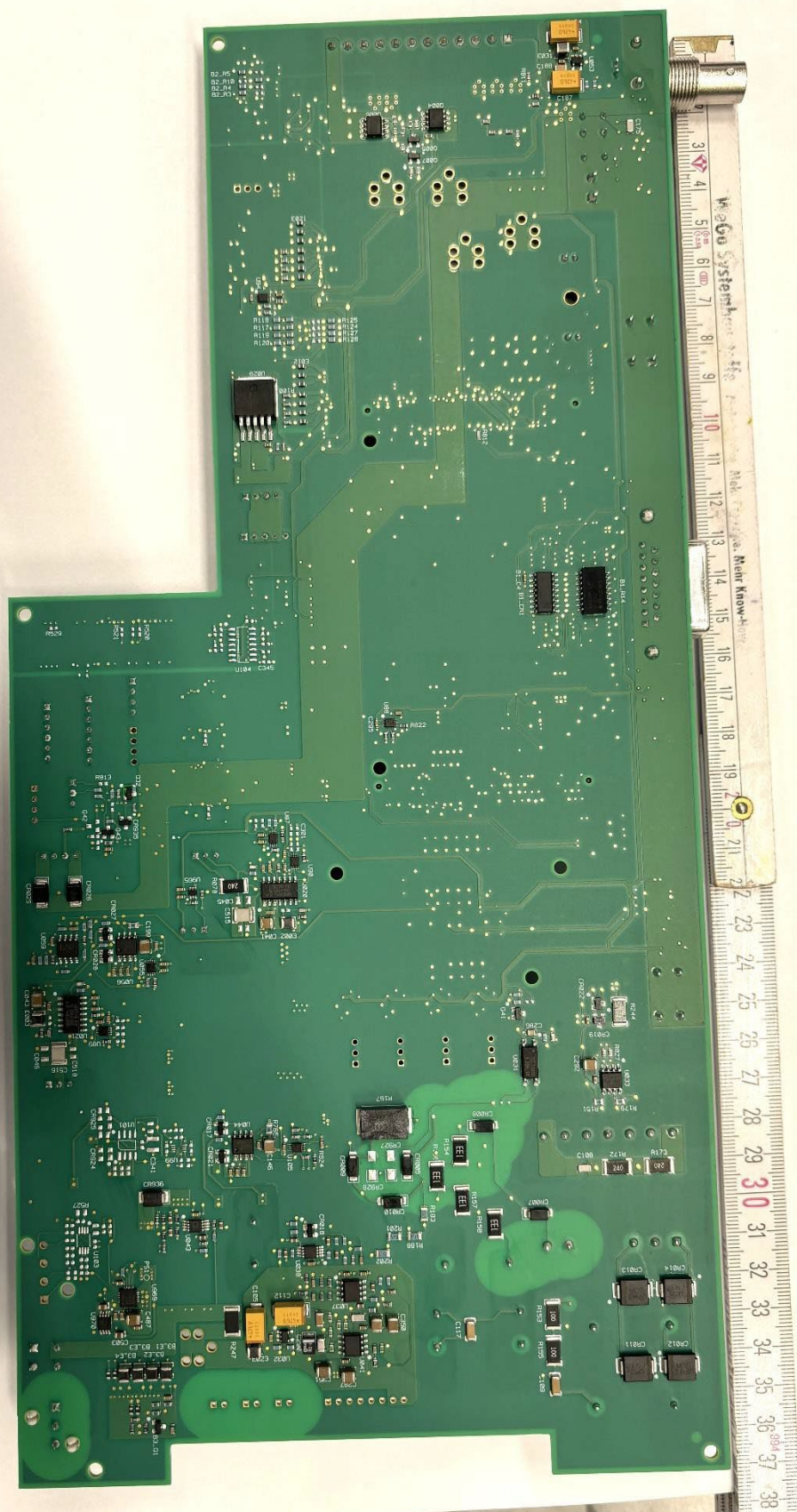
Main-Board bottom
