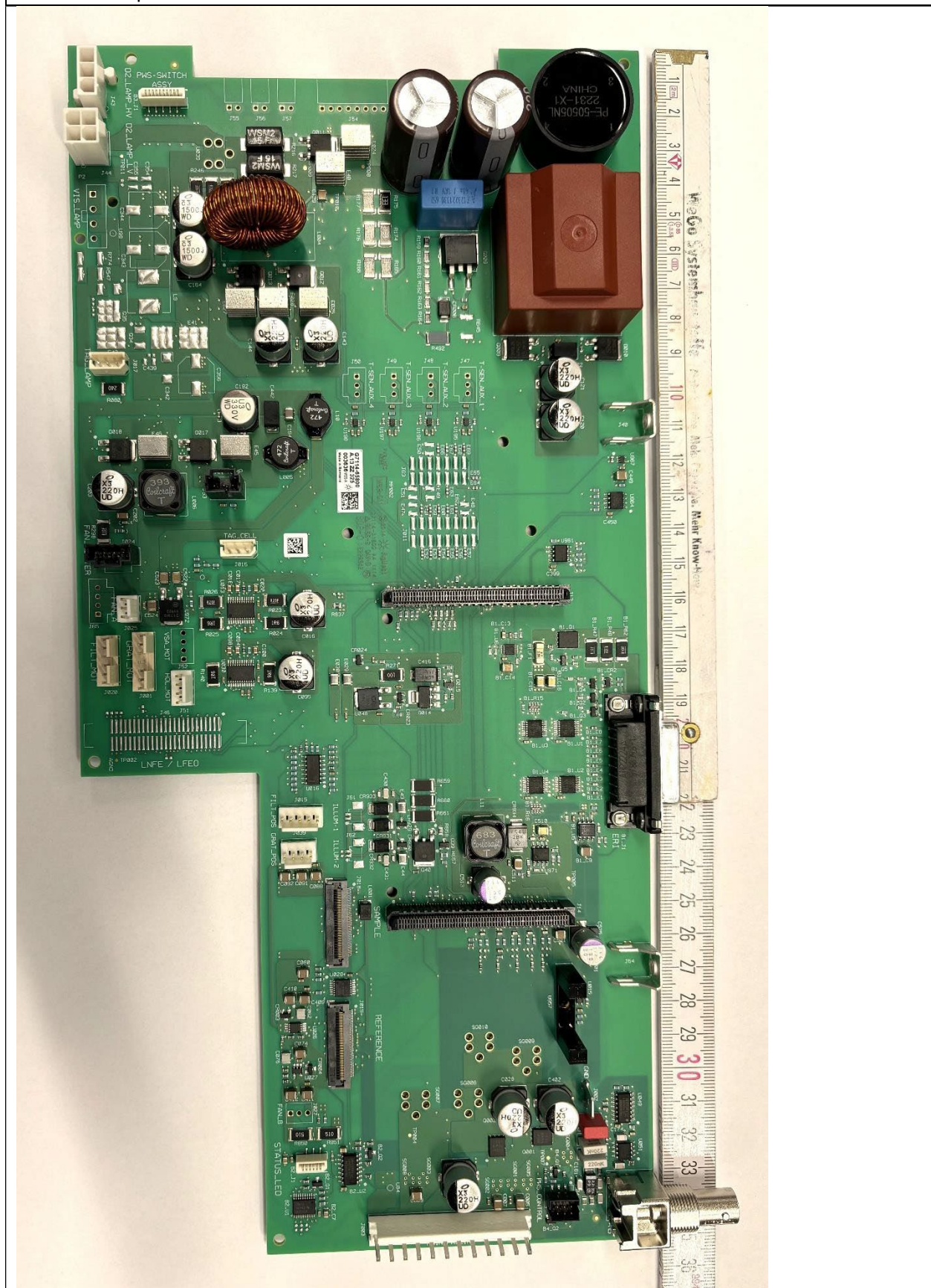
Main-Bord top
