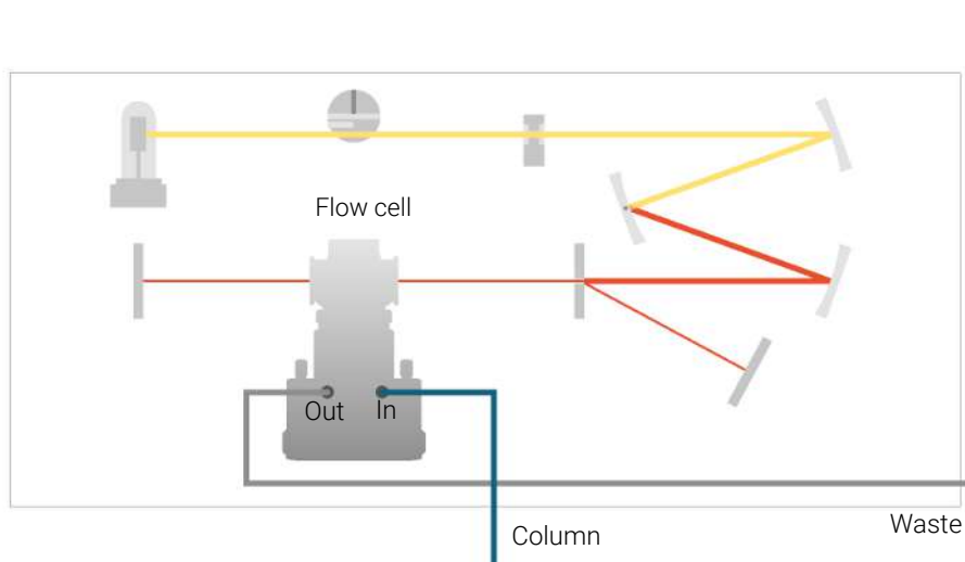
Figure 4: Hydraulic path
