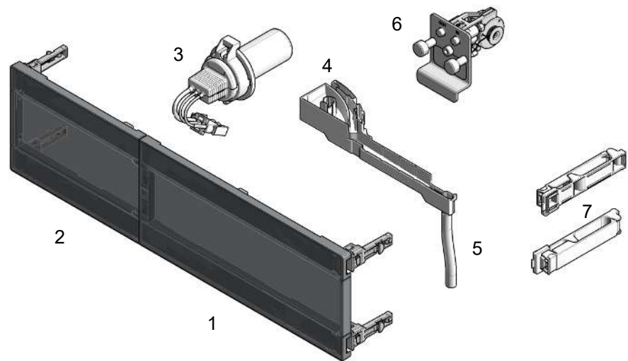
Figure 39: Maintenance Parts
