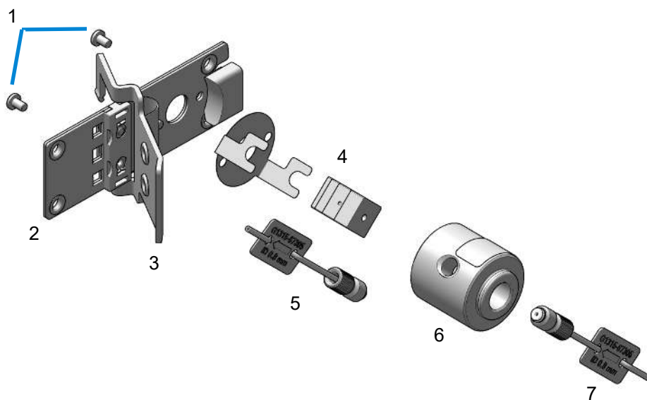
Figure 59: Prep Flow Cell - Quartz Parts
