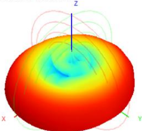
5850.0MHz H+V, Eff: 71.3%
