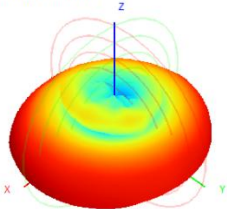
5500.0MHz H+V, Eff: 65.7%
