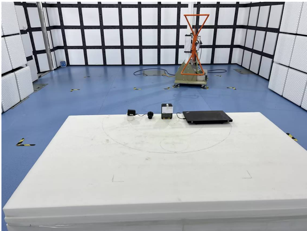
Radiated Emission Front View(30MHz-1GHz)
