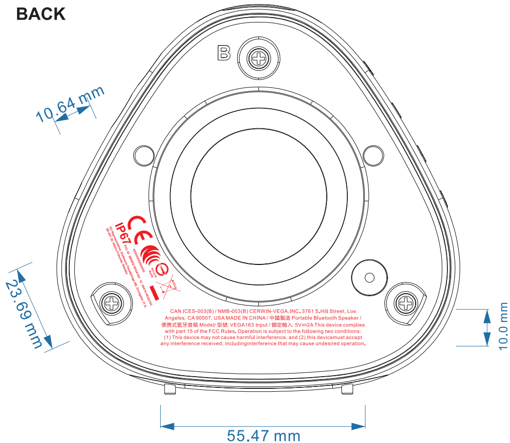
VEGA163-Back Drawing Finished: White silkscreen Color: White
