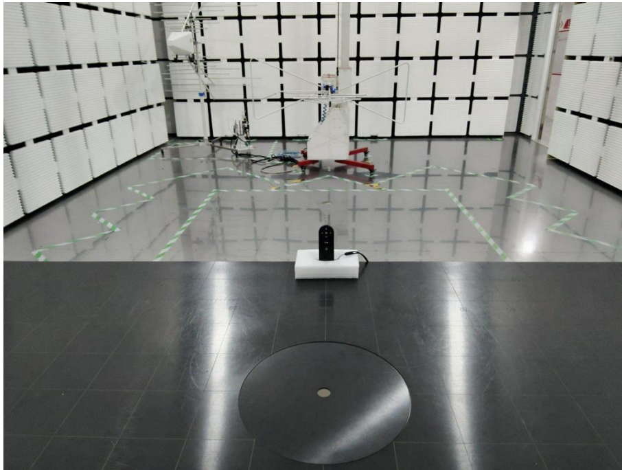
Field Strength of The Fundamental Signal Radiated Emission (below 1GHz)
