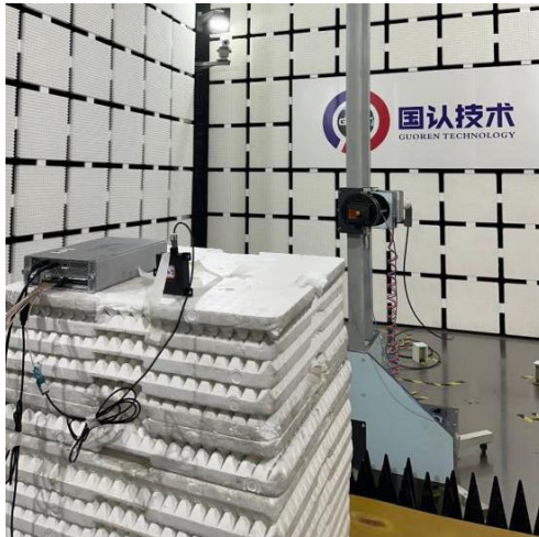
Fig.4(60-90GHZ)
