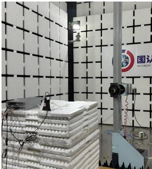
Fig.5(42-60GHZ)
