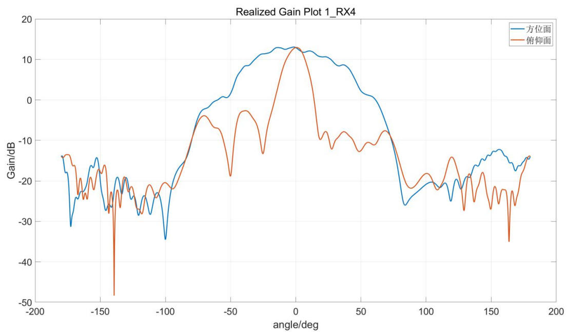
Figure1.4 RX4 directional diagram
