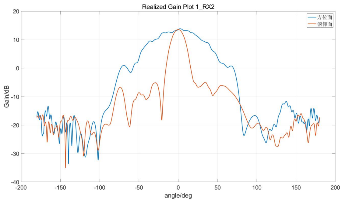
Figure 1.2 RX2directional diagram
