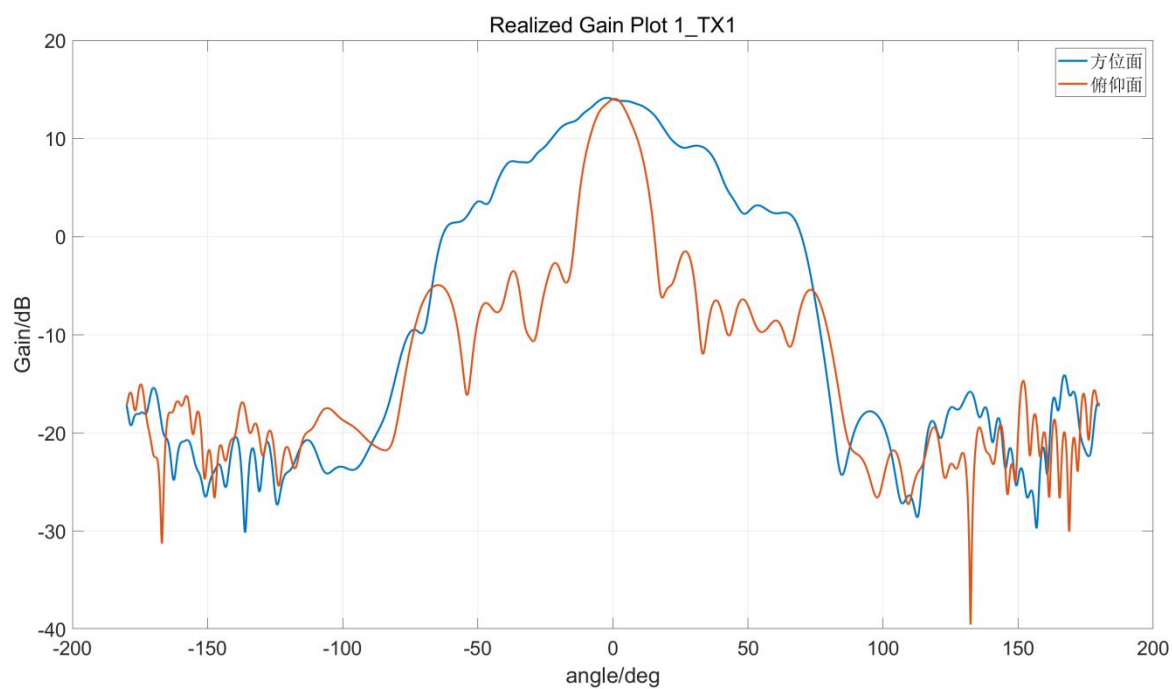
Figure1.5 TX1 directional diagram
