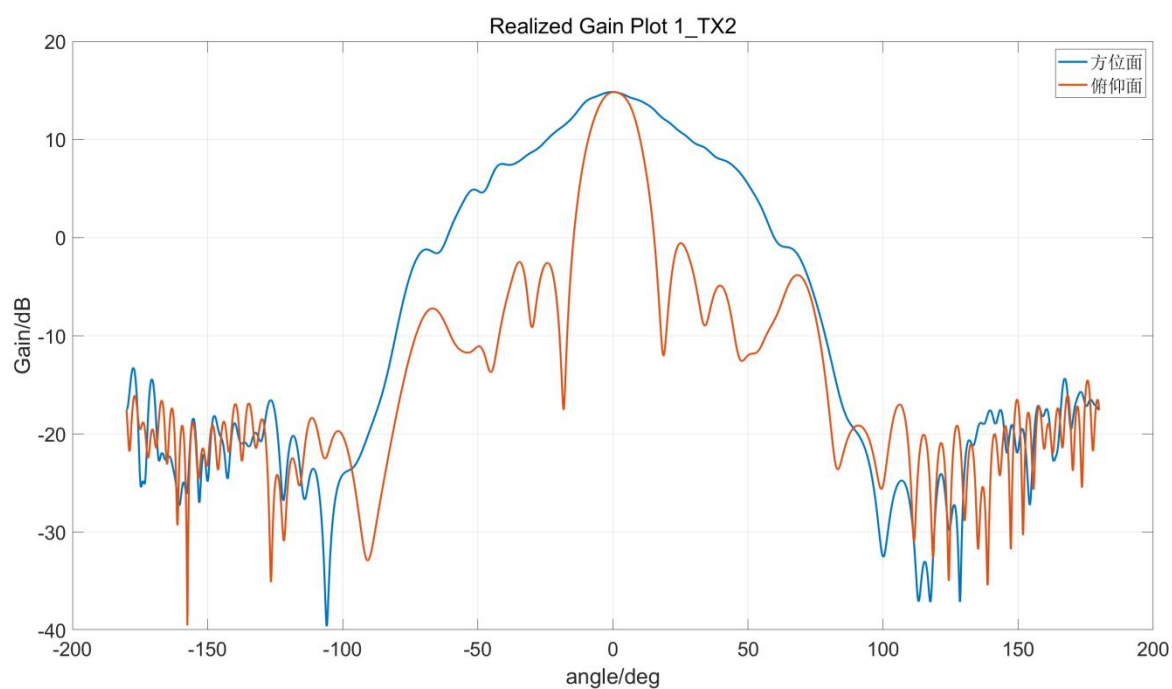
Figure1.6 TX2 directional diagram
