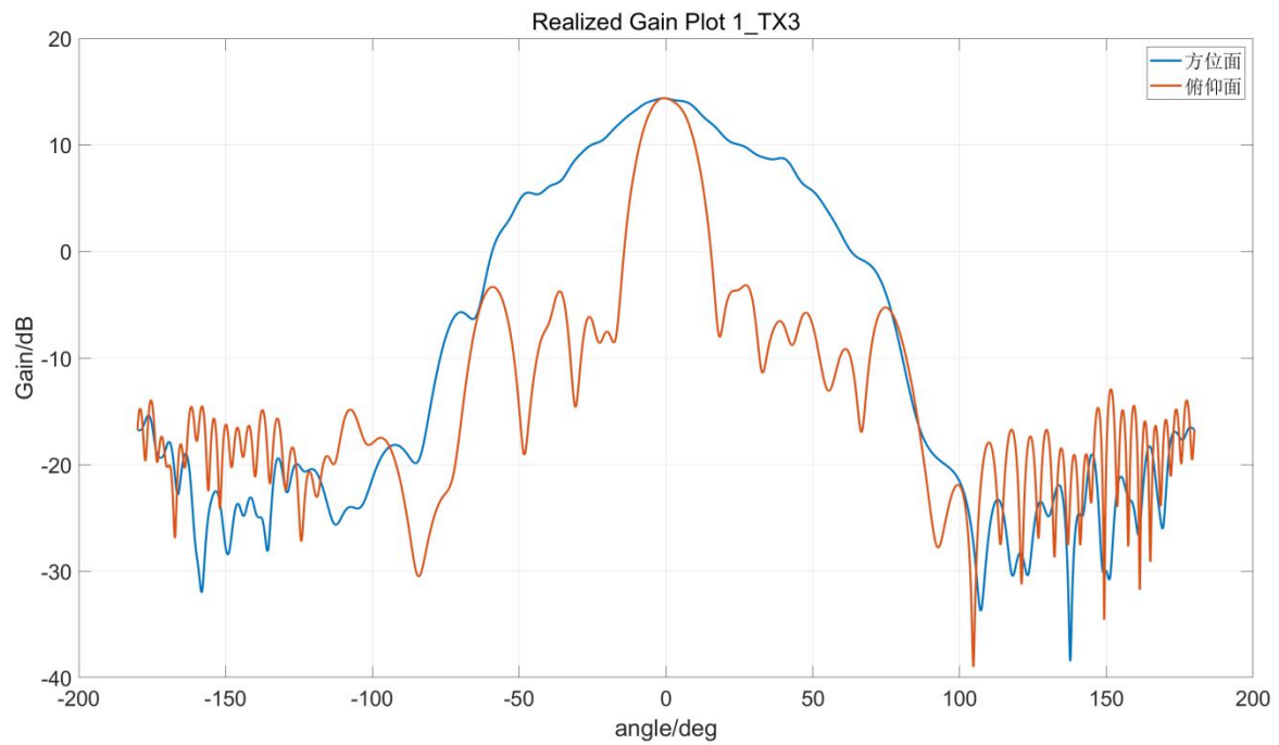
Figure1.7 TX3 directional diagram
