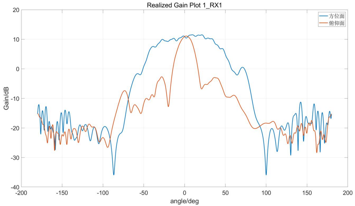
Figure 1.1 RX1 directional diagram
