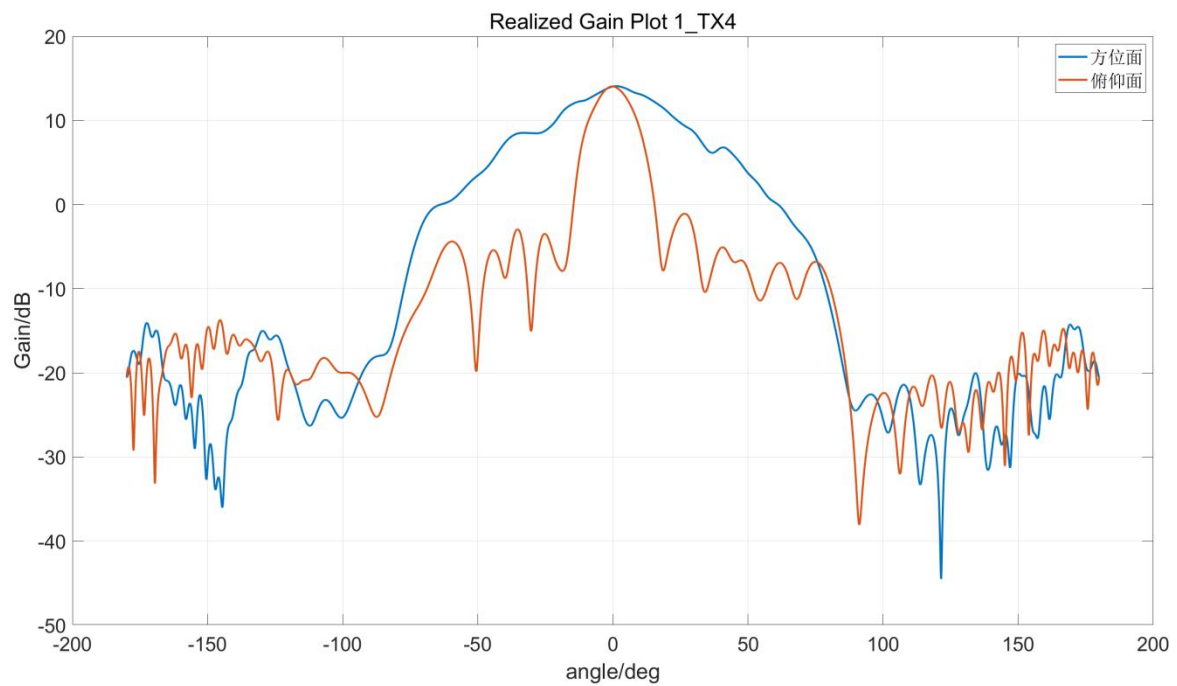
Figure1.8 TX4 directional diagram
