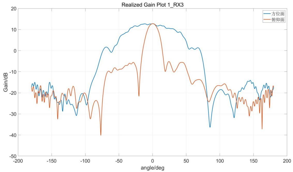
Figure1.3 RX3 directional diagram
