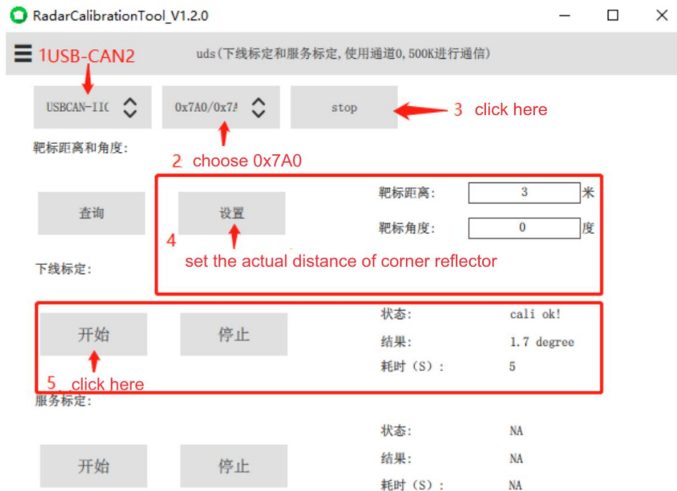
Figure 16. Calibration software operation process
