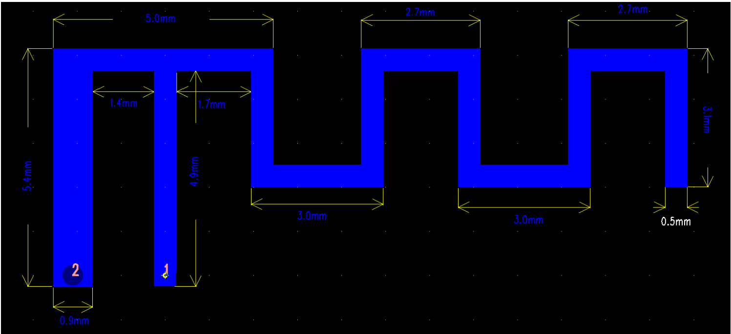
Antenna Photo & Length (mm)
