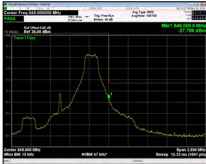
Band5 16QAM BW=1.4MHz Channel=20643 RB Size=6 Position=#0 Extended
