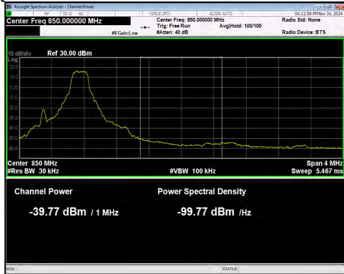
Band5 QPSK BW=1.4MHz Channel=20643 RB Size=1 Position=#Max Normal
