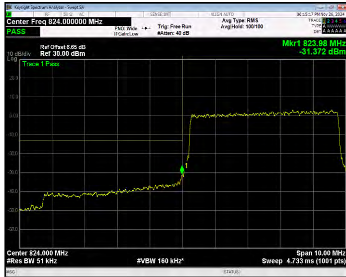
Band5 QPSK BW=5MHz Channel=20425 RB Size=1 Position=#Max Extended
