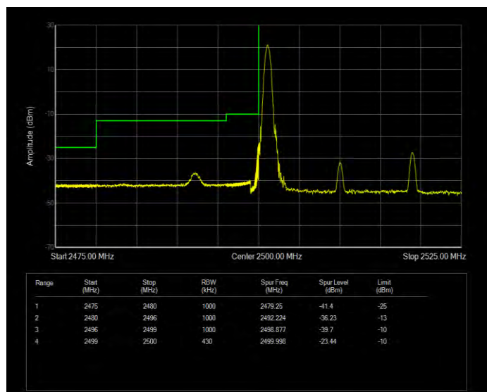
Band7 16QAM BW=20MHz Channel=21350 RB Size=1 Position=#0 Extended
