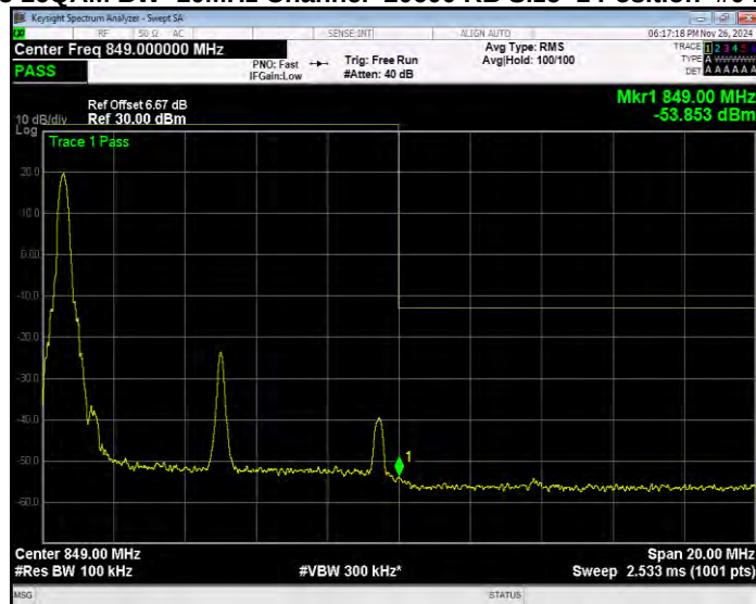
Band5 16QAM BW=10MHz Channel=20600 RB Size=1 Position=#0 Extended
