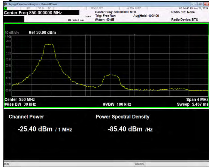
Band5 16QAM BW=3MHz Channel=20635 RB Size=1 Position=#Max Normal
