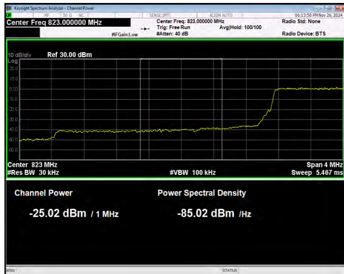
Band5 QPSK BW=3MHz Channel=20635 RB Size=1 Position=#Max Normal
