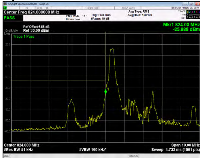
Band5 QPSK BW=5MHz Channel=20425 RB Size=1 Position=#0 Extended
