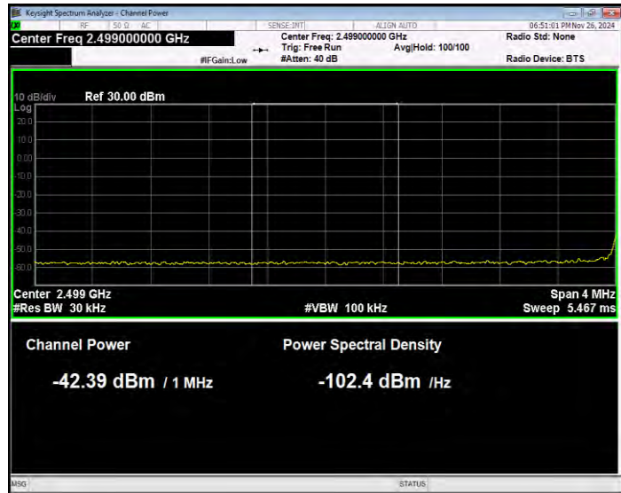
Band7 16QAM BW=20MHz Channel=20850 RB Size=1 Position=#Max Normal
