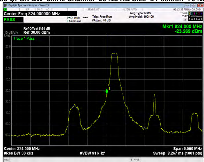
Band5 QPSK BW=3MHz Channel=20415 RB Size=1 Position=#0 Extended
