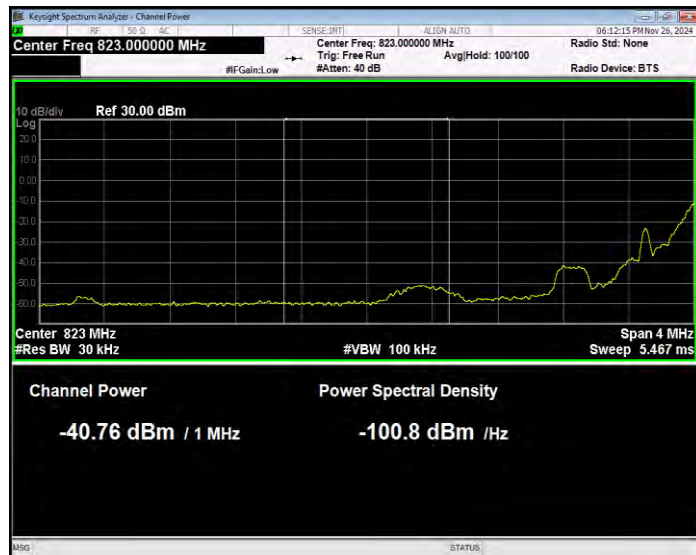
Band5 QPSK BW=1.4MHz Channel=20407 RB Size=1 Position=#Max Normal
