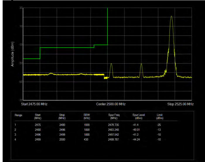
Band7 16QAM BW=20MHz Channel=20850 RB Size=1 Position=#0 Extended
