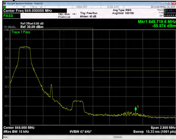
Band5 16QAM BW=1.4MHz Channel=20643 RB Size=1 Position=#Max Extended
