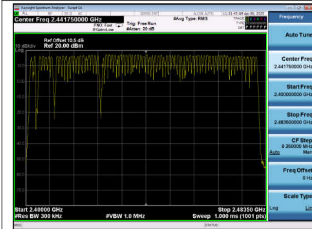
3DH5-Ant7-Hop-PASS
