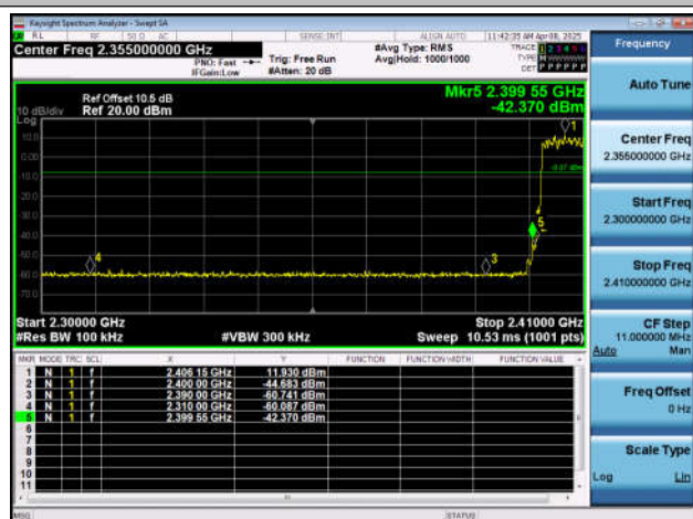
3DH5-Ant7-2402-PASS
