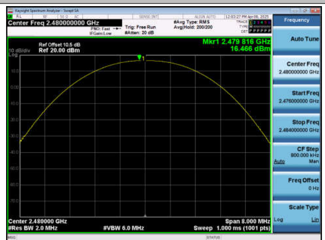
DH5-Ant7-2480-PASS
