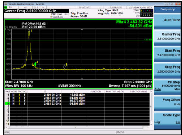
DH5-Ant7-Hop_2480-PASS
