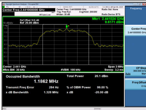
2DH5-Ant7-2441
