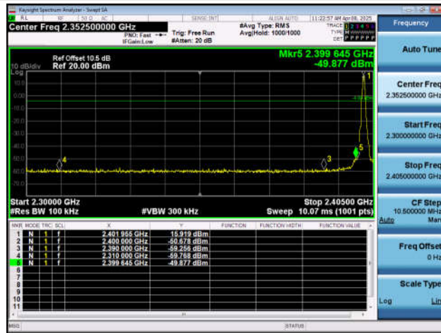
DH5-Ant7-Hop_2402-PASS
