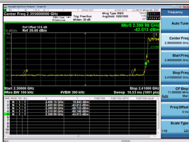
3DH5-Ant7-Hop_2402-PASS
