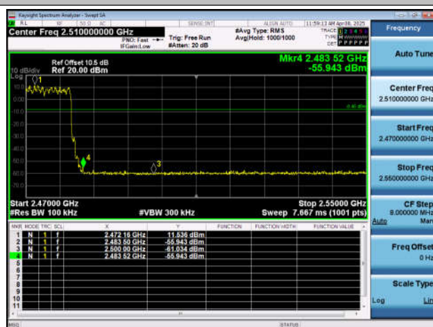
3DH5-Ant7-Hop_2480-PASS
