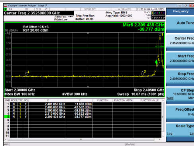
2DH5-Ant7-2402-PASS
