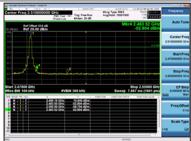
2DH5-Ant7-2480-PASS
