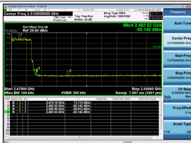
3DH5-Ant7-2480-PASS
