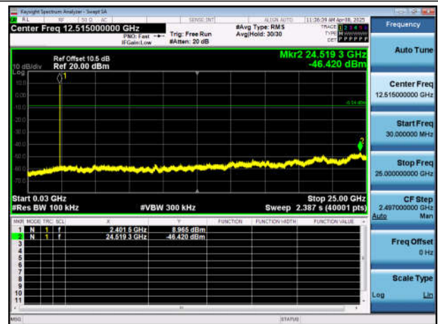
2DH5-Ant7-2441-30~25000-PASS
