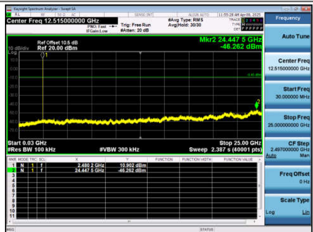
3DH5-Ant7-2480-30~25000-PASS
