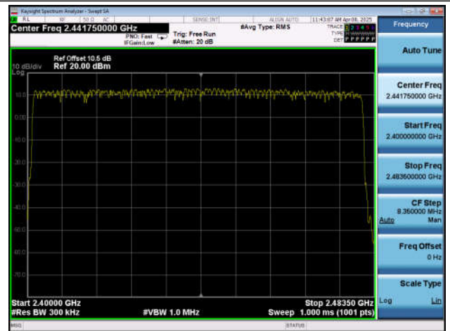
2DH5-Ant7-Hop-PASS
