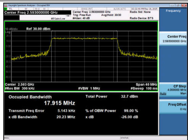
Band41-20MHz-16QAM-40620-100RB#0-PASS
