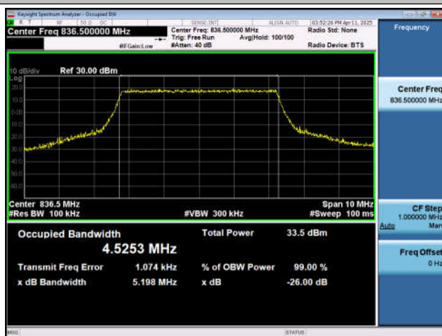
Band26(824-849)-5MHz-QPSK-26915-25RB#0-PASS
