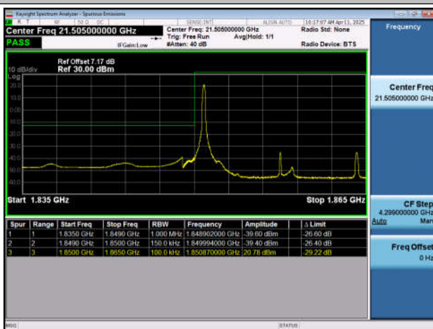
Band2-15MHz-QPSK-18675-1RB#0-PASS
