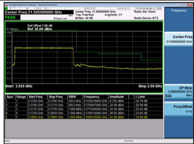
Band7-20MHz-QPSK-20850-100RB#0-PASS
