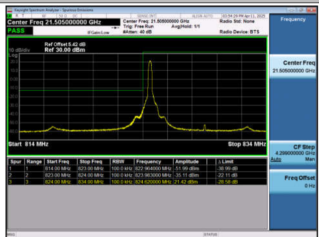
Band26(824-849)-10MHz-QPSK-26840-1RB#0-PASS
