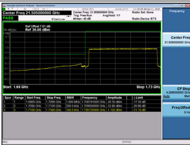
Band66-20MHz-QPSK-132572-100RB#0-PASS
