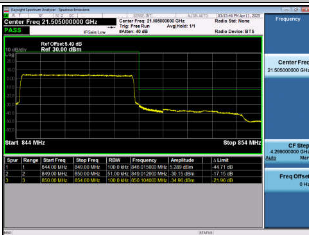
Band26(824-849)-5MHz-QPSK-27015-25RB#0-PASS
