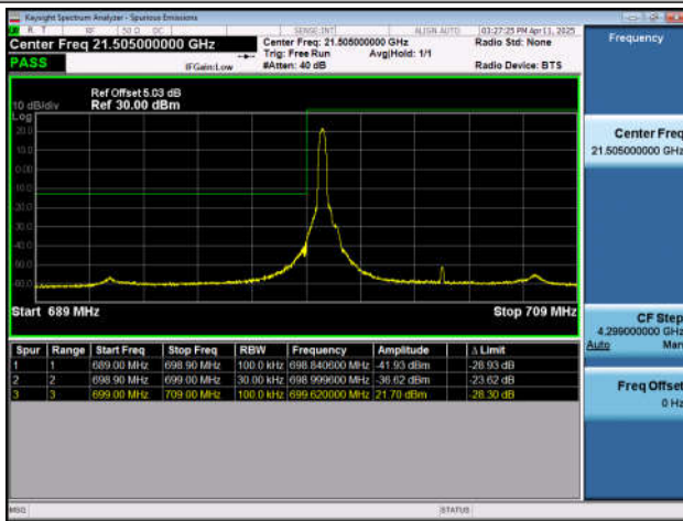
Band12-10MHz-QPSK-23130-1RB#49-PASS
