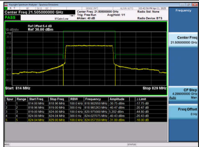
Band26(814-824)-10MHz-QPSK-26740-1RB#49-PASS
