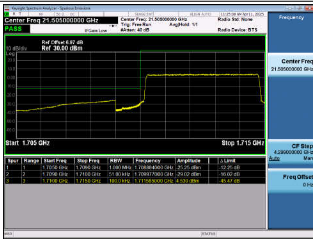
Band66-5MHz-QPSK-132647-25RB#0-PASS
