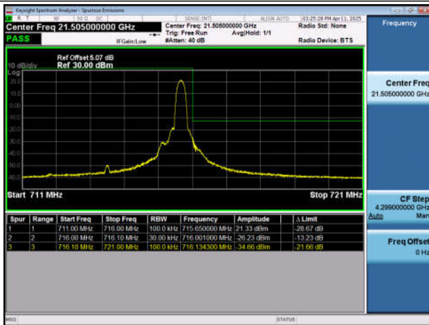
Band12-10MHz-QPSK-23060-1RB#0-PASS
