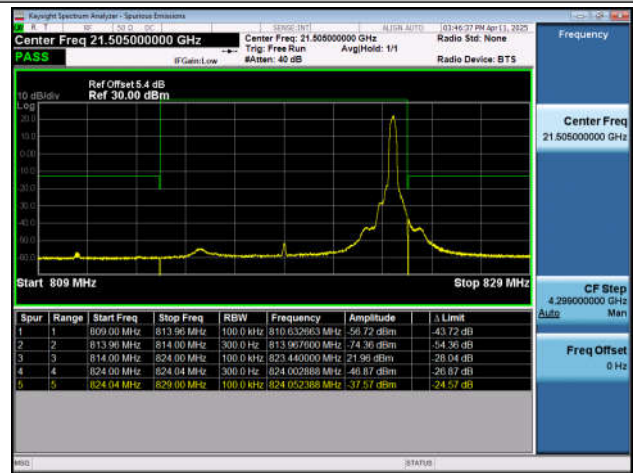
Band26(824-849)-1.4MHz-QPSK-26797-1RB#0-PASS
