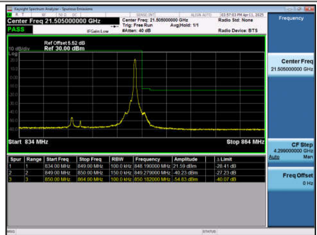
Band26(824-849)-15MHz-QPSK-26965-1RB#74-PASS
