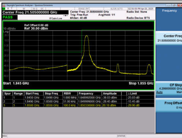
Band25-5MHz-QPSK-26065-1RB#0-PASS
