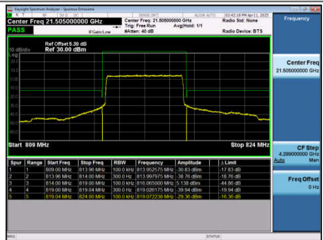
Band26(814-824)-5MHz-QPSK-26715-25RB#0-PASS
