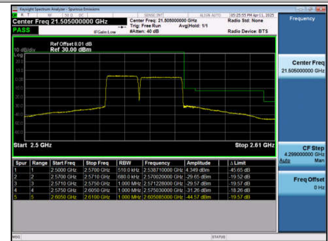
7-7-20MHz-10MHz-QPSK@QPSK-QPSK@QPSK-20850-20 994-100RB#0@100RB#0-50RB#0@50RB#0-PASS
