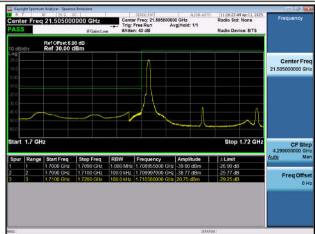
Band66-10MHz-QPSK-132022-1RB#0-PASS
