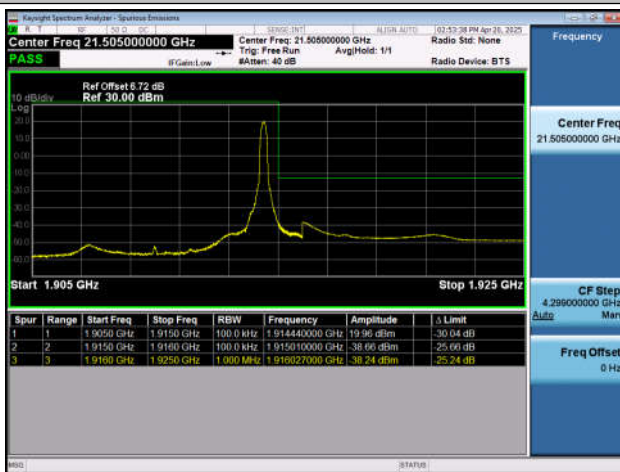
Band25-10MHz-QPSK-26640-1RB#49-PASS
