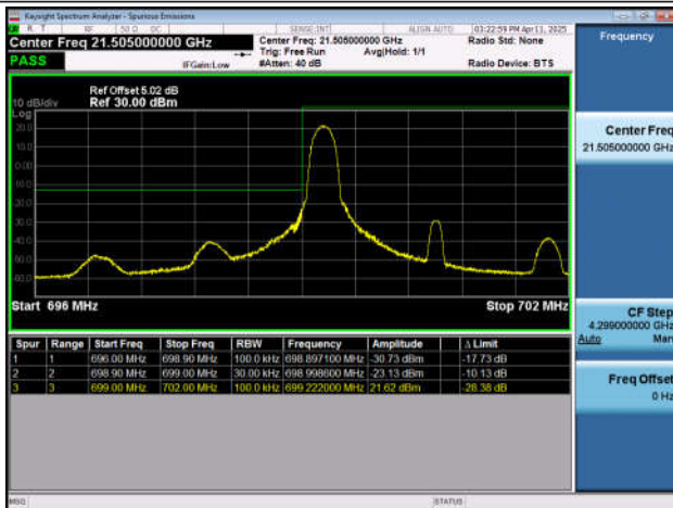
Band12-3MHz-QPSK-23165-1RB#14-PASS
