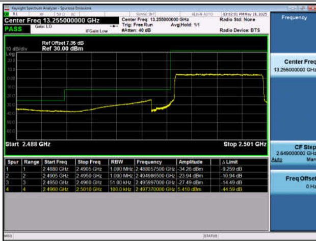
Band41-5MHz-QPSK-41565-25RB#0-PASS
