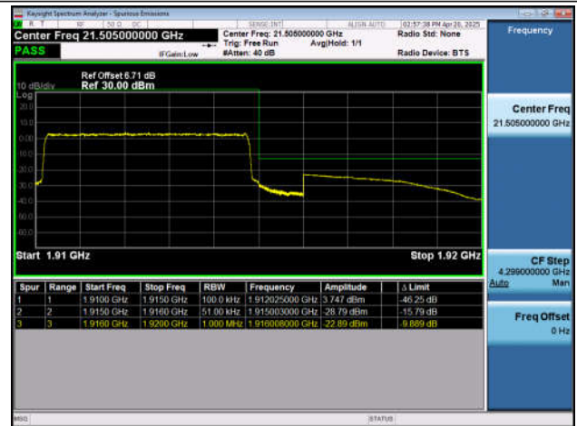
Band25-10MHz-QPSK-26090-50RB#0-PASS
