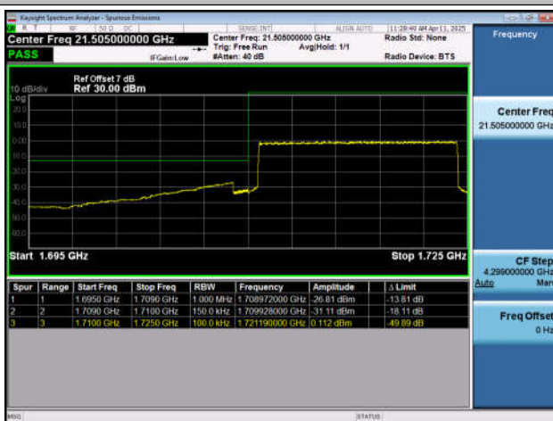
Band66-15MHz-QPSK-132047-75RB#0-PASS
