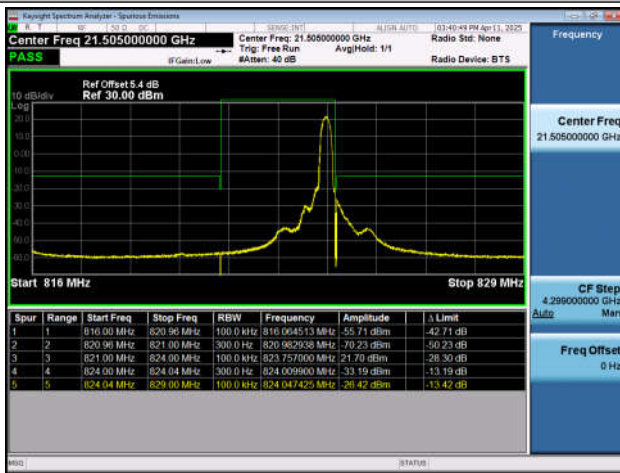
Band26(814-824)-5MHz-QPSK-26715-1RB#0-PASS
