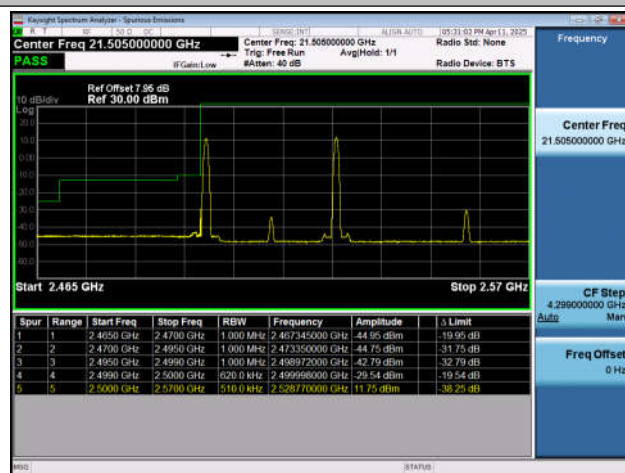
7-7-20MHz-10MHz-QPSK@QPSK-QPSK@QPSK-20850-2 0994-1RB#0@100RB#0-1RB#49@50RB#0-PASS
