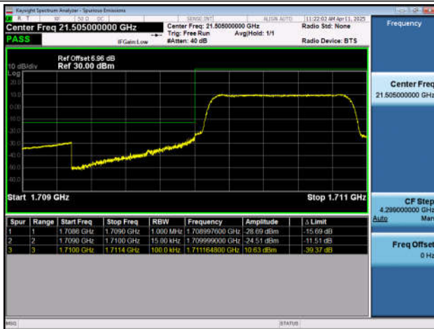
Band66-1.4MHz-QPSK-132665-6RB#0-PASS
