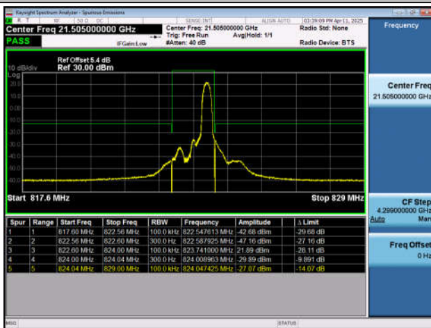
Band26(814-824)-1.4MHz-QPSK-26783-1RB#5-PASS
