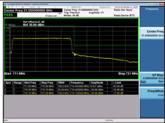
Band17-10MHz-QPSK-23780-50RB#0-PASS
