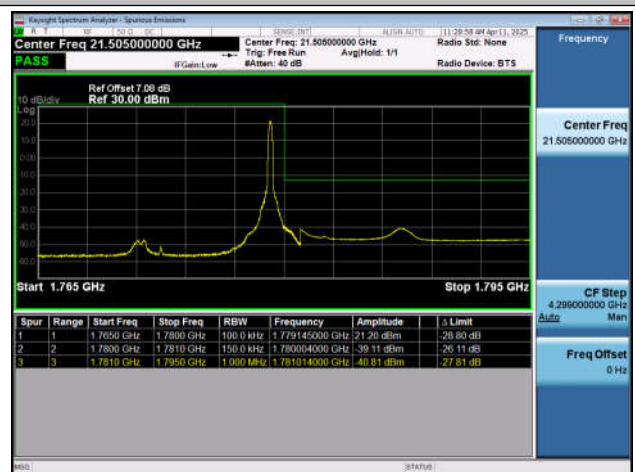
Band66-15MHz-QPSK-132597-1RB#74-PASS
