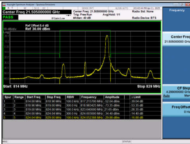
Band26(814-824)-10MHz-QPSK-26740-1RB#0-PASS
