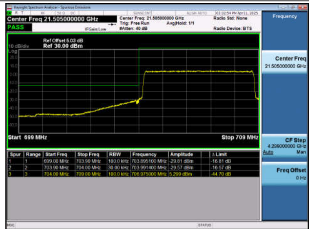
Band17-5MHz-QPSK-23825-25RB#0-PASS
