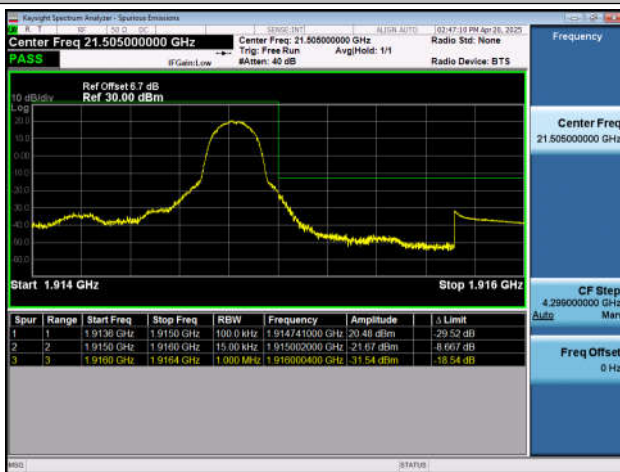
Band25-1.4MHz-QPSK-26683-1RB#5-PASS
