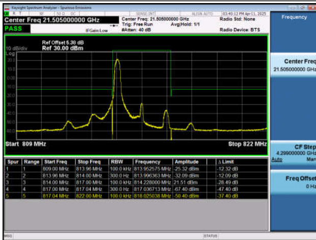
Band26(814-824)-3MHz-QPSK-26775-1RB#14-PASS
