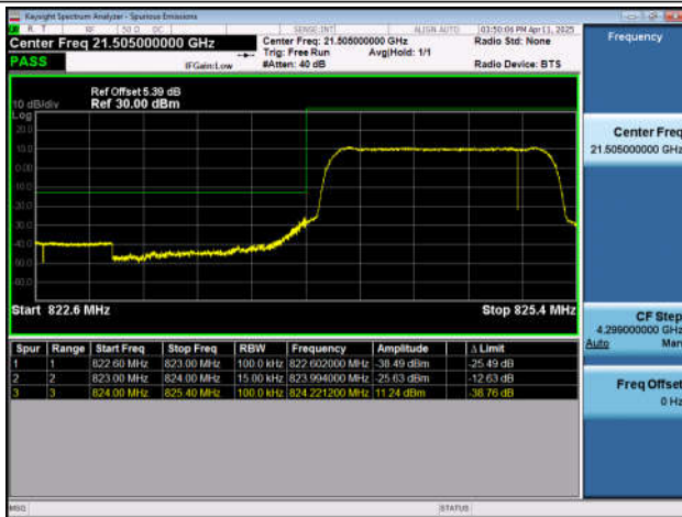
Band26(824-849)-1.4MHz-QPSK-27033-6RB#0-PASS
