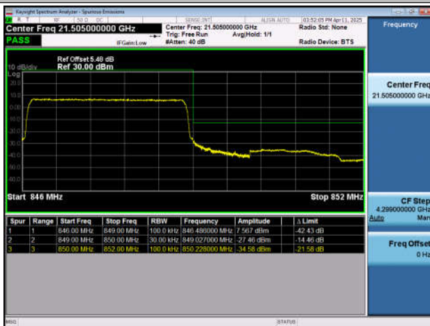
Band26(824-849)-5MHz-QPSK-26815-25RB#0-PASS
