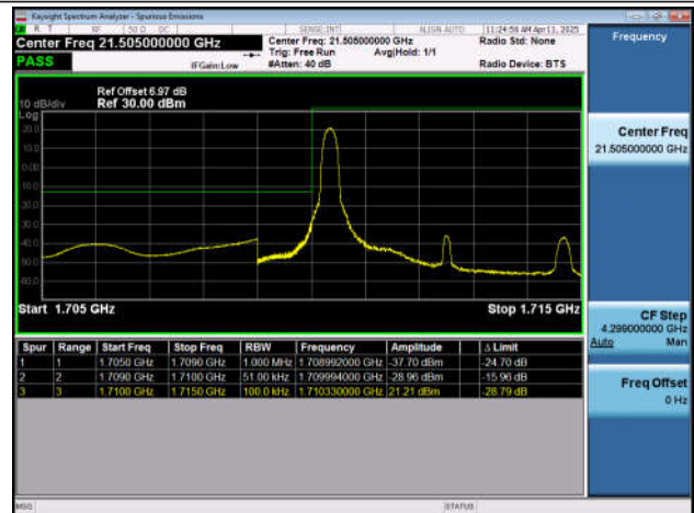
Band66-5MHz-QPSK-132647-1RB#24-PASS
