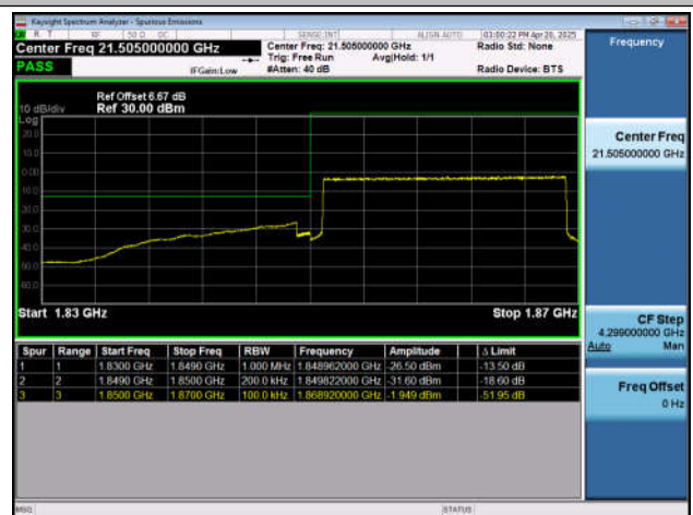
Band25-20MHz-QPSK-26140-100RB#0-PASS
