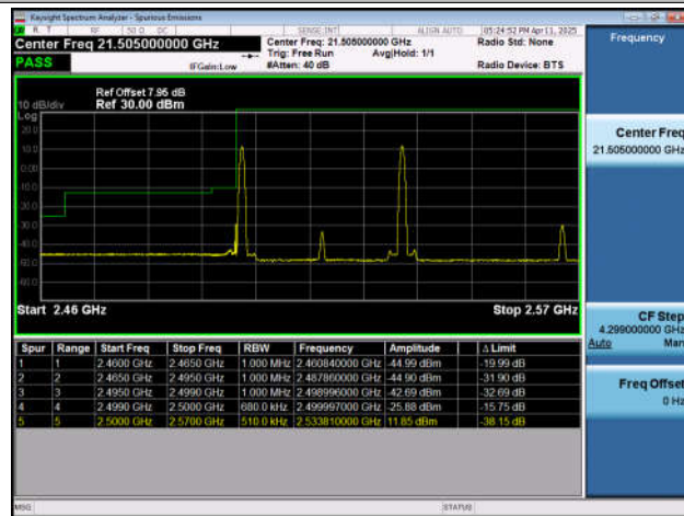
7-7-15MHz-20MHz-QPSK@QPSK-QPSK@QPSK-21179-2 1350-1RB#0@75RB#0-1RB#99@100RB#0-PASS
