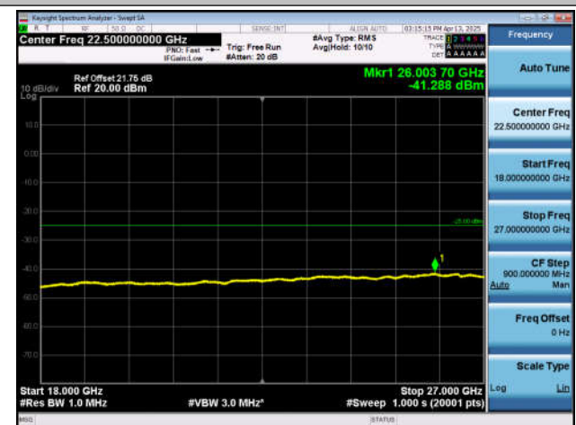
41-41-20MHz-20MHz-QPSK-QPSK-39750-39948-1RB#0-0 RB#0-18000~27000MHz-PASS
