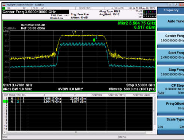
NTNT-n78(3450-3550)-PC2-30-30-M-CP-256QAM-Outer_ Full-Ant1-PASS
