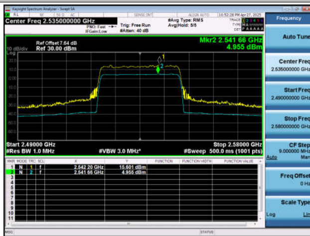
NTNT-n7-PC3-15-40-M-DFT-256QAM-Outer_Full-Ant1-PAS
