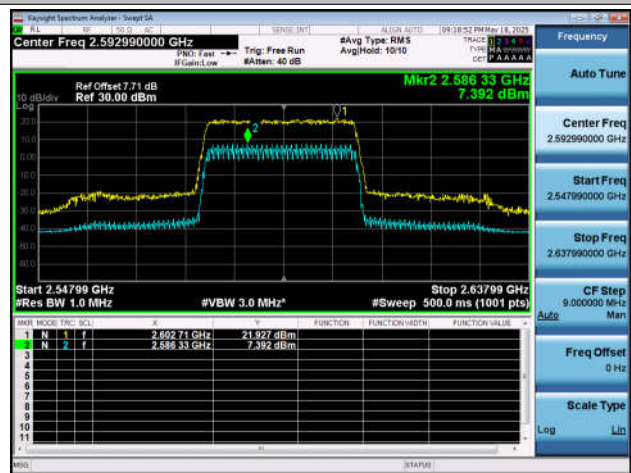
NTNT-n41-PC2-30-40-M-DFT-256QAM-Outer_Full-Ant1-PA
