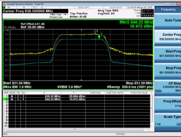
NTNT-n26(824-849)-PC3-15-15-M-CP-256QAM-Outer_Full -Ant1-PASS
