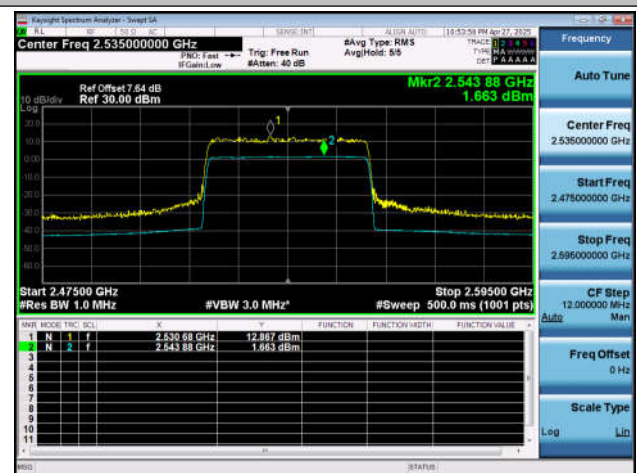
NTNT-n7-PC3-15-40-M-CP-256QAM-Outer_Full-Ant1-PAS
