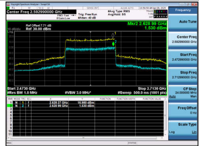
NTNT-n41-PC2-30-90-M-DFT-256QAM-Outer_Full-Ant1-PA
