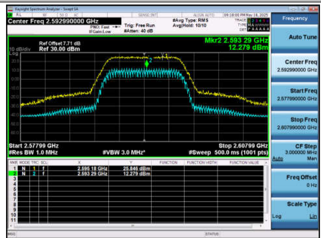
NTNT-n41-PC2-30-10-M-DFT-256QAM-Outer_Full-Ant1-PA SS
