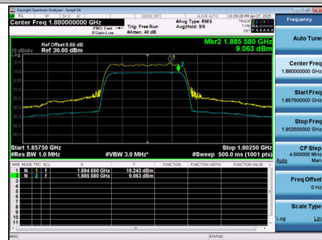
NTNT-n2-PC3-15-15-M-DFT-256QAM-Outer_Full-Ant1-PAS
