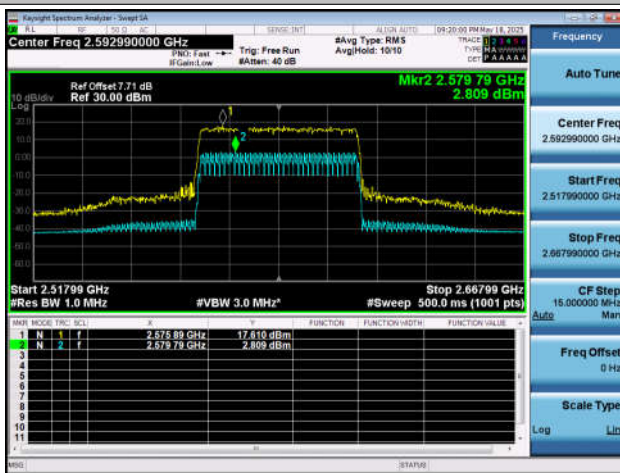
NTNT-n41-PC2-30-60-M-CP-256QAM-Outer_Full-Ant1-PA
