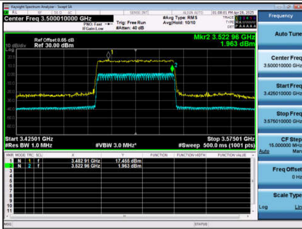
NTNT-n77(3450-3550)-PC2-30-60-M-CP-256QAM-Outer_ Full-Ant1-PASS
