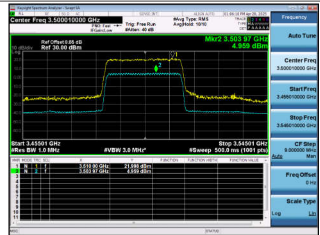
NTNT-n77(3450-3550)-PC2-30-40-M-DFT-256QAM-Out_ Full-Ant1-PASS
