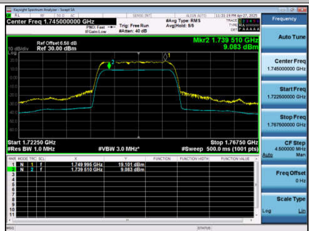
NTNT-n66-PC3-15-15-M-DFT-256QAM-Outer_Full-Ant1-PA
