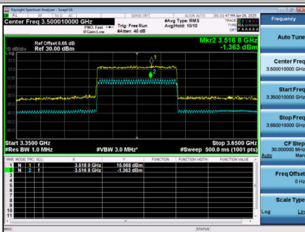
NTNT-n77(3450-3550)-PC2-30-100-M-CP-256QAM-Out_ Full-Ant1-PASS
