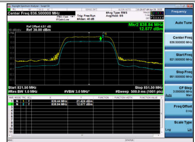
NTNT-n26(824-849)-PC3-15-10-M-DFT-256QAM-Outer_Full-I-Ant1-PASS
