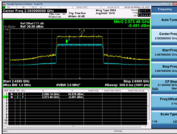
NTNT-n41-PC2-30-80-M-CP-256QAM-Outer_Full-Ant1-PA
