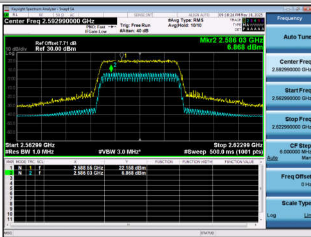
NTNT-n41-PC2-30-30-M-CP-256QAM-Outer_Full-Ant1-PA
