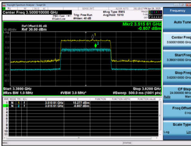
NTNT-n77(3450-3550)-PC2-30-90-M-CP-256QAM-Out_ Full-Ant1-PASS
