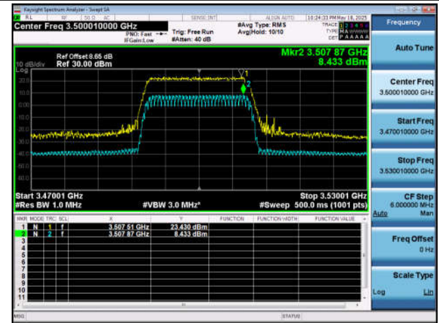
NTNT-n78(3450-3550)-PC2-30-30-M-DFT-256QAM-Outer_ Full-Ant1-PASS
