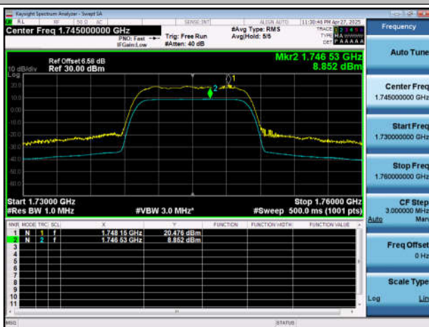
NTNT-n66-PC3-15-10-M-CP-256QAM-Outer_Full-Ant1-PA
