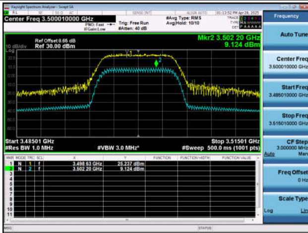
NTNT-n78(3450-3550)-PC2-30-20-M-CP-256QAM-Outer_ Full-Ant1-PASS
