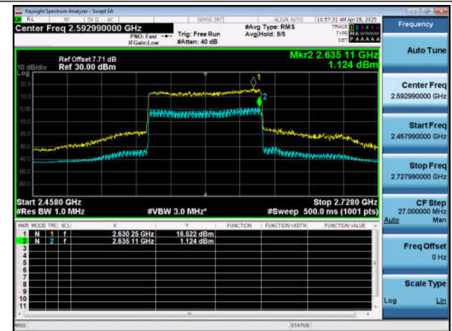
NTNT-n41-PC2-30-100-M-DFT-256QAM-Outer_Full-Ant1-PA
