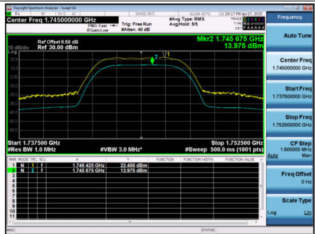
NTNT-n66-PC3-15-10-M-DFT-256QAM-Outer_Full-Ant1-PA
