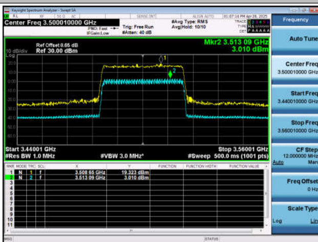
NTNT-n77(3450-3550)-PC2-30-40-M-CP-256QAM-Out_ Full-Ant1-PASS
