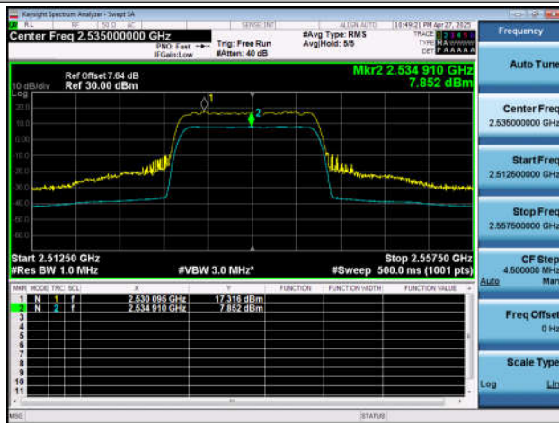
NTNT-n7-PC3-15-20-M-DFT-256QAM-Outer_Full-Ant1-PAS
