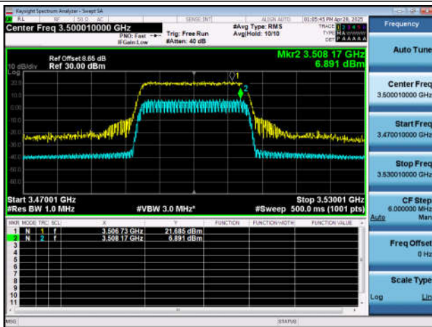
NTNT-n77(3450-3550)-PC2-30-30-M-CP-256QAM-Out_ Full-Ant1-PASS
