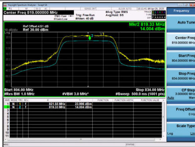
NTNT-n26(814-824)-PC3-15-10-M-CP-256QAM-Outer_Full-Ant1-PASS
