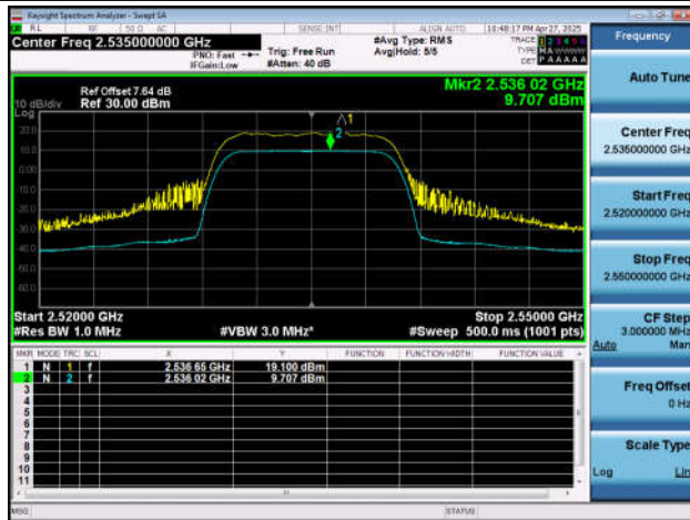
NTNT-n7-PC3-15-15-M-DFT-256QAM-Outer_Full-Ant1-PAS
