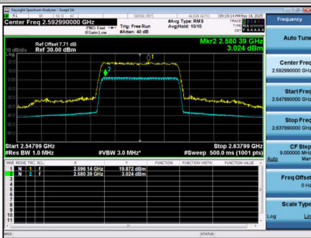
NTNT-n41-PC2-30-30-M-CP-256QAM-Outer_Full-Ant1-PA
