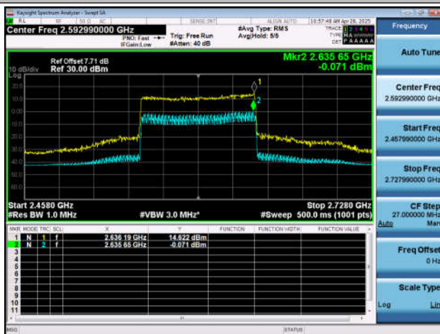
NTNT-n41-PC2-30-90-M-CP-256QAM-Outer_Full-Ant1-PA
