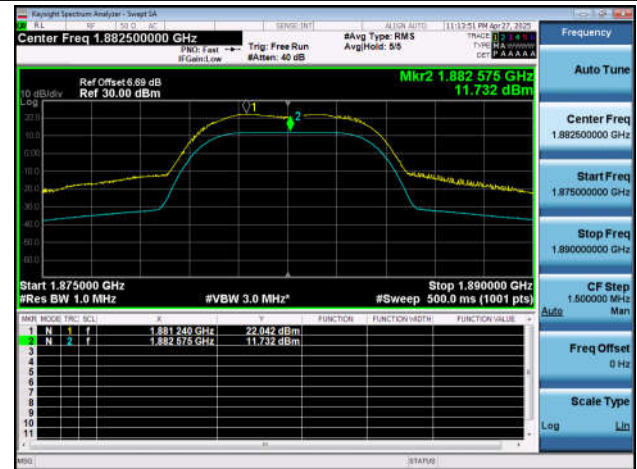
NTNT-n25-PC3-15-10-M-CP-256QAM-Outer_Full-Ant1-PAS
