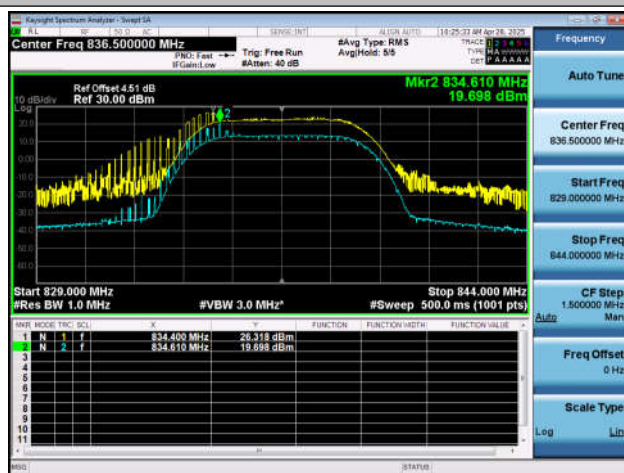
NTNT-n26(824-849)-PC3-15-5-M-CP-256QAM-Outer_Full-Ant1-PASS
