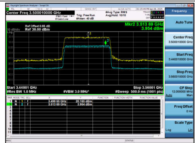
NTNT-n78(3450-3550)-PC2-30-40-M-DFT-256QAM-Outer_ Full-Ant1-PASS
