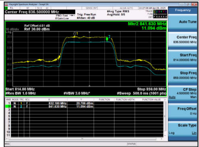
NTNT-n26(824-849)-PC3-15-20-M-DFT-256QAM-Outer_Ful I-Ant1-PASS
