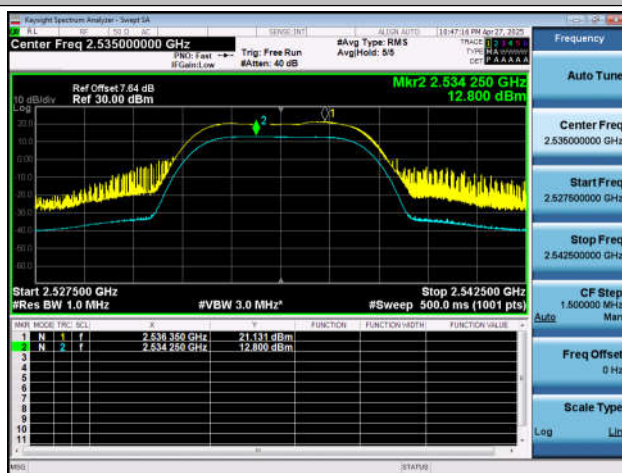
NTNT-n7-PC3-15-5-M-DFT-256QAM-Outer_Full-Ant1-PASS
