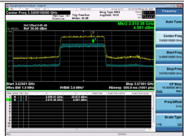
NTNT-n77(3450-3550)-PC2-30-50-M-DFT-256QAM-Out_ Full-Ant1-PASS
