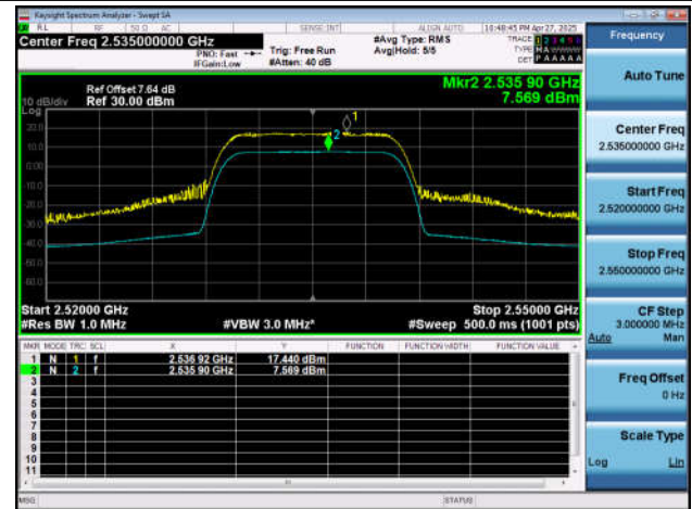
NTNT-n7-PC3-15-15-M-CP-256QAM-Outer_Full-Ant1-PAS
