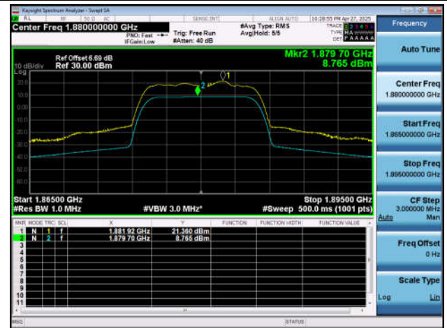
NTNT-n2-PC3-15-15-M-CP-256QAM-Outer_Full-Ant1-PAS
