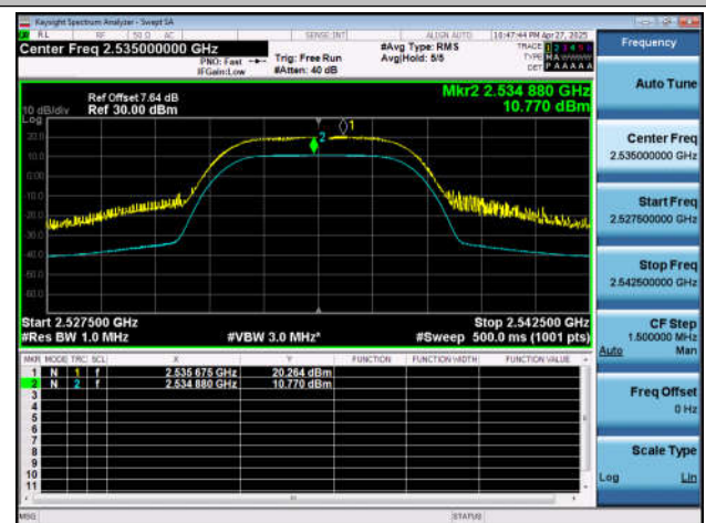
NTNT-n7-PC3-15-5-M-CP-256QAM-Outer_Full-Ant1-PASS
