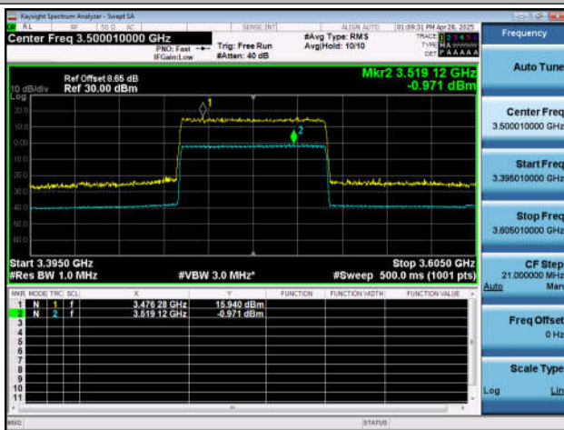
NTNT-n77(3450-3550)-PC2-30-70-M-CP-256QAM-Outer_ Full-Ant1-PASS
