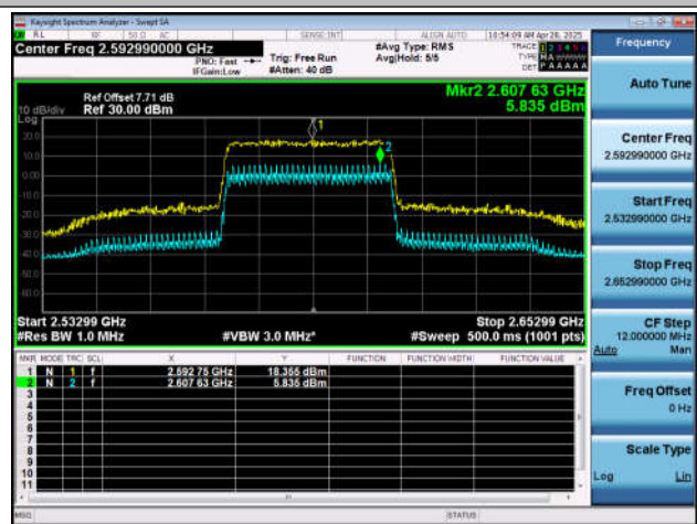
NTNT-n41-PC2-30-40-M-DFT-256QAM-Outer_Full-Ant1-PA
