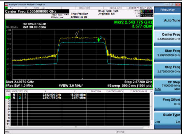
NTNT-n7-PC3-15-30-M-CP-256QAM-Outer_Full-Ant1-PAS
