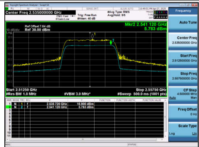
NTNT-n7-PC3-15-20-M-CP-256QAM-Outer_Full-Ant1-PAS
