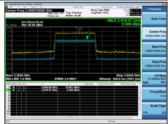
NTNT-n77(3450-3550)-PC2-30-80-M-DFT-256QAM-Outer_ Full-Ant1-PASS
