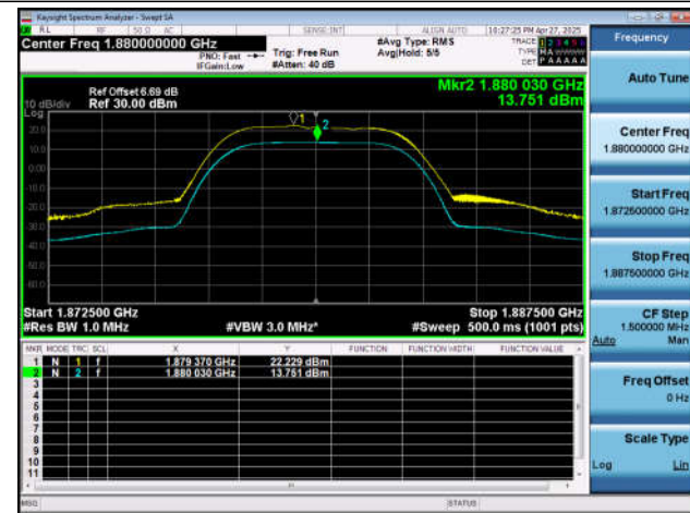
NTNT-n2-PC3-15-10-M-DFT-256QAM-Outer_Full-Ant1-PAS
