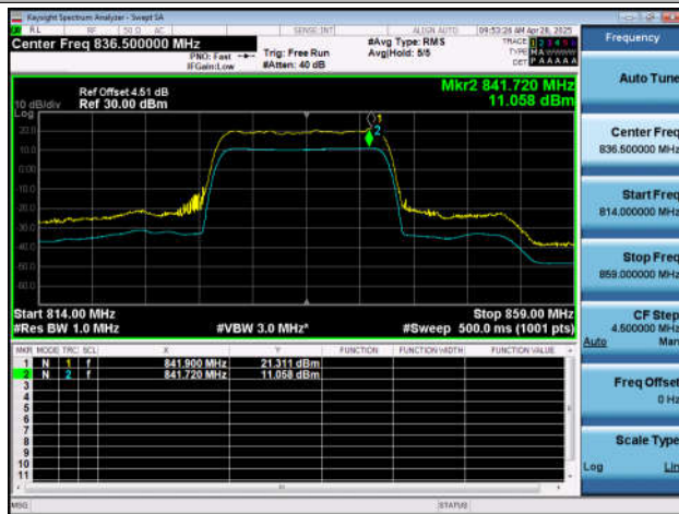
NTNT-n5-PC3-15-20-M-DFT-256QAM-Outer_Full-Ant1-PAS
