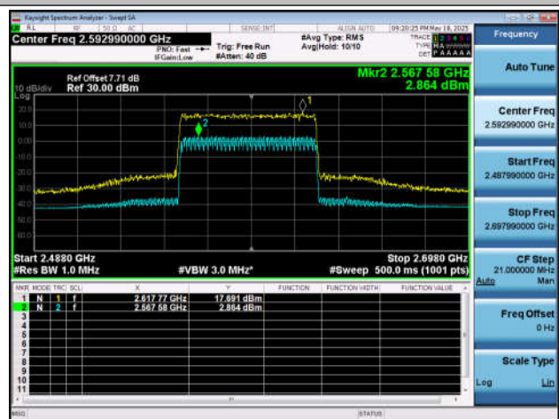
NTNT-n41-PC2-30-70-M-DFT-256QAM-Outer_Full-Ant1-PA
