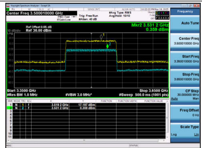
NTNT-n78(3450-3550)-PC2-30-10-M-DFT-256QAM-Out_ Full-Ant1-PASS
