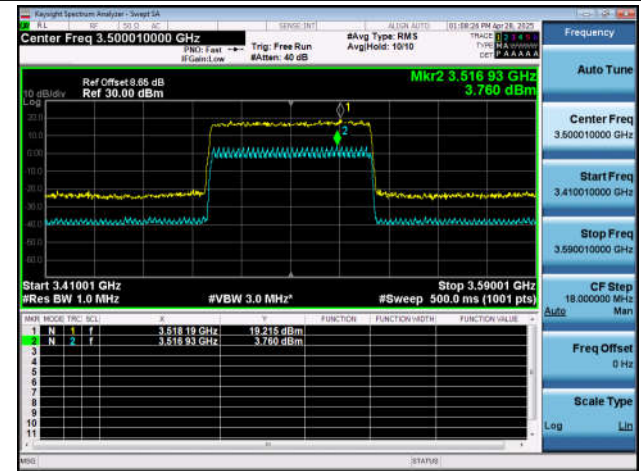
NTNT-n77(3450-3550)-PC2-30-70-M-DFT-256QAM-Outer_ Full-Ant1-PASS
