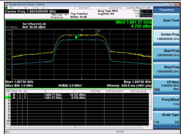
NTNT-n25-PC3-15-15-M-CP-256QAM-Outer_Full-Ant1-PAS
