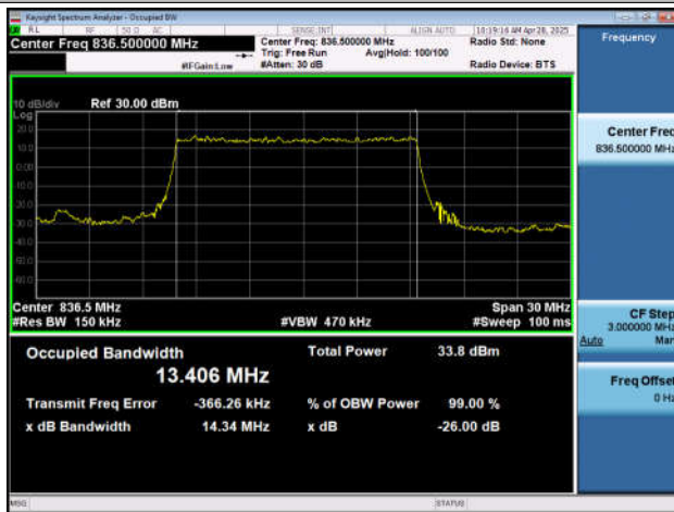
NTNV-n26(824-849)-PC3-15-15-M-DFT-16QAM-Outer_Full -Ant1-PASS
