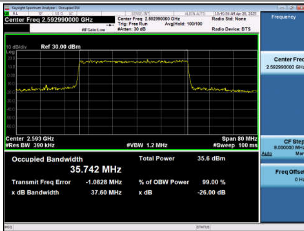
NTNV-n41-PC2-30-40-M-DFT-QPSK-Outer_Full-Ant1-PASS S
