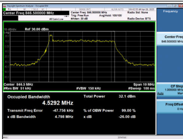
NTNV-n5-PC3-15-5-H-DFT-QPSK-Outer_Full-Ant1-PASS
