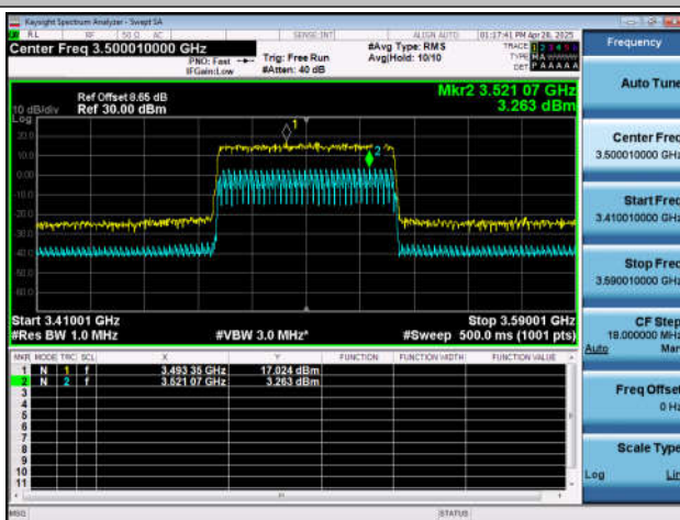
NTNT-n78(3450-3550)-PC2-30-60-M-CP-256QAM-Out_ Full-Ant1-PASS
