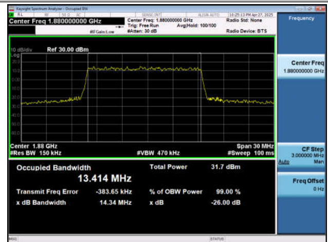
NTNV-n2-PC3-15-15-M-DFT-QPSK-Outter_Full-Ant1-PASS
