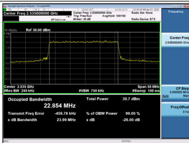
NTNV-n7-PC3-15-25-M-DFT-QPSK-Outter_Full-Ant1-PASS
