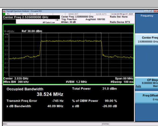
NTNV-n7-PC3-15-40-M-DFT-QPSK-Outer_Full-Ant1-PASS
