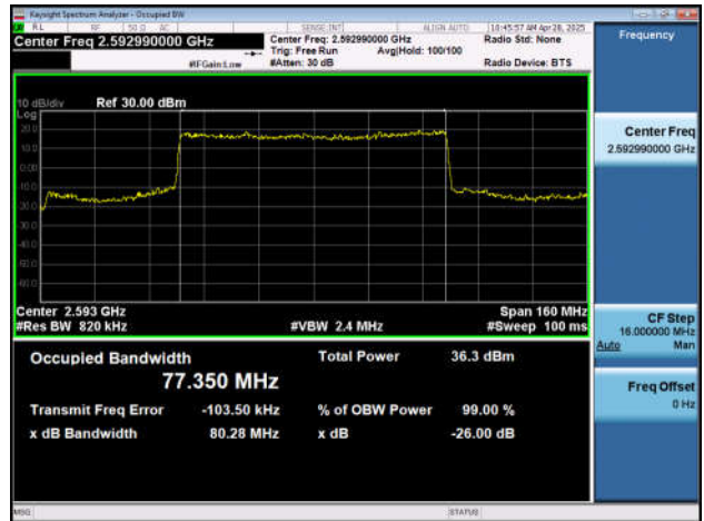
NTNV-n41-PC2-30-80-M-DFT-16QAM-Outer_Full-Ant1-PASS SS
