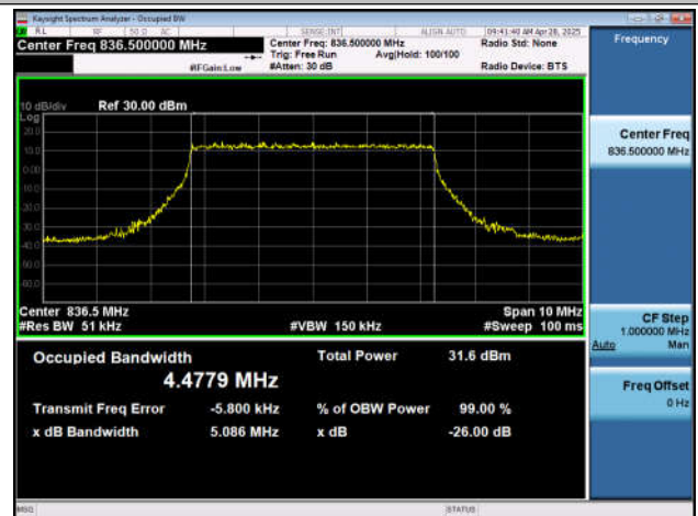
NTNV-n5-PC3-15-5-H-DFT-BPSK-Outer_Full-Ant1-PASS
