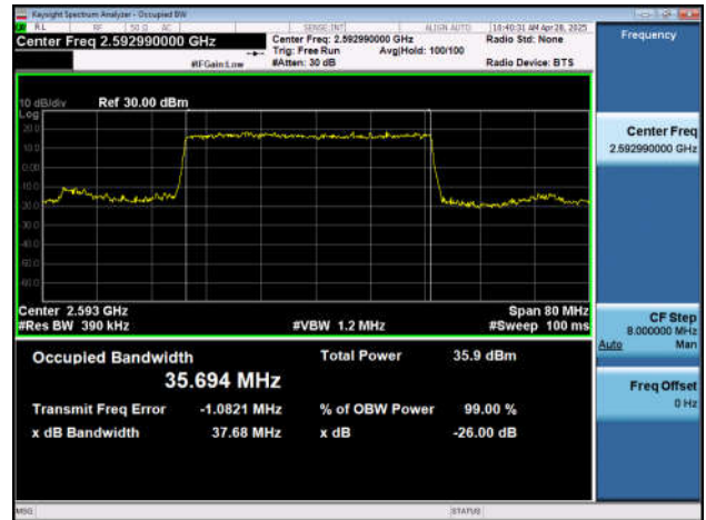
NTNV-n41-PC2-30-40-M-DFT-16QAM-Outer_Full-Ant1-PASS SS
