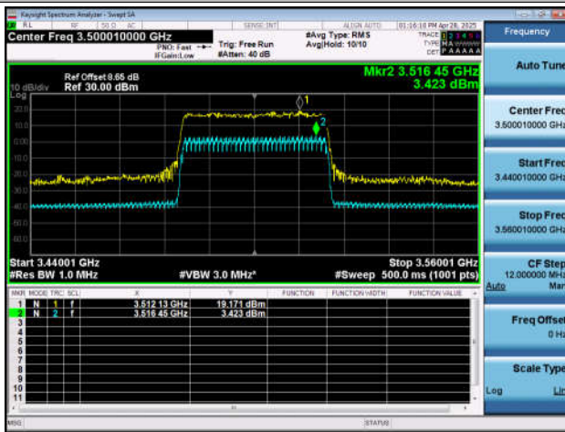
NTNT-n78(3450-3550)-PC2-30-50-M-CP-256QAM-Out_ Full-Ant1-PASS
