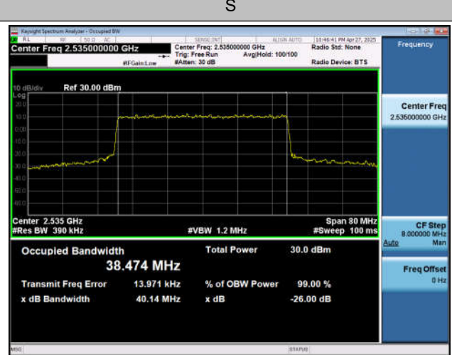
NTNV-n7-PC3-15-40-M-DFT-16QAM-Outer_Full-Ant1-PASS
