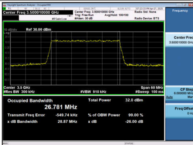
NTNV-n77(3450-3550)-PC2-30-40-M-DFT-QPSK-Outet_Ful
