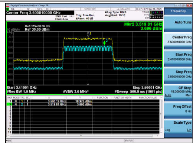
NTNT-n78(3450-3550)-PC2-30-70-M-DFT-256QAM-Out_ Full-Ant1-PASS
