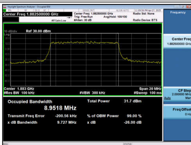
NTNV-n25-PC3-15-10-M-DFT-QPSK-Outet_Full-Ant1-PAS
