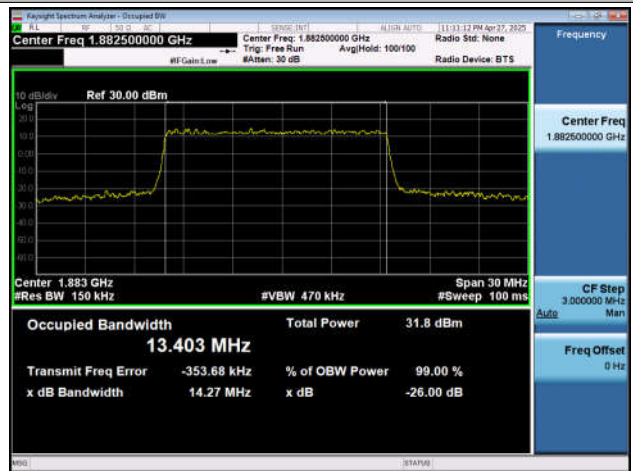
NTNV-n25-PC3-15-15-M-DFT-QPSK-Outer_Full-Ant1-PASS S
