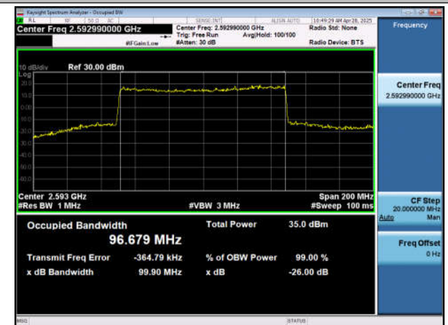
NTNV-n41-PC2-30-100-M-DFT-16QAM-Outer_Full-Ant1-PA
