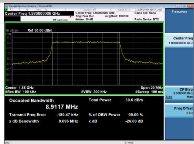
NTNV-n2-PC3-15-10-M-DFT-16QAM-Outer_Full-Ant1-PASS
