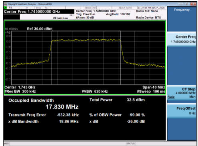
NTNV-n66-PC3-15-20-M-DFT-16QAM-Outer_Full-Ant1-PASS SS
