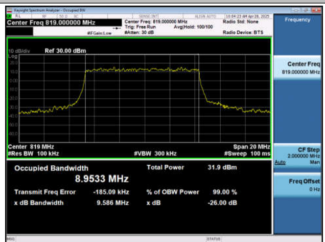
NTNV-n26(814-824)-PC3-15-10-M-DFT-16QAM-Outet_Full-A Ant1-PASS
