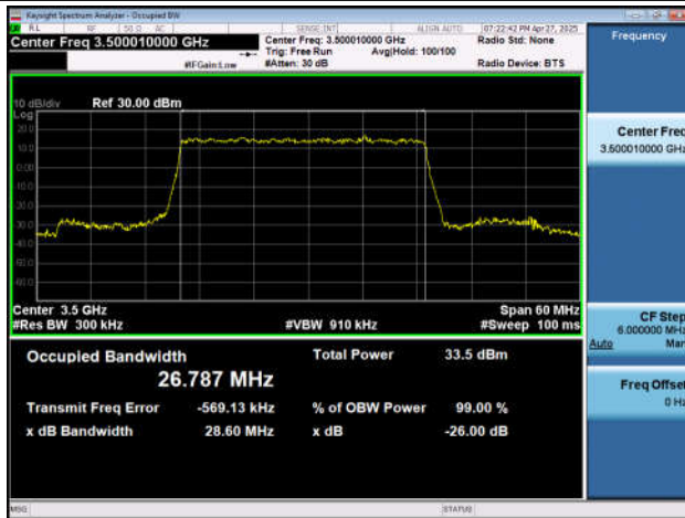
NTNV-n77(3450-3550)-PC2-30-30-M-DFT-16QAM-Outet_F
