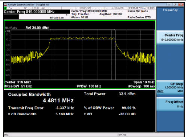
NTNV-n26(814-824)-PC3-15-10-M-DFT-BPSK-Outet_Full-A nt1-PASS
