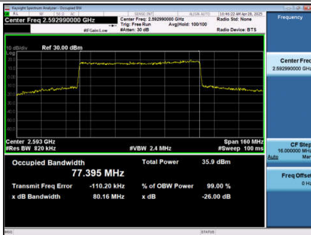
NTNV-n41-PC2-30-80-M-DFT-QPSK-Outer_Full-Ant1-PASS S
