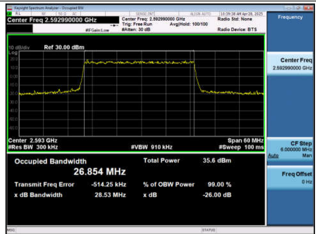
NTNV-n41-PC2-30-30-M-DFT-QPSK-Outer_Full-Ant1-PASS S
