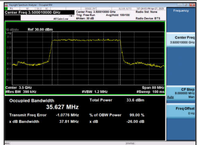
NTNV-n77(3450-3550)-PC2-30-40-M-DFT-16QAM-Outet_F
