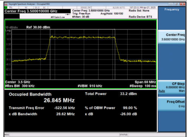
NTNV-n77(3450-3550)-PC2-30-40-M-DFT-BPSK-Outet_Ful
