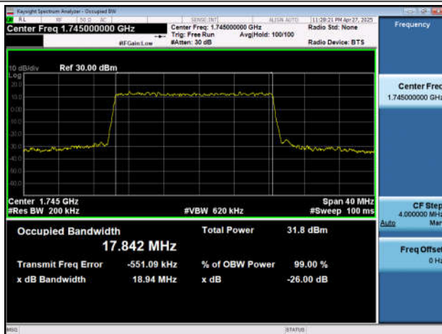
NTNV-n66-PC3-15-20-M-DFT-QPSK-Outer_Full-Ant1-PASS S
