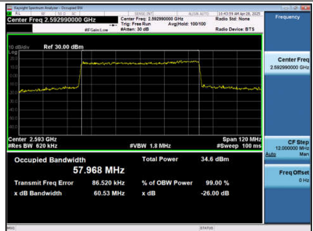
NTNV-n41-PC2-30-60-M-DFT-16QAM-Outer_Full-Ant1-PASS SS
