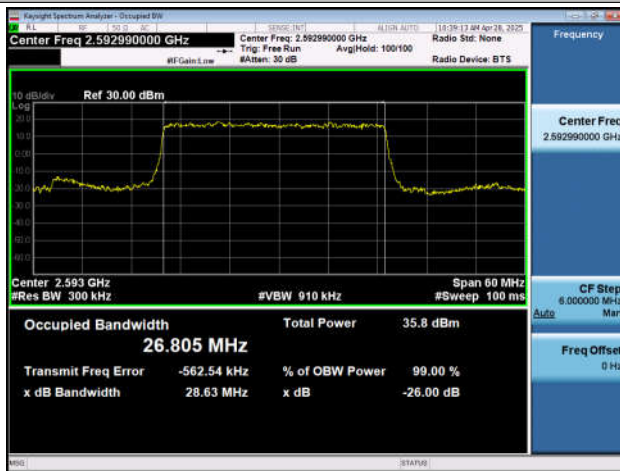
NTNV-n41-PC2-30-30-M-DFT-16QAM-Outer_Full-Ant1-PASS SS
