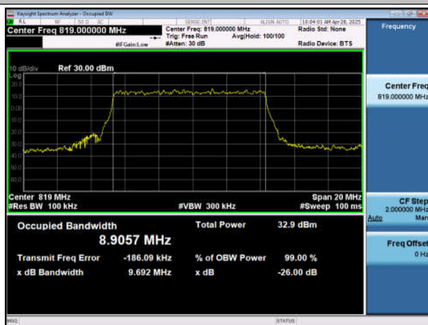
NTNV-n26(814-824)-PC3-15-10-M-DFT-QPSK-Outet_Full-A Ant1-PASS
