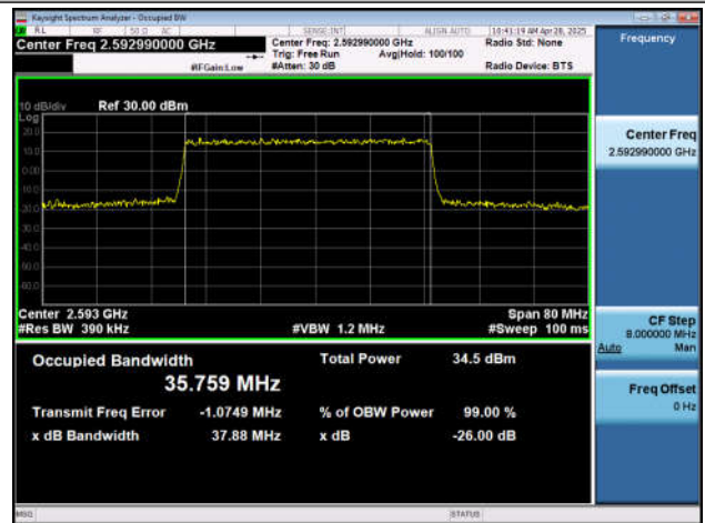
NTNV-n41-PC2-30-40-M-DFT-16QAM-Outer_Full-Ant1-PASS SS
