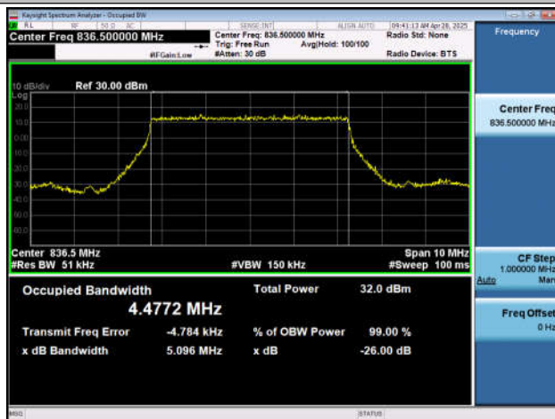
NTNV-n5-PC3-15-5-M-DFT-16QAM-Outer_Full-Ant1-PASS
