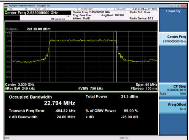
NTNV-n7-PC3-15-25-M-DFT-16QAM-Outter_Full-Ant1-PASS
