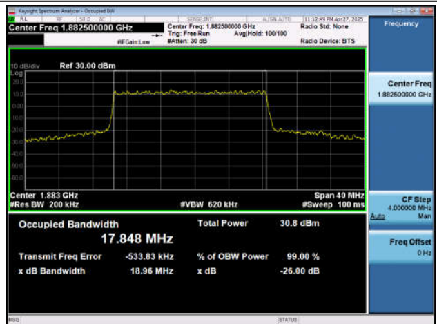
NTNV-n25-PC3-15-20-M-DFT-16QAM-Outer_Full-Ant1-PASS SS
