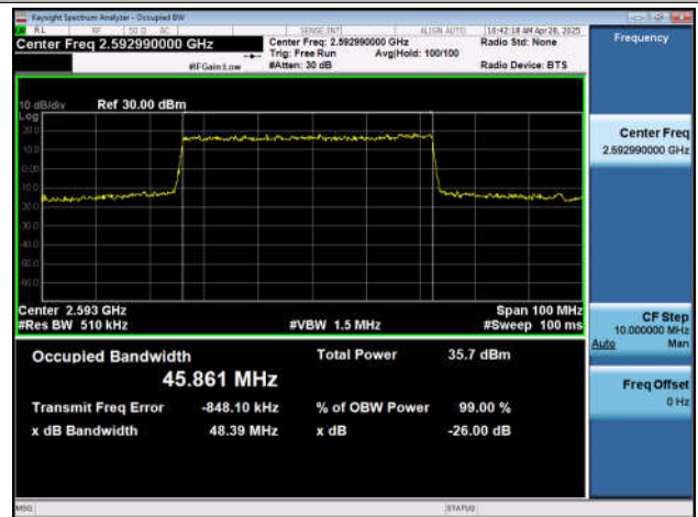
NTNV-n41-PC2-30-50-M-DFT-QPSK-Outer_Full-Ant1-PASS S
