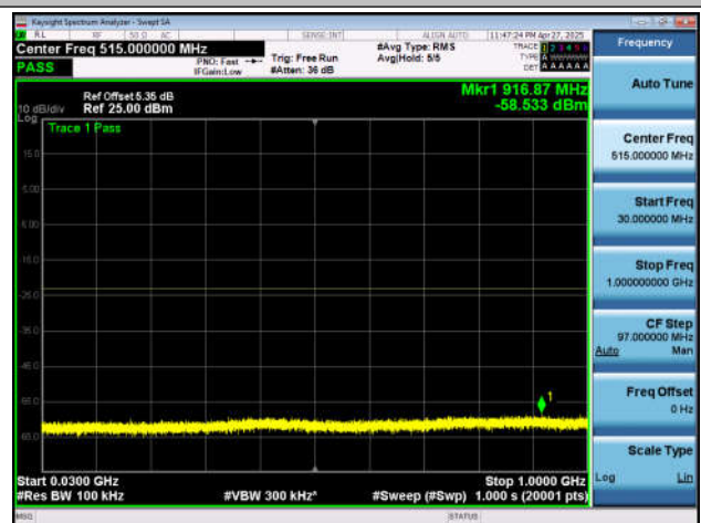
NTNV-n25-PC3-15-20-L-DFT-BPSK-Inner_1RB_Left-30-10
