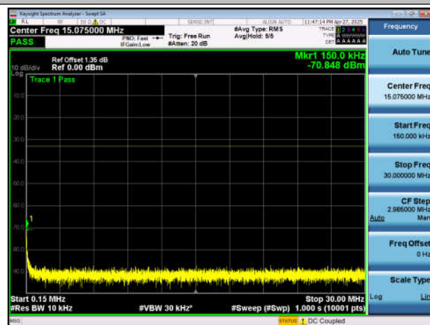
NTNV-n25-PC3-15-20-L-DFT-BPSK-Inner_1RB_Left-0.15-3
