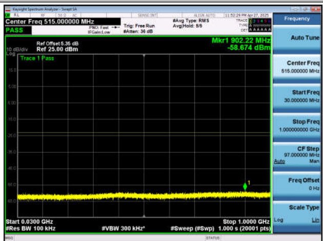
NTNV-n66-PC3-15-20-L-DFT-BPSK-Inner_1RB_Left-30-10 00-PASS
