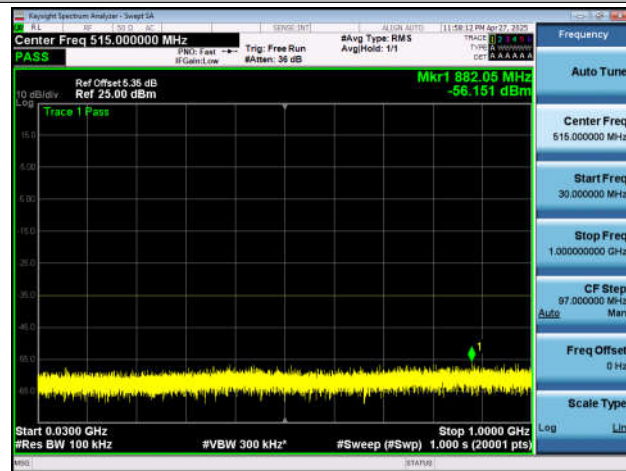
NTNV-n7-PC3-15-40-H-DFT-BPSK-Inner_1RB_Left-12000-
