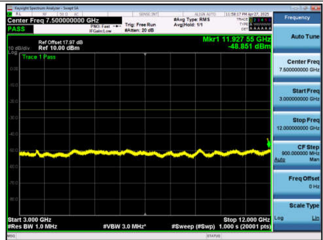
NTNV-n25-PC3-15-20-L-DFT-BPSK-Inner_1RB_Left-0.009
