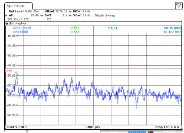
NTNV-n78(3450-3550)-PC2-30-90-H-DFT-BPSK-Inner_1R B_Left-0.009-0.15-PASS
