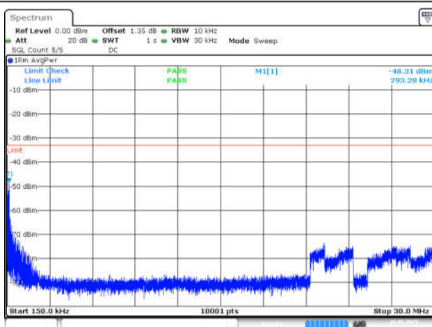
NTNV-n77(3450-3550)-PC2-30-90-L-DFT-BPSK-Inner_1R B_Left-0.15-30-PASS
