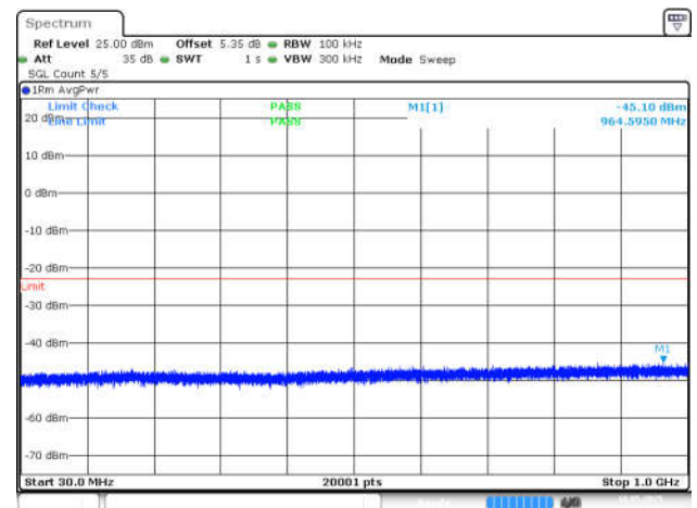
NTNV-n78(3450-3550)-PC2-30-90-H-DFT-BPSK-Inner_1R B_Left-30-1000-PASS
