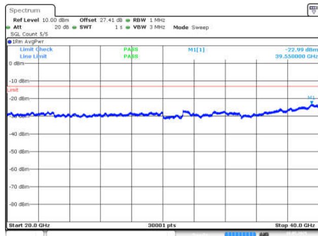
NTNV-n78(3450-3550)-PC2-30-90-M-DFT-BPSK-Inner_1R B_Left-20000-40000-PASS
