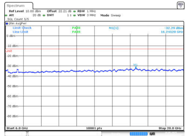
NTNV-n78(3450-3550)-PC2-30-90-M-DFT-BPSK-Inner_1R B_Left-6000-20000-PASS
