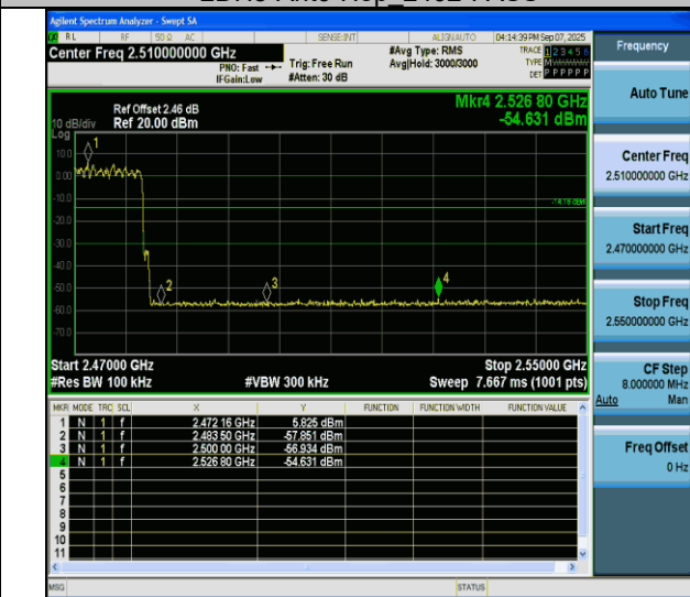
2DH5-Ant6-Hop 2480-PASS
