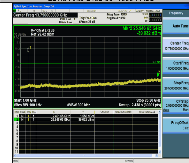
2DH5-Ant6-2402-1000~26500-PASS
