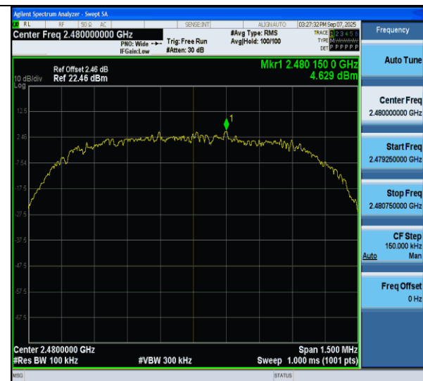
3DH5-Ant6-2480-0~Reference-PASS
