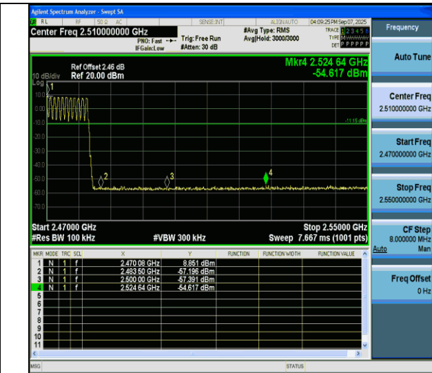
DH5-Ant6-Hop 2480-PASS
