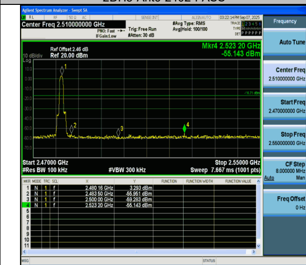
2DH5-Ant6-2480-PASS
