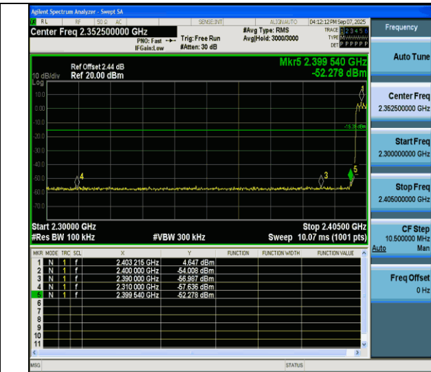
2DH5-Ant6-Hop 2402-PASS
