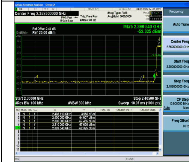
3DH5-Ant4-Hop 2402-PASS
