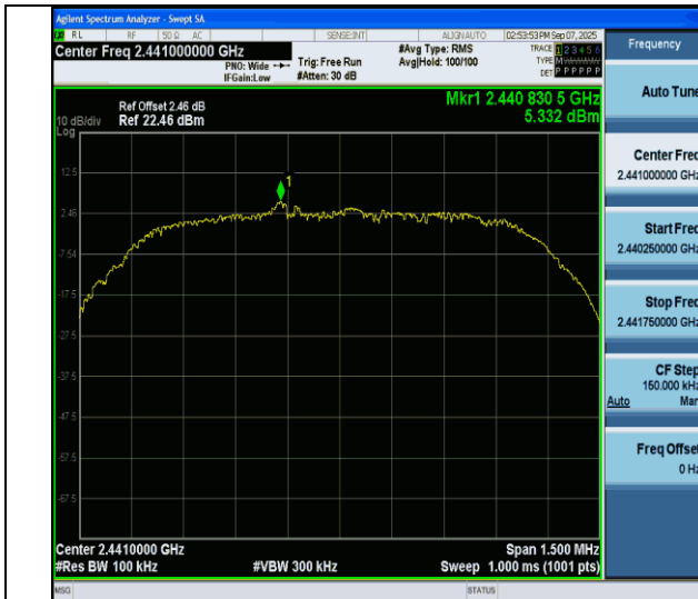
2DH5-Ant4-2441-0~Reference-PASS
