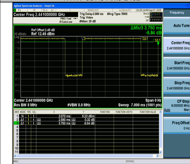
NTNV-3DH5-Ant6-2441
