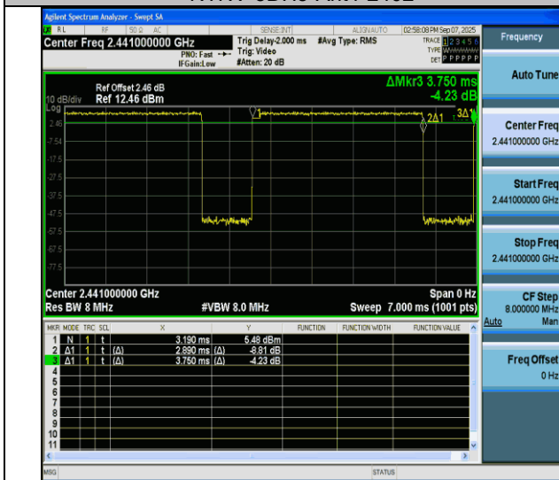
NTNV-3DH5-Ant4-2441
