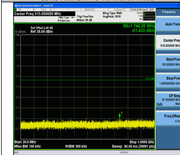
3DH5-Ant4-2441-30~1000-PASS
