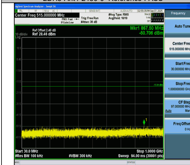
2DH5-Ant4-2480-30~1000-PASS
