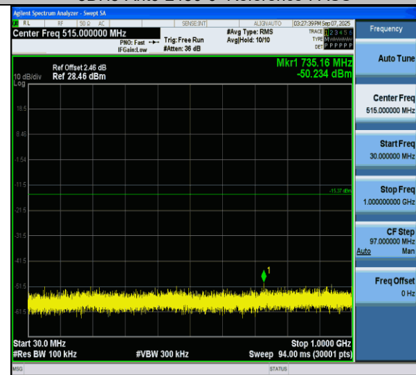
3DH5-Ant6-2480-30~1000-PASS
