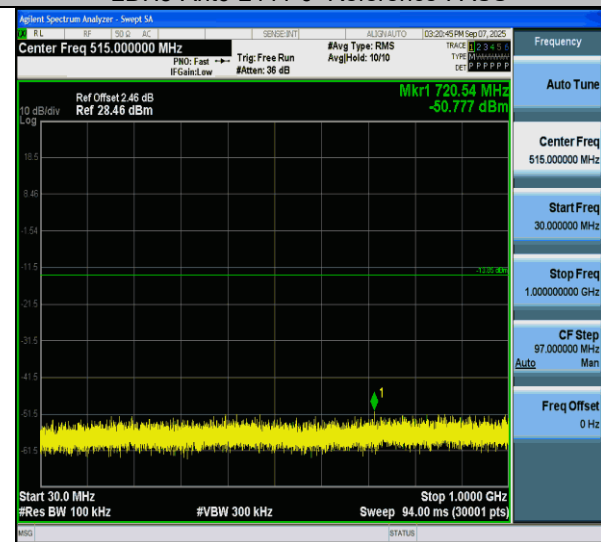
2DH5-Ant6-2441-30~1000-PASS
