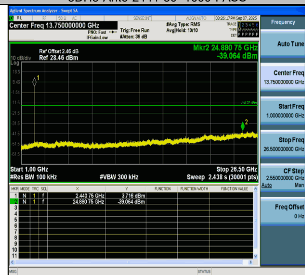
3DH5-Ant6-2441-1000~26500-PASS
