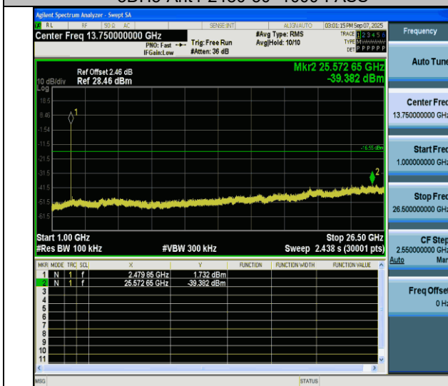
3DH5-Ant4-2480-1000~26500-PASS
