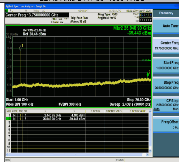
2DH5-Ant6-2441-1000~26500-PASS
