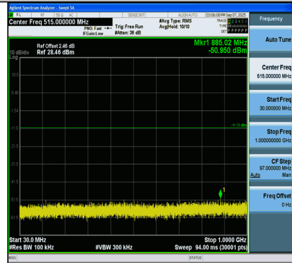
DH5-Ant6-2441-30~1000-PASS
