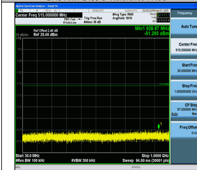
DH5-Ant4-2480-30~1000-PASS
