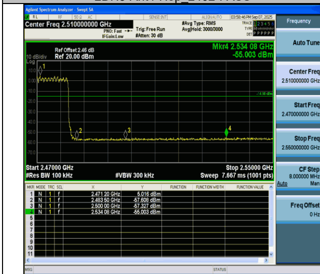
2DH5-Ant4-Hop 2480-PASS
