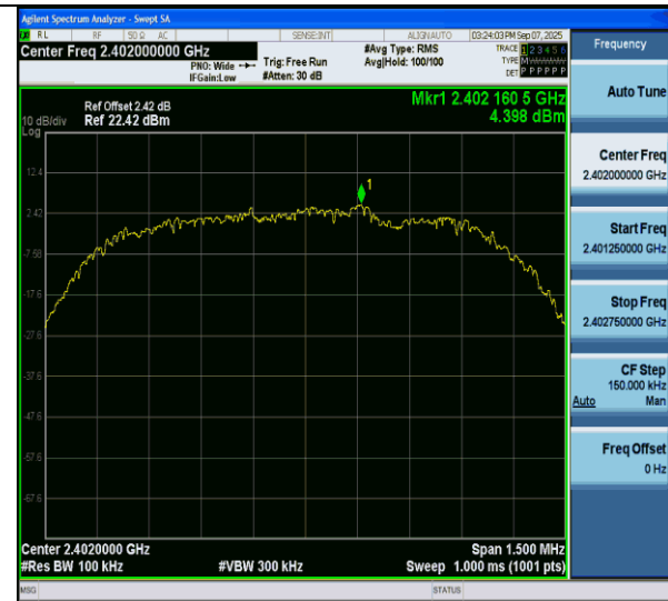
3DH5-Ant6-2402-0~Reference-PASS
