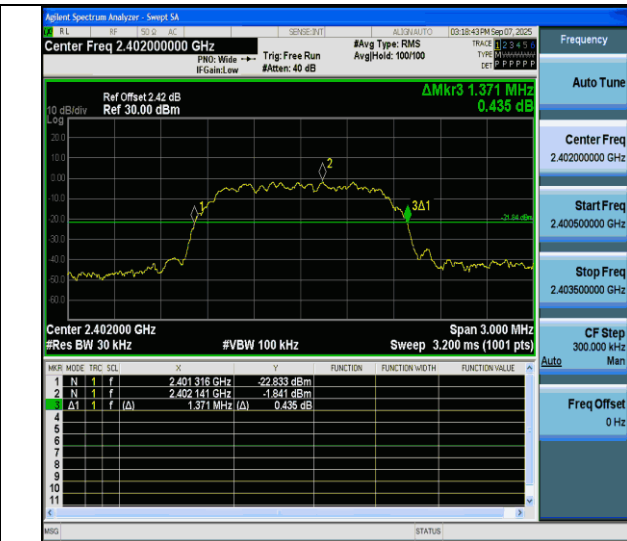
2DH5-Ant6-2402
