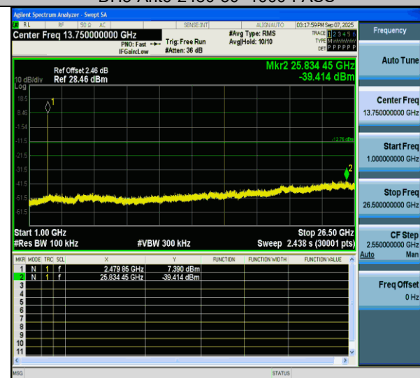
DH5-Ant6-2480-1000~26500-PASS
