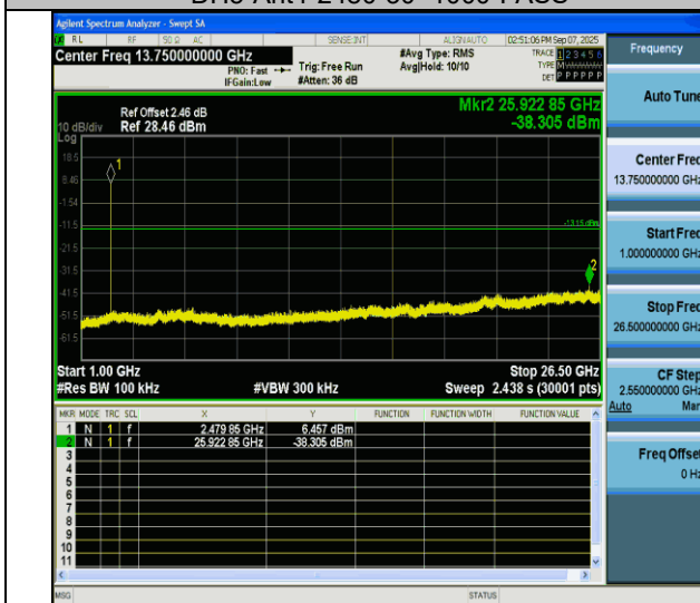
DH5-Ant4-2480-1000~26500-PASS
