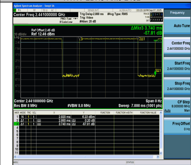
NTNV-2DH5-Ant6-2441
