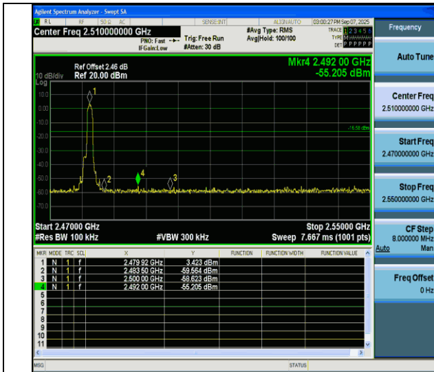
3DH5-Ant4-2480-PASS
