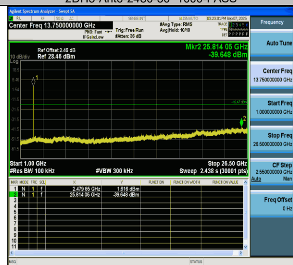
2DH5-Ant6-2480-1000~26500-PASS
