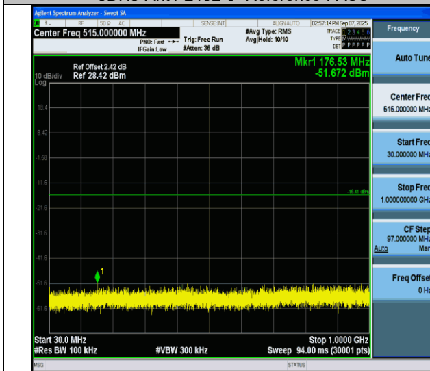
3DH5-Ant4-2402-30~1000-PASS
