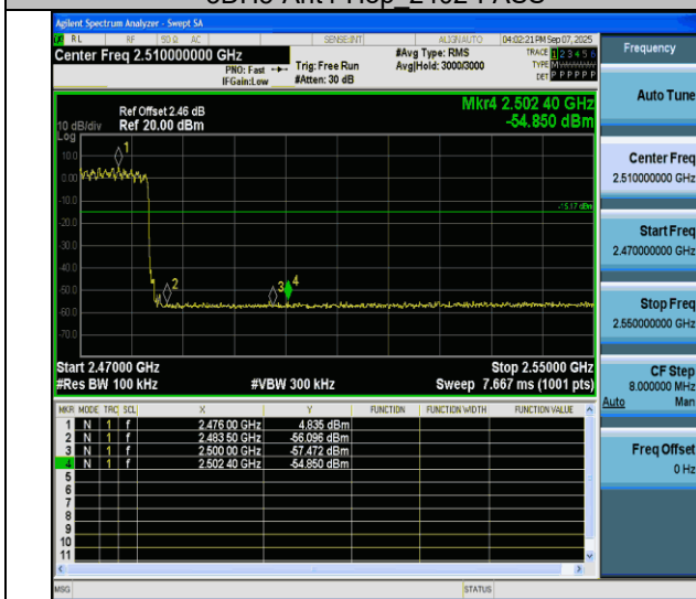
3DH5-Ant4-Hop 2480-PASS
