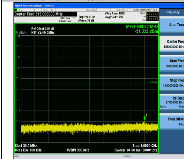
3DH5-Ant4-2480-30~1000-PASS
