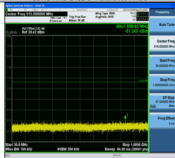
3DH5-Ant6-2402-30~1000-PASS
