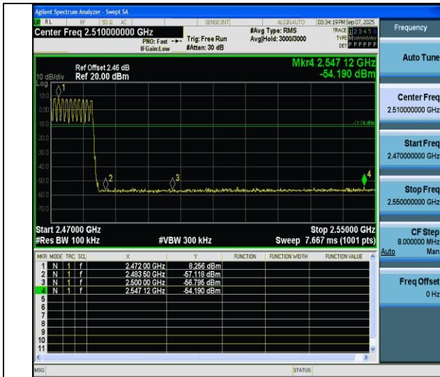
DH5-Ant4-Hop 2480-PASS
