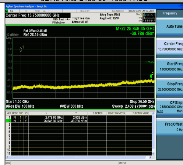
3DH5-Ant6-2480-1000~26500-PASS
