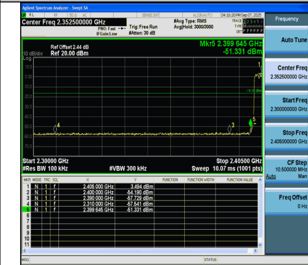
3DH5-Ant6-Hop 2402-PASS
