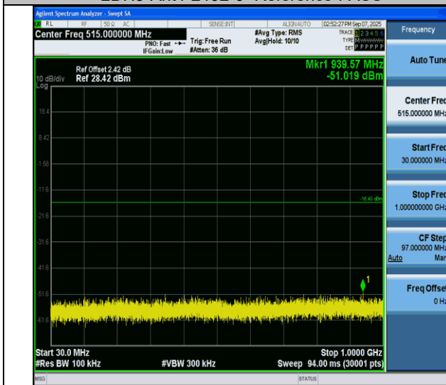
2DH5-Ant4-2402-30~1000-PASS
