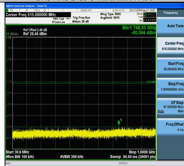
DH5-Ant6-2480-30~1000-PASS
