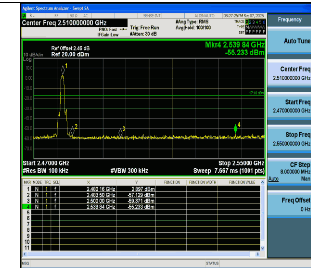
3DH5-Ant6-2480-PASS
