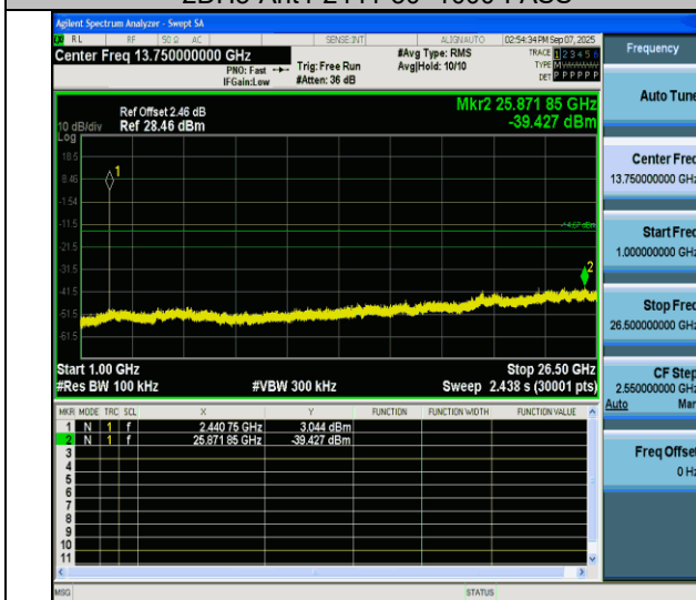
2DH5-Ant4-2441-1000~26500-PASS
