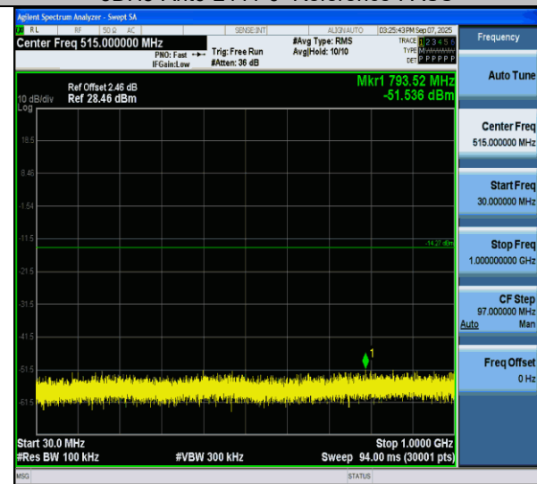
3DH5-Ant6-2441-30~1000-PASS
