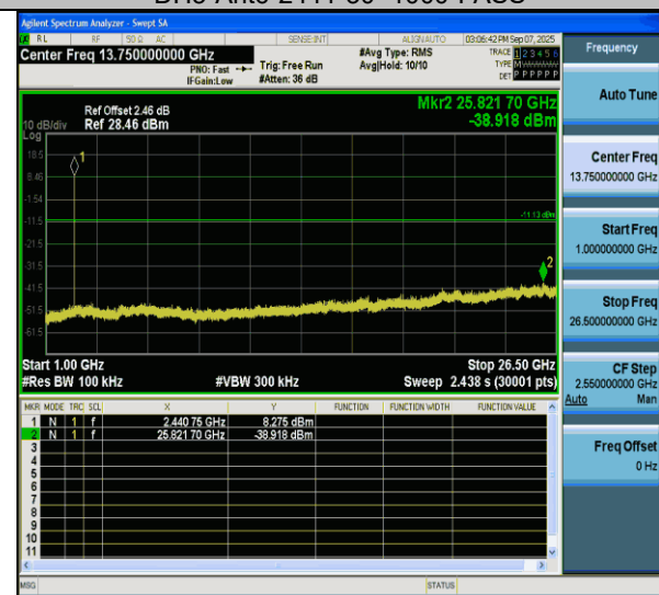
DH5-Ant6-2441-1000~26500-PASS
