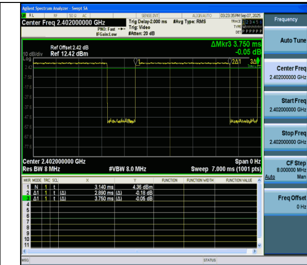
NTNV-3DH5-Ant6-2402
