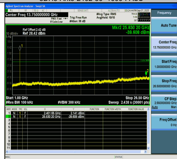
3DH5-Ant6-2402-1000~26500-PASS
