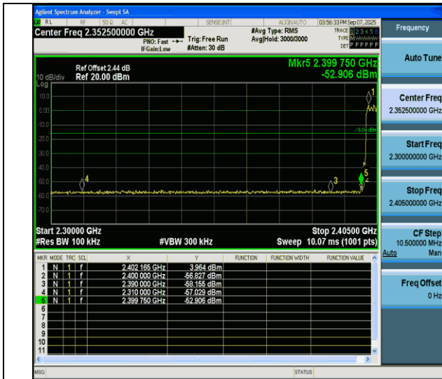
2DH5-Ant4-Hop 2402-PASS
