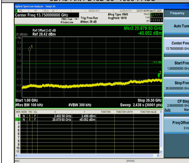
3DH5-Ant4-2402-1000~26500-PASS
