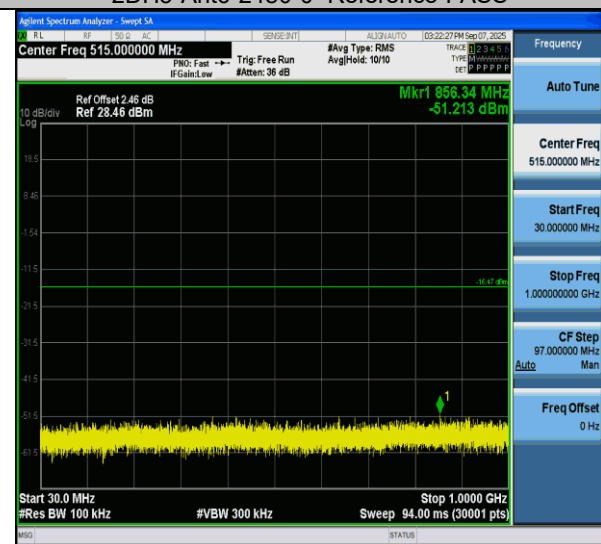
2DH5-Ant6-2480-30~1000-PASS
