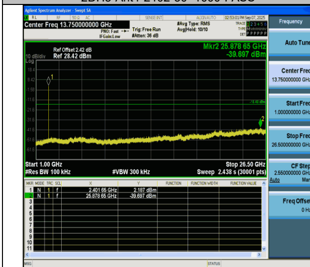
2DH5-Ant4-2402-1000~26500-PASS
