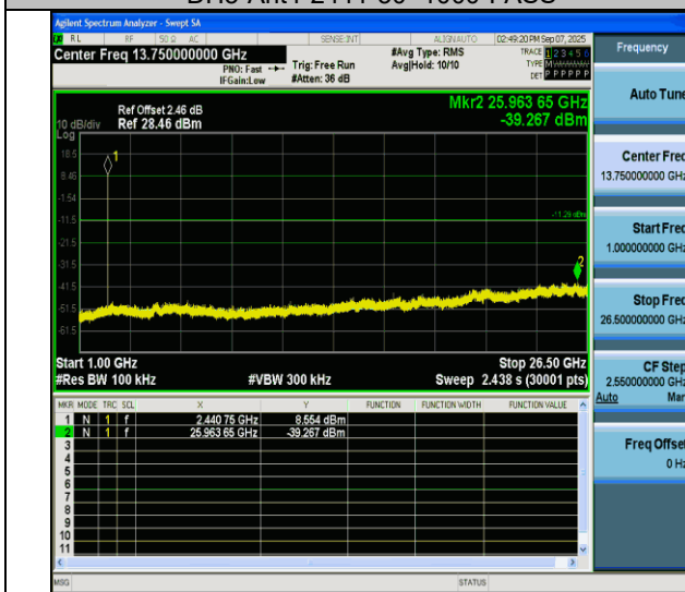
DH5-Ant4-2441-1000~26500-PASS
