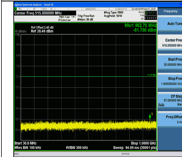
DH5-Ant4-2441-30~1000-PASS
