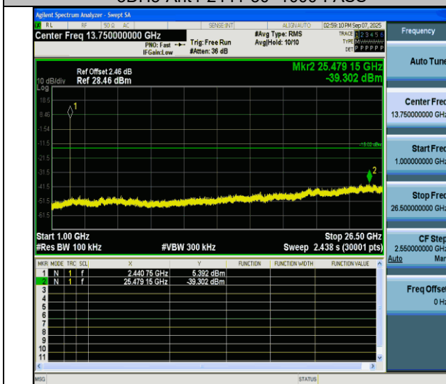
3DH5-Ant4-2441-1000~26500-PASS
