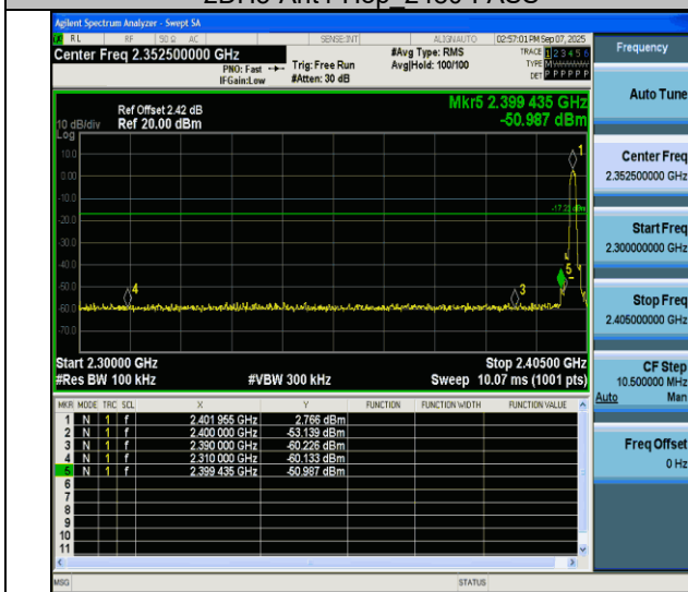
3DH5-Ant4-2402-PASS
