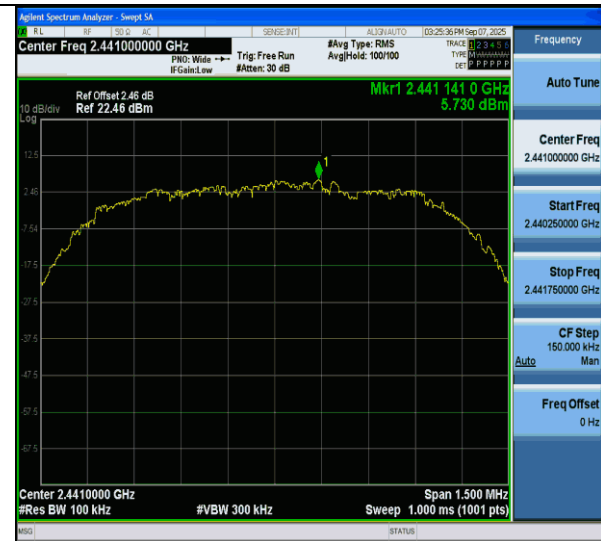
3DH5-Ant6-2441-0~Reference-PASS
