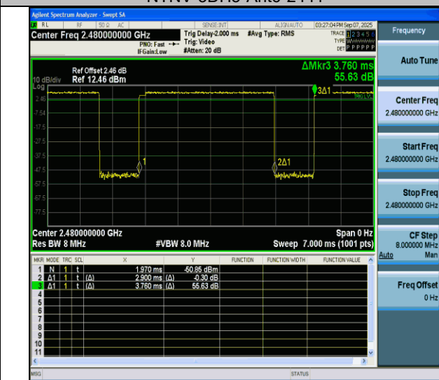
NTNV-3DH5-Ant6-2480
