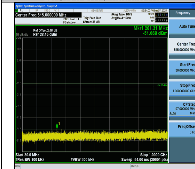
2DH5-Ant4-2441-30~1000-PASS
