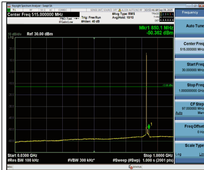
Band26(824-849)-15MHz-QPSK-26965-1RB#0-30~1000-PASS
