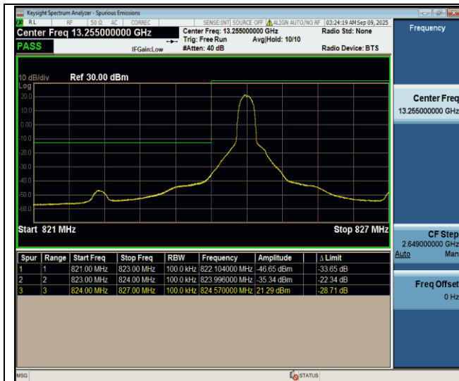
Band26(824-849)-10MHz-QPSK-26840-1RB#0-PASS
