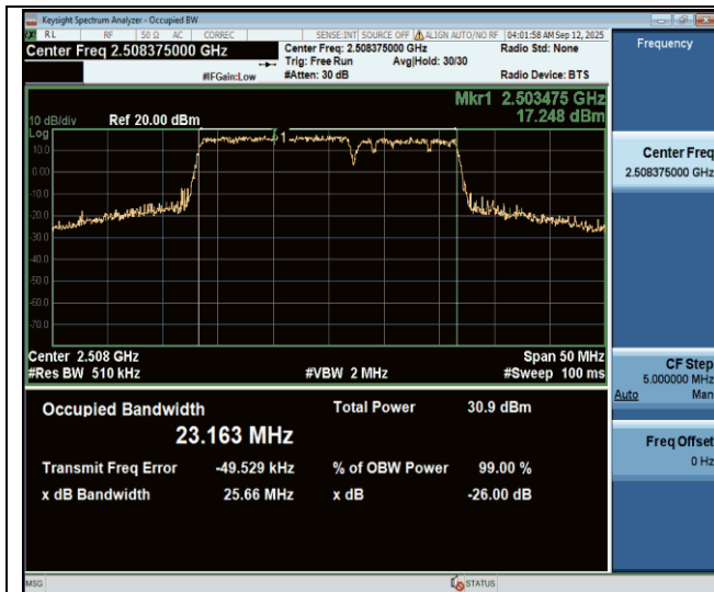
41-41-15MHz-10MHz-16QAM-16QAM-39725-39845-75RB#0-50RB#0-PASS
