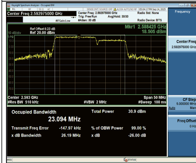
41-41-15MHz-10MHz-64QAM-64QAM-40571-40691-75RB#0-50RB#0-PASS
