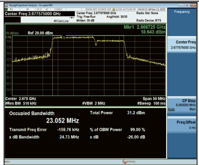
41-41-15MHz-10MHz-QPSK-QPSK-41417-41537-75RB#0-50RB#0-PASS
