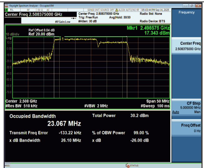
41-41-15MHz-10MHz-64QAM-64QAM-39725-39845-75RB#0-50RB#0-PASS
