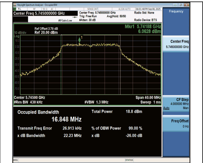
11a-CDD-Ant7-5745
