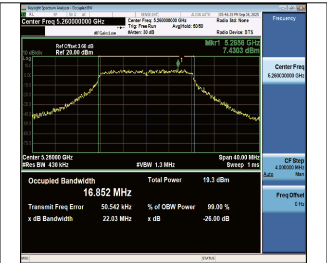
11a-CDD-Ant7-5260
