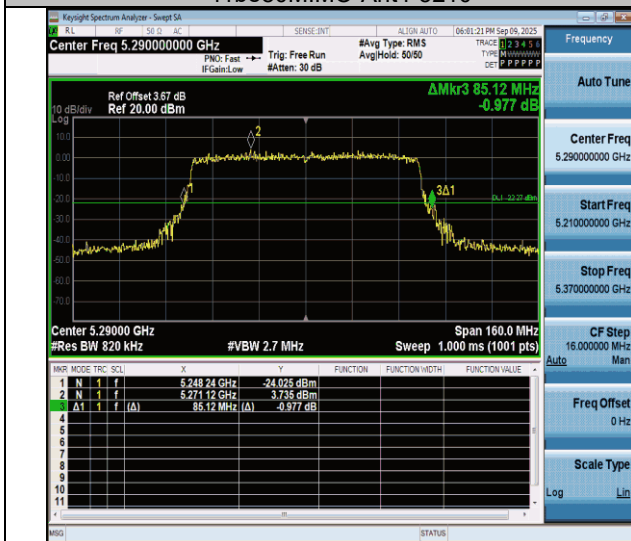
11be80MIMO-Ant4-5290
