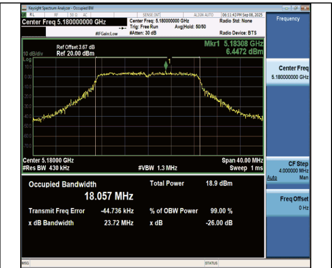
11n20MIMO-Ant7-5180
