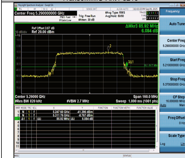
11ax80MIMO-Ant4-5290
