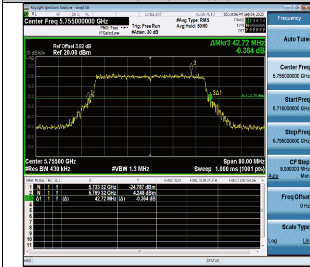
11be40MIMO-Ant4-5755
