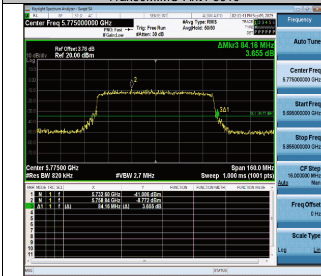
11ax80MIMO-Ant4-5775
