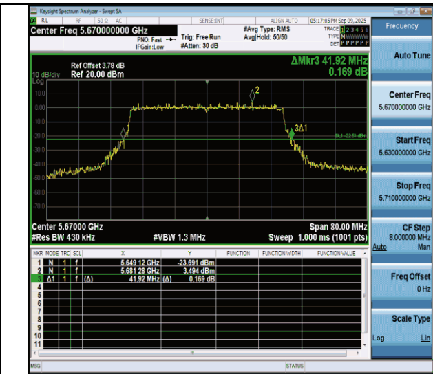
11be40MIMO-Ant7-5670
