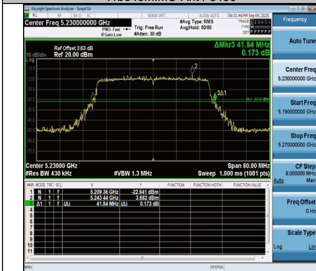
11be40MIMO-Ant4-5230
