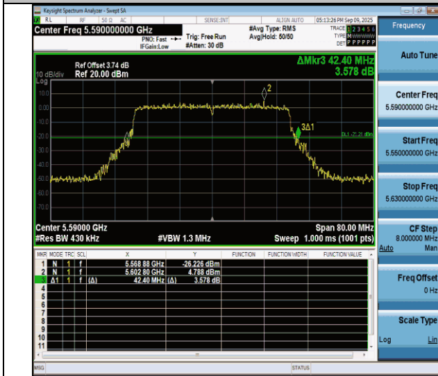
11be40MIMO-Ant4-5590
