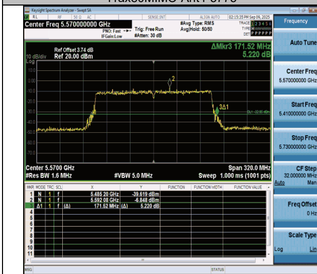
11ax160MIMO-Ant4-5570
