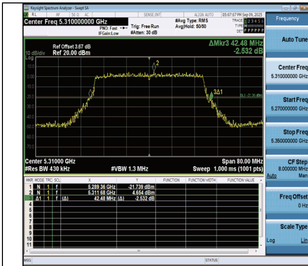
11be40MIMO-Ant4-5310
