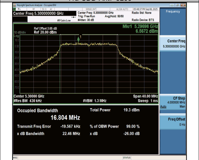
11a-CDD-Ant7-5300
