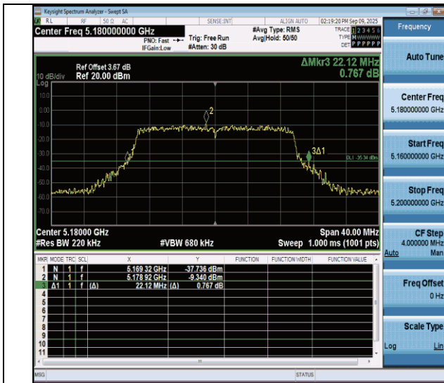
11be20MIMO-Ant4-5180
