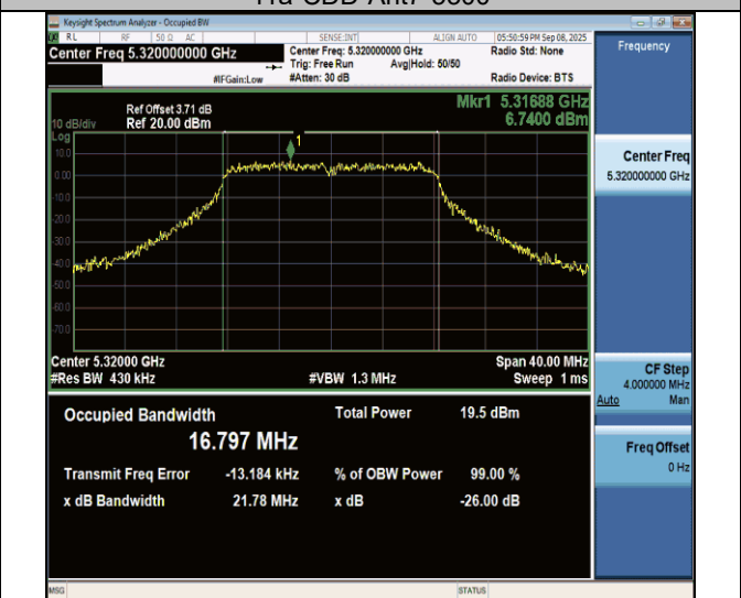
11a-CDD-Ant7-5320
