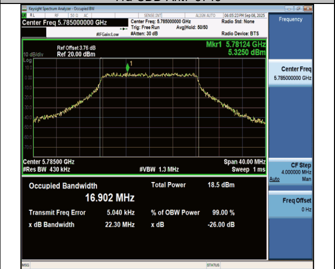
11a-CDD-Ant7-5785
