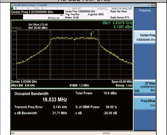
11a-CDD-Ant7-5825
