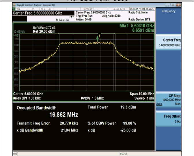
11a-CDD-Ant7-5600
