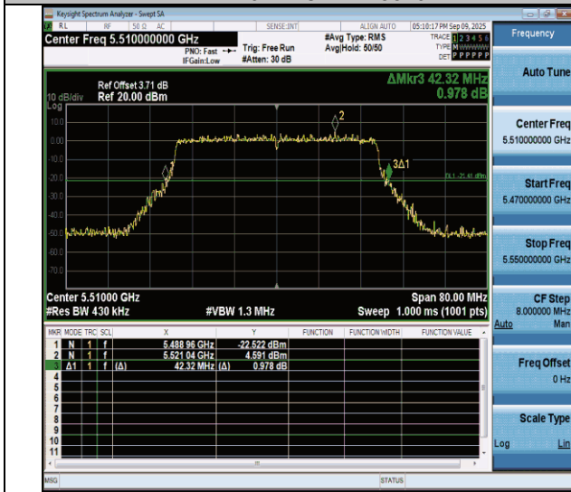
11be40MIMO-Ant4-5510
