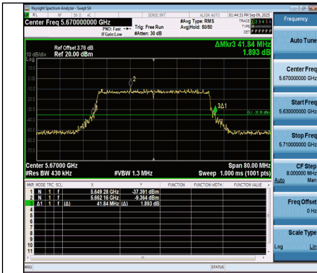
11ax40MIMO-Ant4-5670
