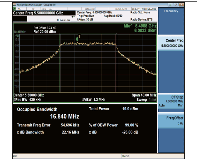
11a-CDD-Ant7-5500
