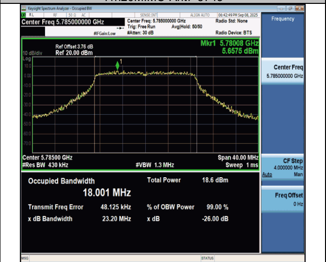
11n20MIMO-Ant7-5785
