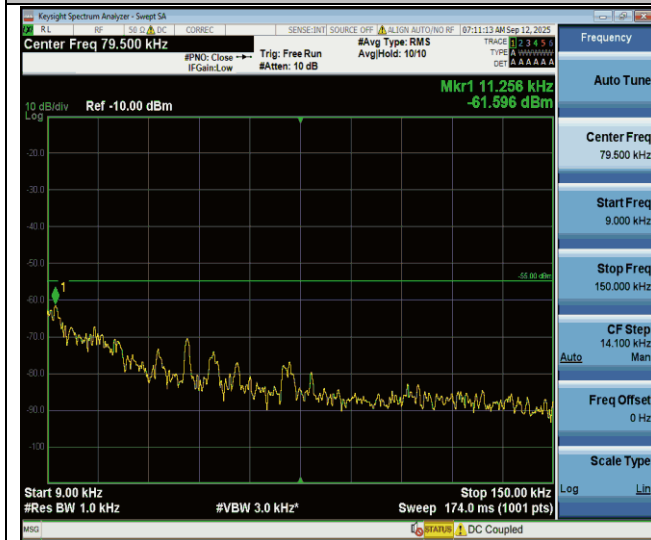
41-41-20MHz-20MHz-QPSK-QPSK-40521-40719-1RB#0-ORB#0- 0.009~0.15MHz-PASS
