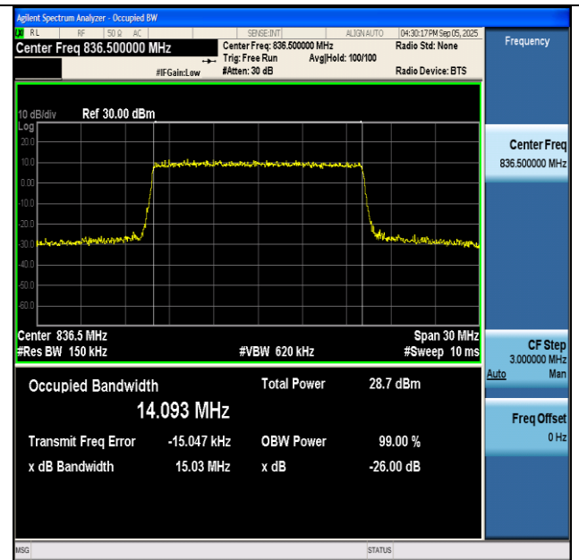
NTVN-n5-PC3-15-15-M-CP-16QAM-Outer_Full-Ant1-PASS
