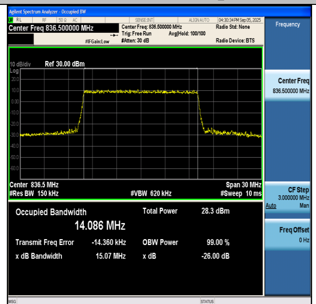
NTVN-n5-PC3-15-15-M-CP-256QAM-Outer_Full-Ant1-PASS
