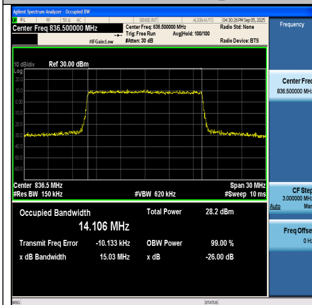
NTVN-n5-PC3-15-15-M-CP-64QAM-Outer_Full-Ant1-PASS
