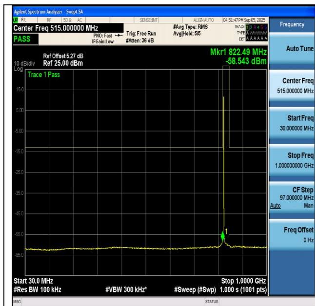
NTNV-n5-PC3-15-20-M-CP-QPSK-Edge_1RB_Left-30-1000- PASS
