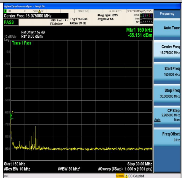
NTVN-n5-PC3-15-20-L-CP-QPSK-Edge_1RB_Left-0.15-30-PASS
