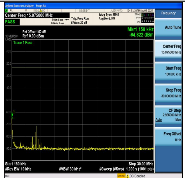
NTNV-n5-PC3-15-20-M-DFT-BPSK-Edge_1RB_Left-12000- 20000-PASS
