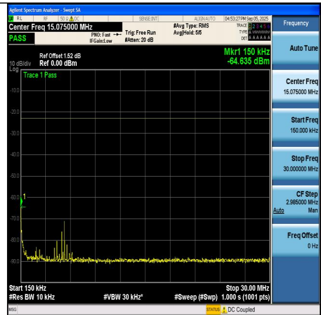
NTVN-n5-PC3-15-20-H-DFT-BPSK-Edge_1RB_Left-0.15-30- PASS
