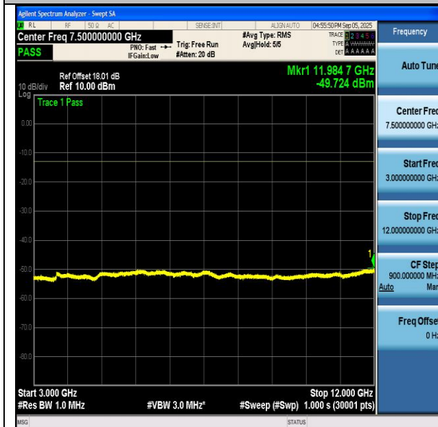
NTNV-n5-PC3-15-20-H-CP-QPSK-Edge_1RB_Left-3000-12000- PASS
