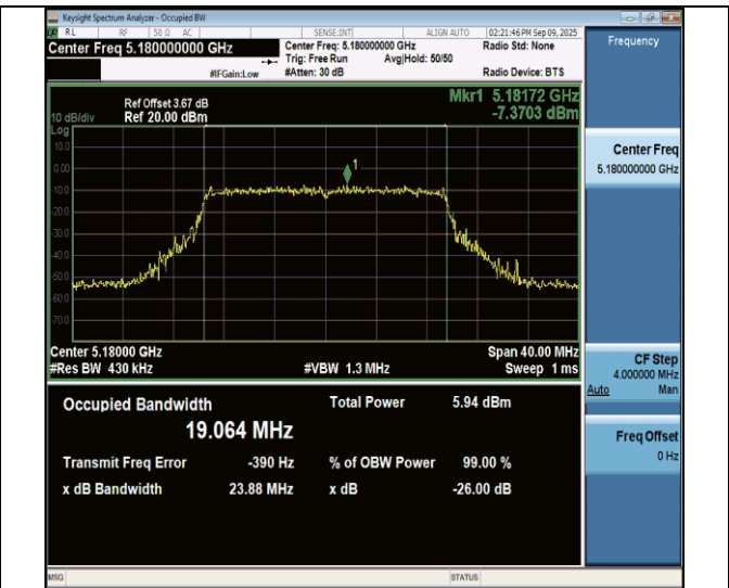
11be20MIMO-Ant7-5180
