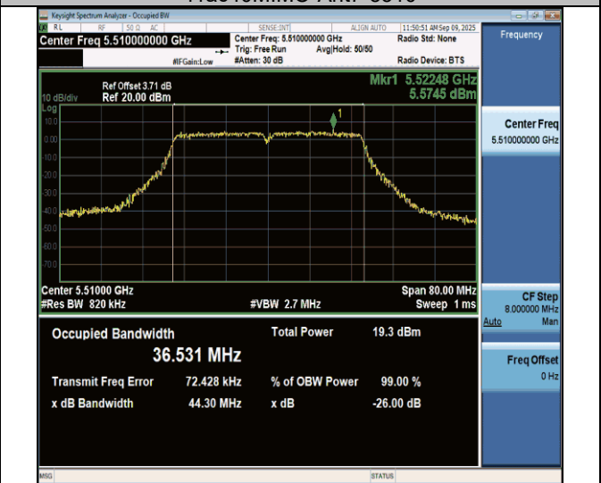
11ac40MIMO-Ant7-5510
