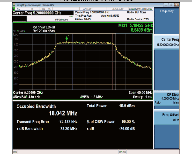
11ac20MIMO-Ant7-5200
