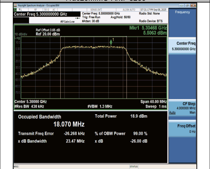
11ac20MIMO-Ant7-5300
