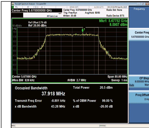
11be40MIMO-Ant4-5670
