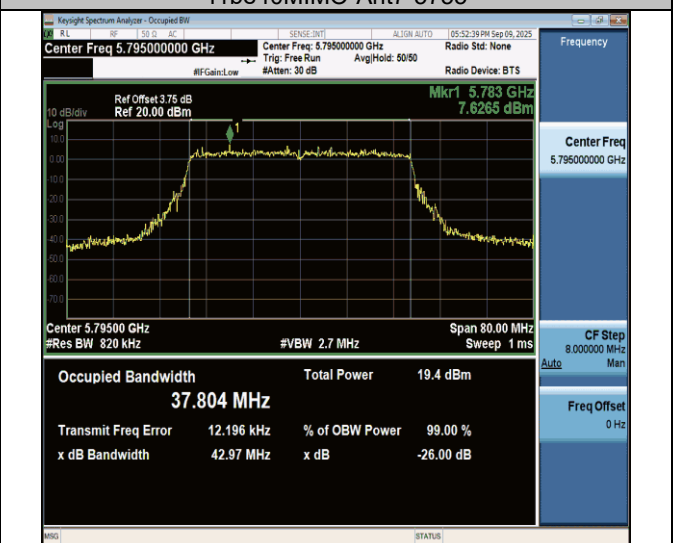
11be40MIMO-Ant7-5795
