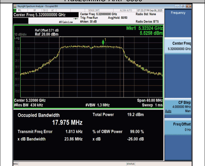
11ac20MIMO-Ant7-5320
