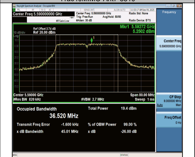
11ac40MIMO-Ant7-5590
