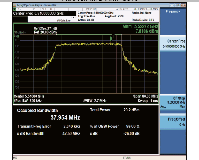
11be40MIMO-Ant7-5510
