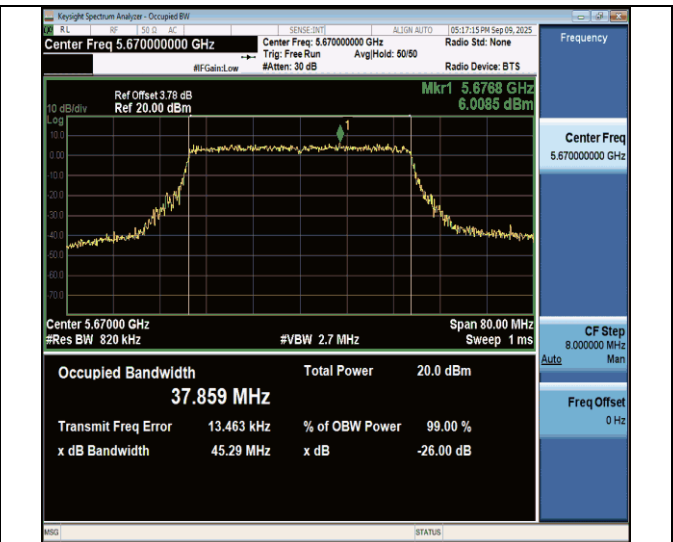
11be40MIMO-Ant7-5670
