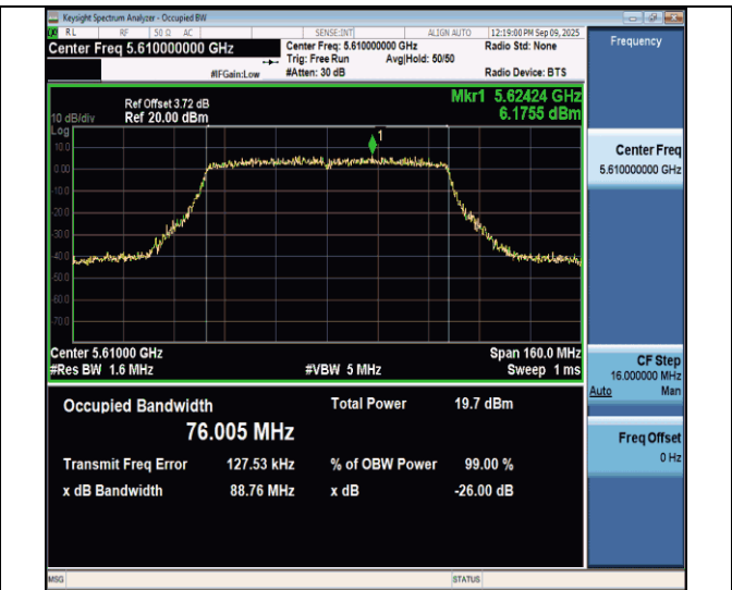
11ac80MIMO-Ant7-5610
