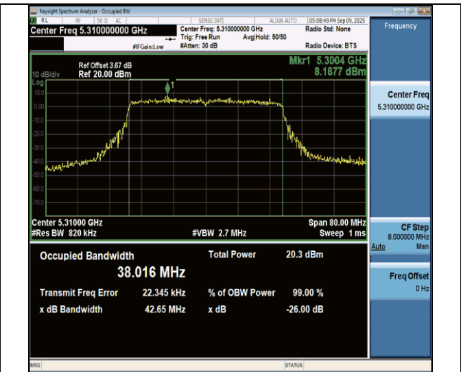
11be40MIMO-Ant7-5310
