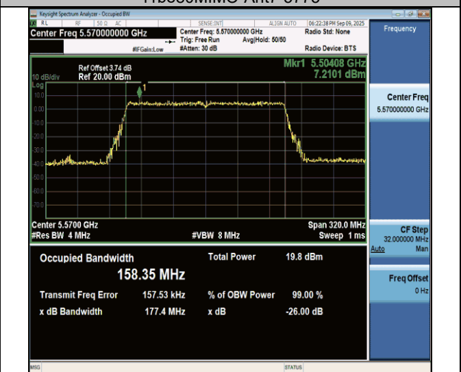
11be160MIMO-Ant7-5570
