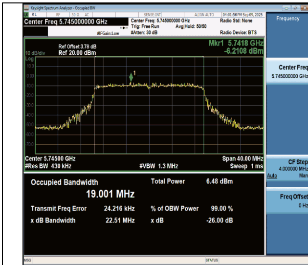
11be20MIMO-Ant4-5745
