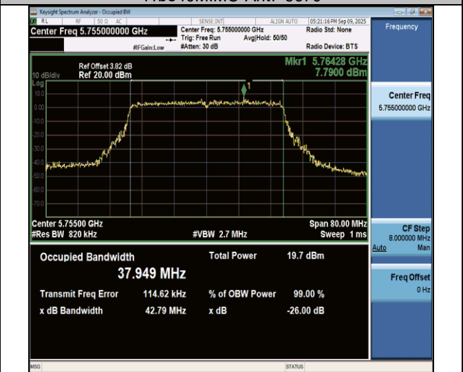
11be40MIMO-Ant7-5755
