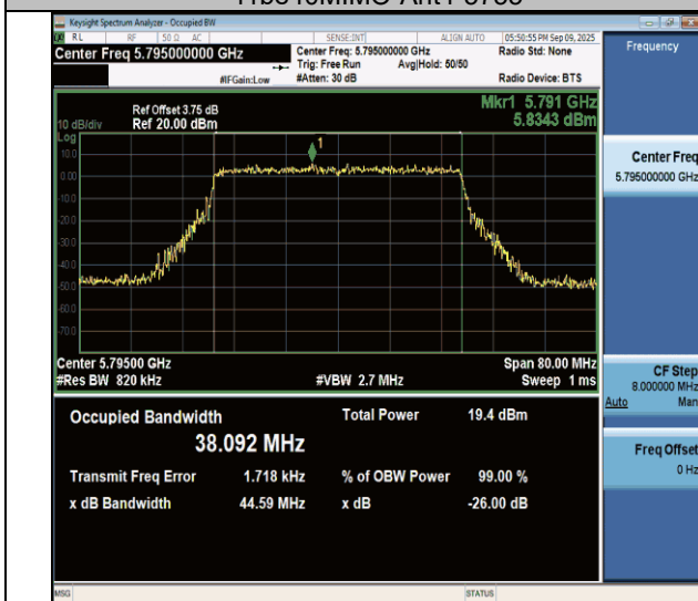
11be40MIMO-Ant4-5795
