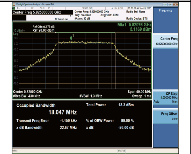
11ac20MIMO-Ant7-5825
