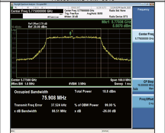
11ac80MIMO-Ant7-5775
