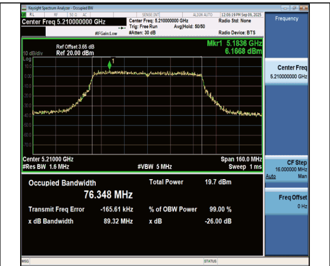
11ac80MIMO-Ant7-5210
