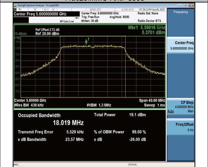
11ac20MIMO-Ant7-5600
