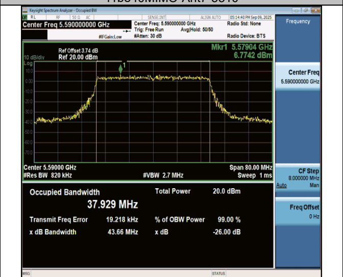
11be40MIMO-Ant7-5590
