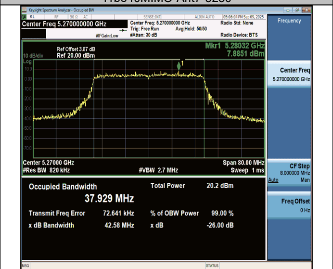
11be40MIMO-Ant7-5270
