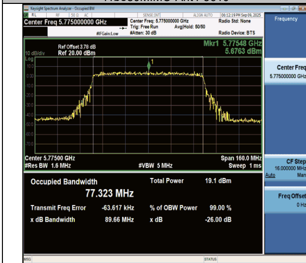
11be80MIMO-Ant4-5775
