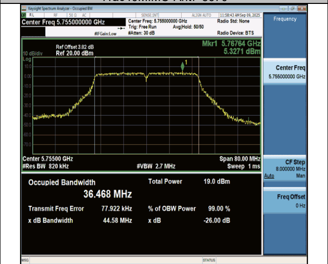
11ac40MIMO-Ant7-5755
