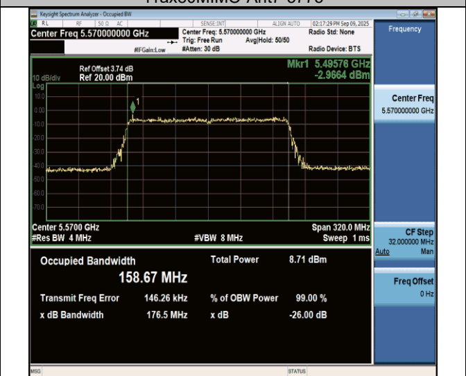
11ax160MIMO-Ant7-5570
