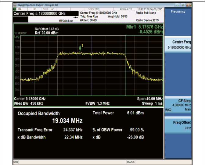
11ax20MIMO-Ant7-5180
