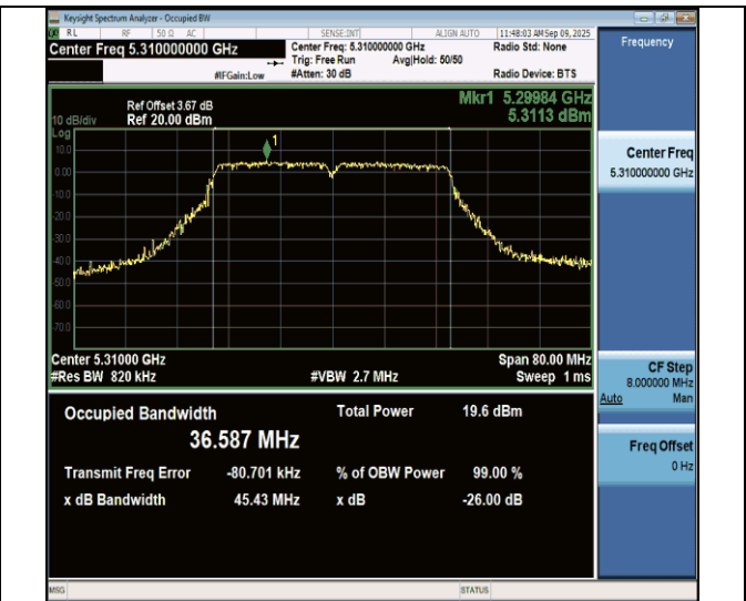
11ac40MIMO-Ant7-5310
