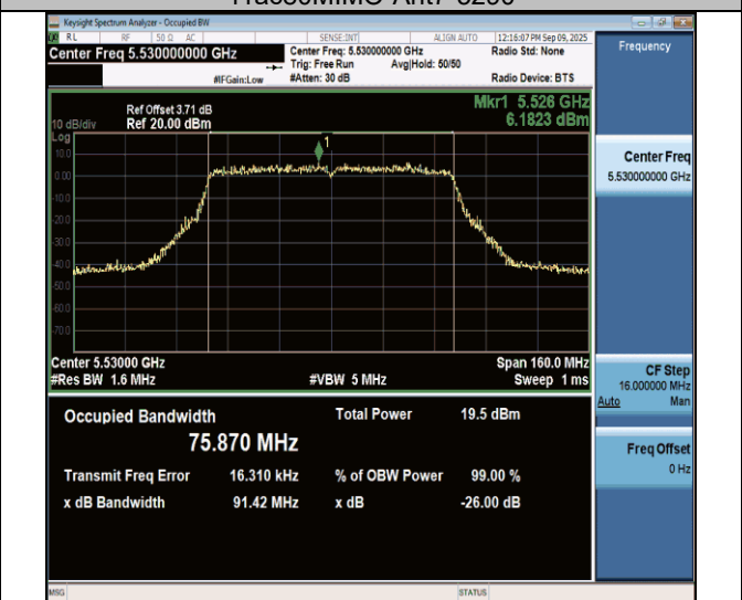
11ac80MIMO-Ant7-5530
