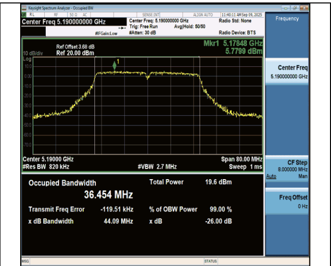
11ac40MIMO-Ant7-5190
