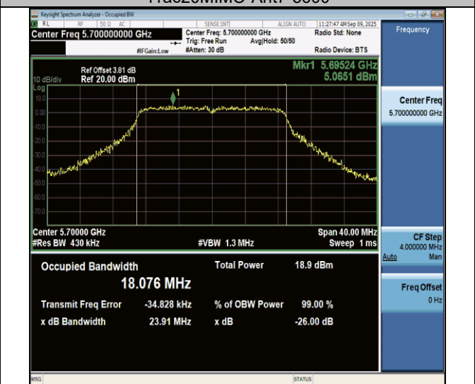
11ac20MIMO-Ant7-5700
