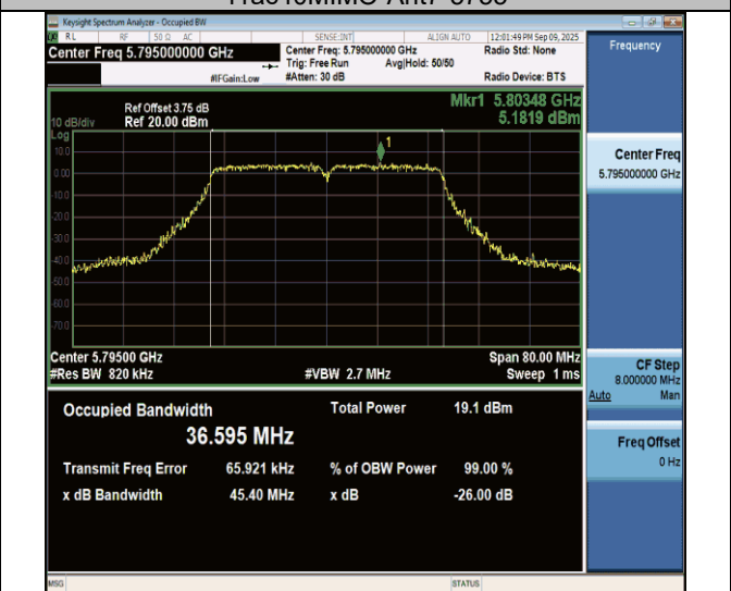
11ac40MIMO-Ant7-5795
