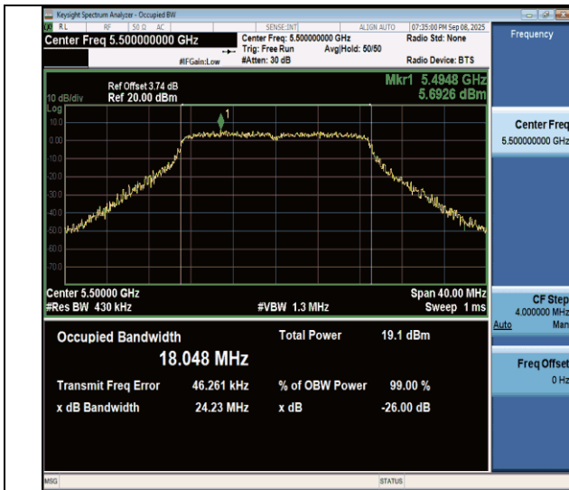
11ac20MIMO-Ant4-5500
