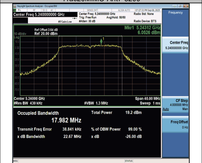
11ac20MIMO-Ant7-5240
