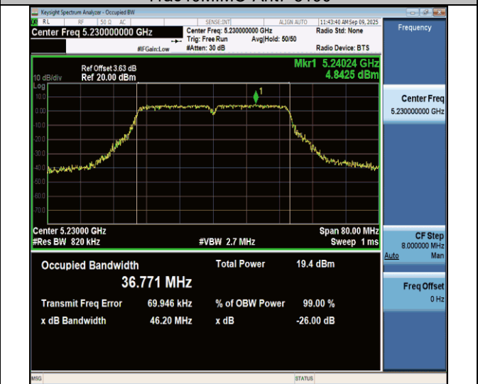
11ac40MIMO-Ant7-5230
