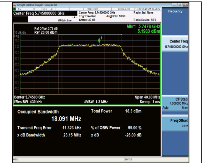
11ac20MIMO-Ant7-5745
