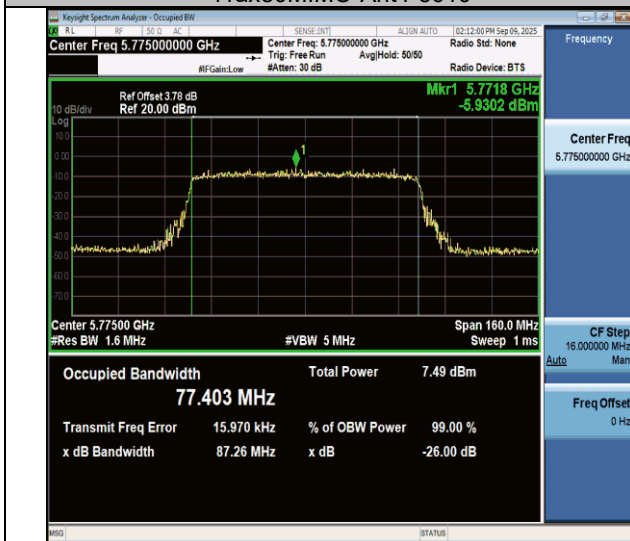
11ax80MIMO-Ant4-5775
