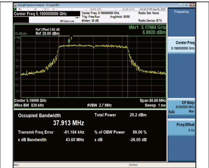
11be40MIMO-Ant7-5190
