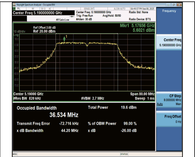
11n40MIMO-Ant7-5190
