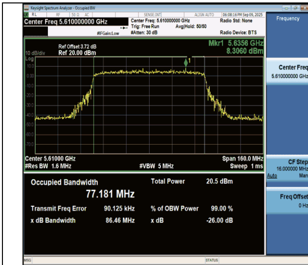
11be80MIMO-Ant4-5610
