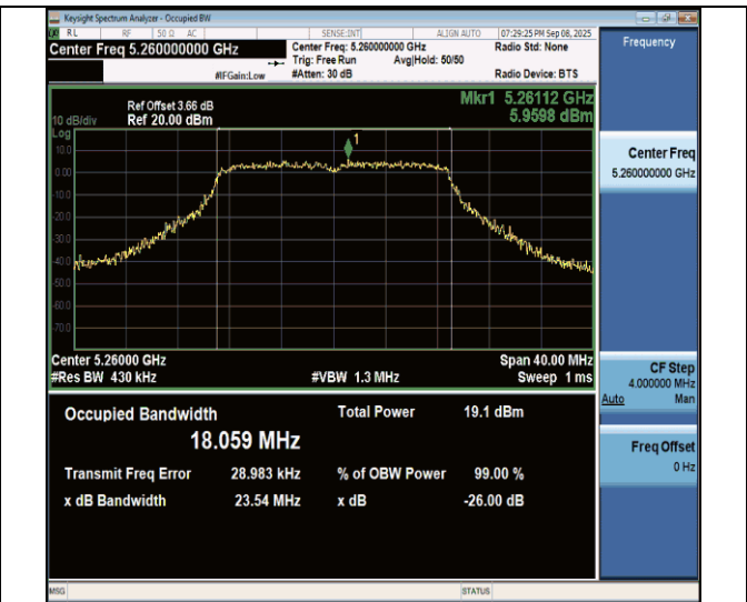
11ac20MIMO-Ant7-5260
