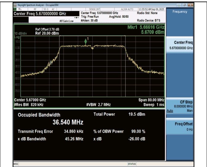
11ac40MIMO-Ant7-5670
