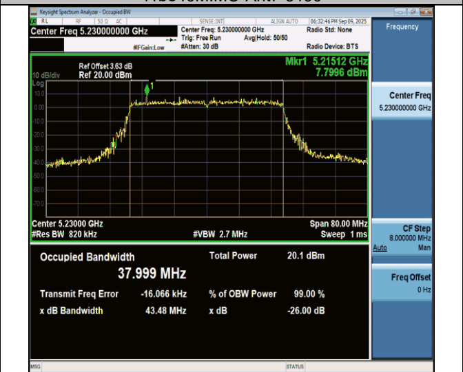
11be40MIMO-Ant7-5230
