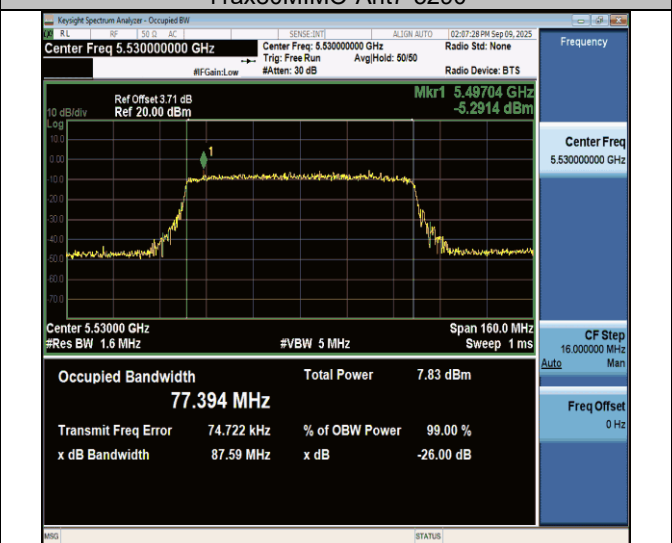
11ax80MIMO-Ant7-5530
