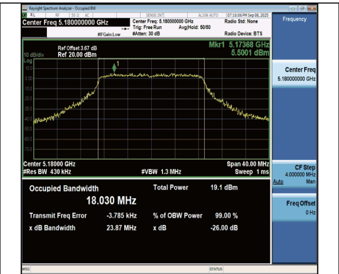
11ac20MIMO-Ant7-5180
