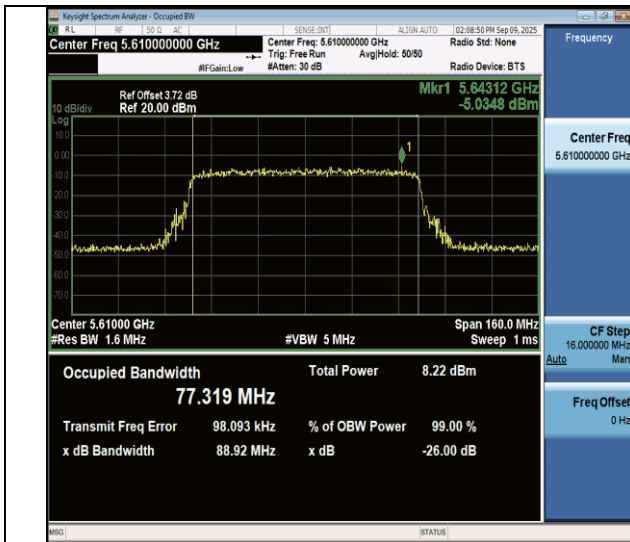
11ax80MIMO-Ant4-5610
