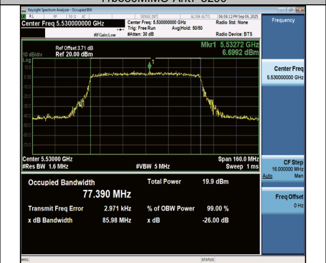
11be80MIMO-Ant7-5530
