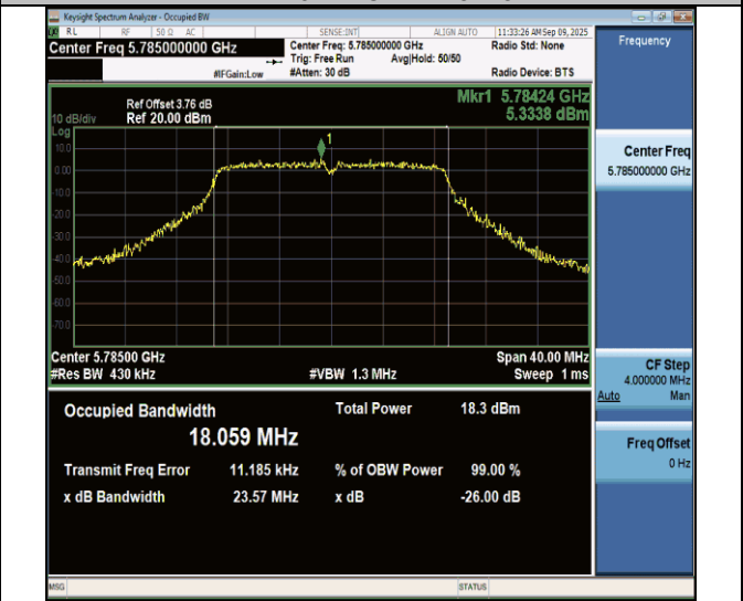
11ac20MIMO-Ant7-5785
