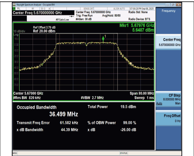
11n40MIMO-Ant7-5670
