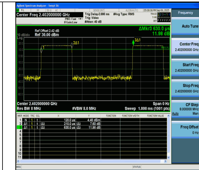
NTVN-BLE 2M-Ant6-2402
