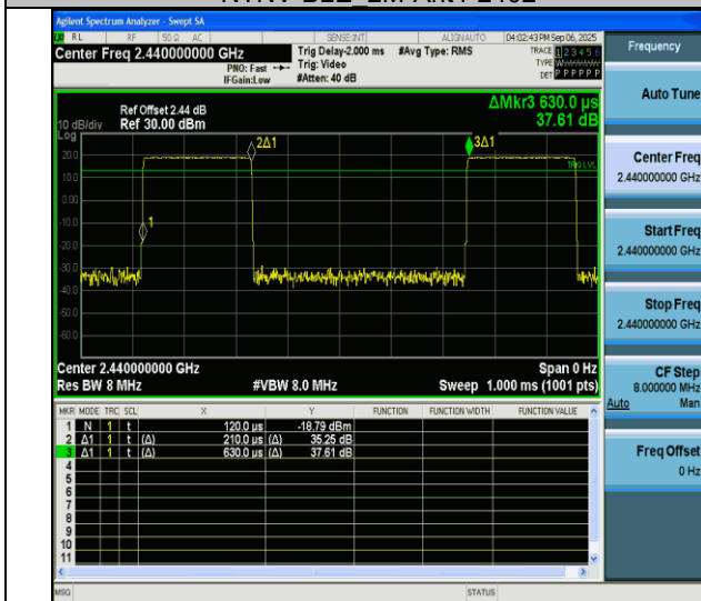
NTVN-BLE 2M-Ant4-2440
