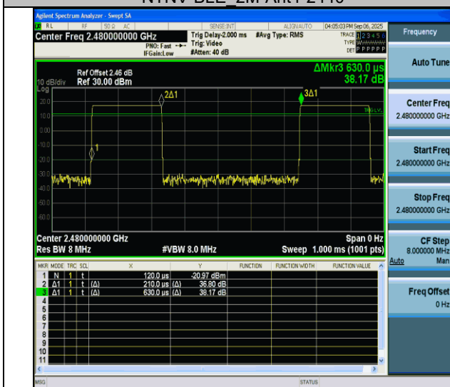
NTVN-BLE 2M-Ant4-2480
