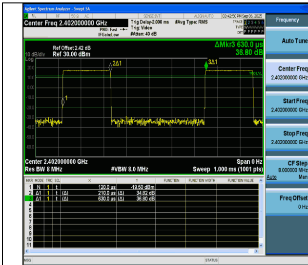
NTVN-BLE 2M-Ant4-2402
