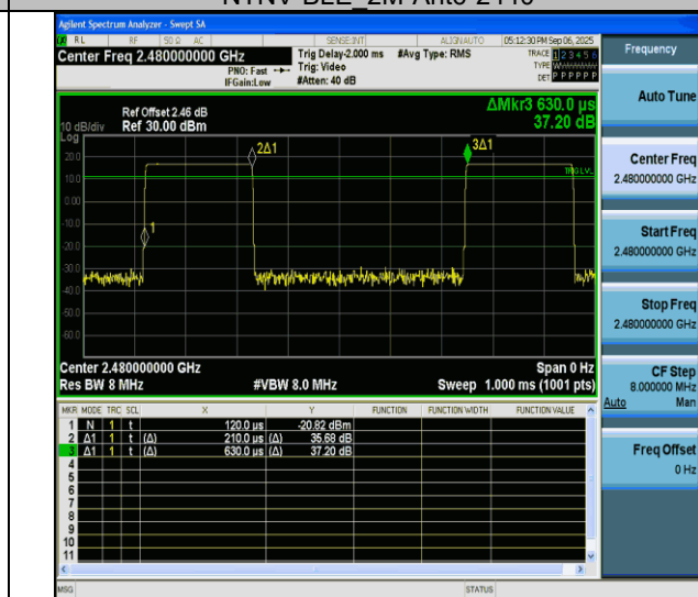
NTVN-BLE 2M-Ant6-2480
