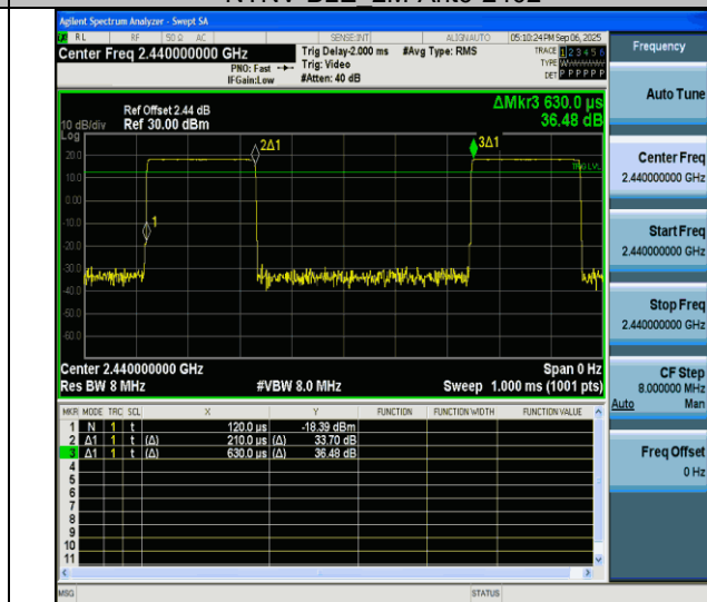
NTVN-BLE 2M-Ant6-2440
