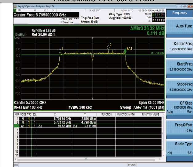
11ac40MIMO-Ant7-5755-PASS
