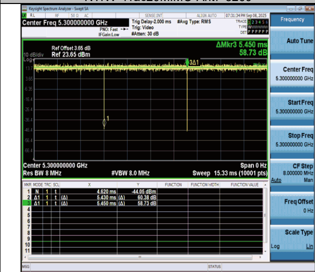
NTNV-11ac20MIMO-Ant7-5300
