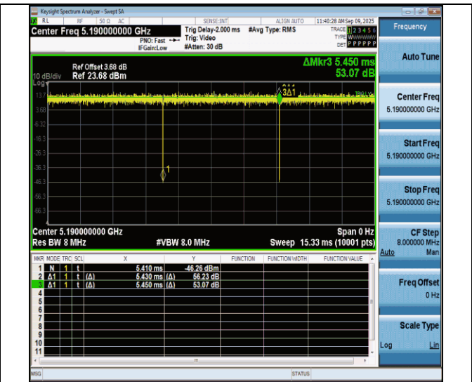
NTNV-11ac40MIMO-Ant7-5190
