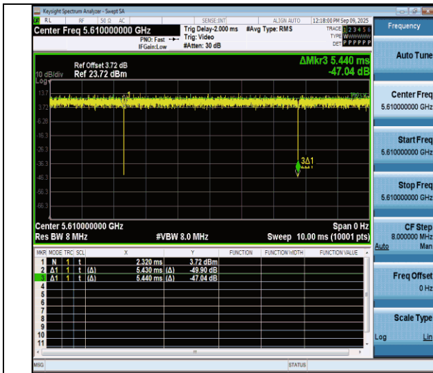
NTNV-11ac80MIMO-Ant4-5610
