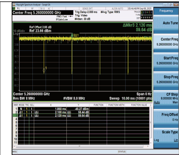
NTVN-11a-CDD-Ant7-5260
