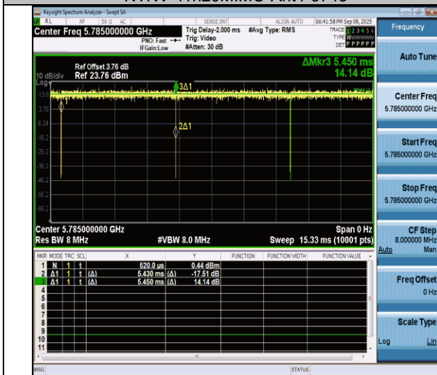
NTNV-11n20MIMO-Ant4-5785
