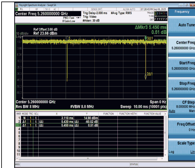
NTNV-11ac20MIMO-Ant4-5260
