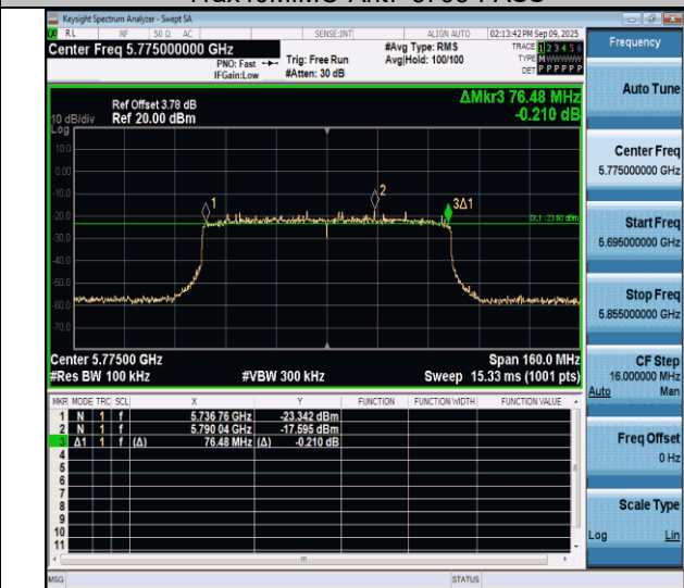
11ax80MIMO-Ant7-5775-PASS
