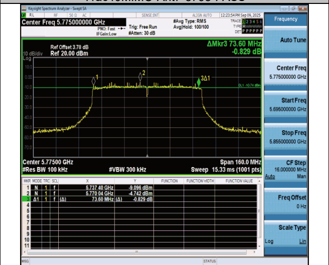
11ac80MIMO-Ant7-5775-PASS
