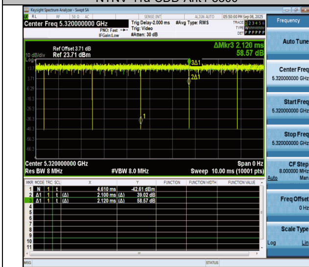
NTVN-11a-CDD-Ant4-5320
