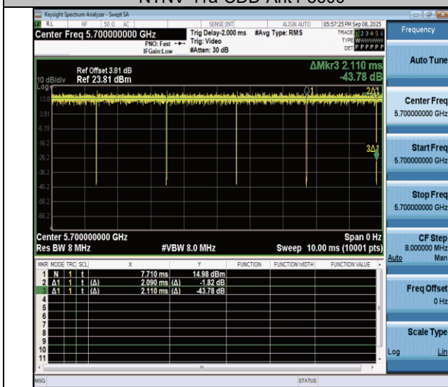
NTVN-11a-CDD-Ant4-5700
