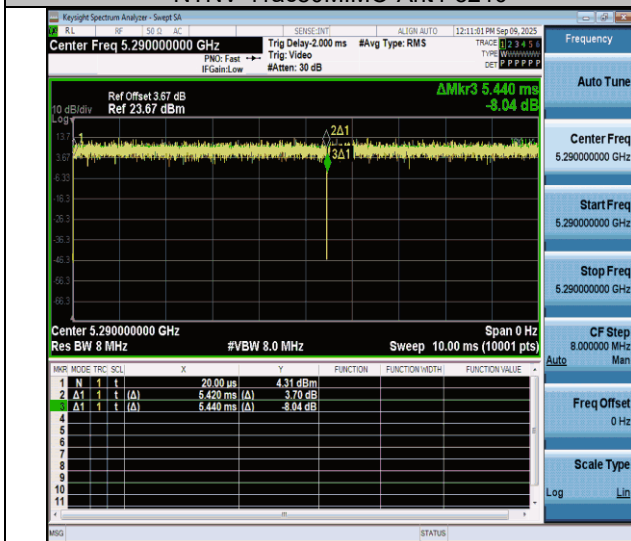
NTNV-11ac80MIMO-Ant4-5290
