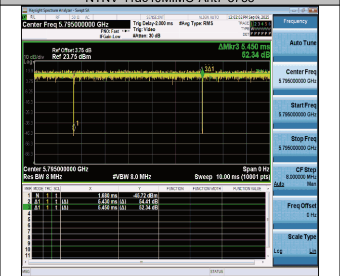
NTNV-11ac40MIMO-Ant7-5795
