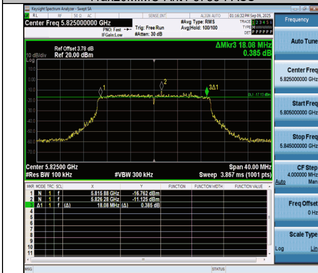
11ax20MIMO-Ant4-5825-PASS
