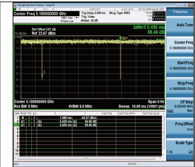
NTNV-11ac20MIMO-Ant7-5180
