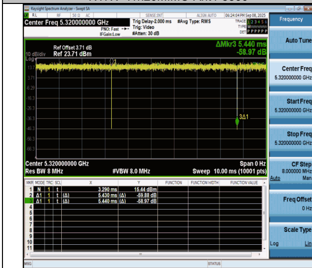
NTNV-11n20MIMO-Ant4-5320
