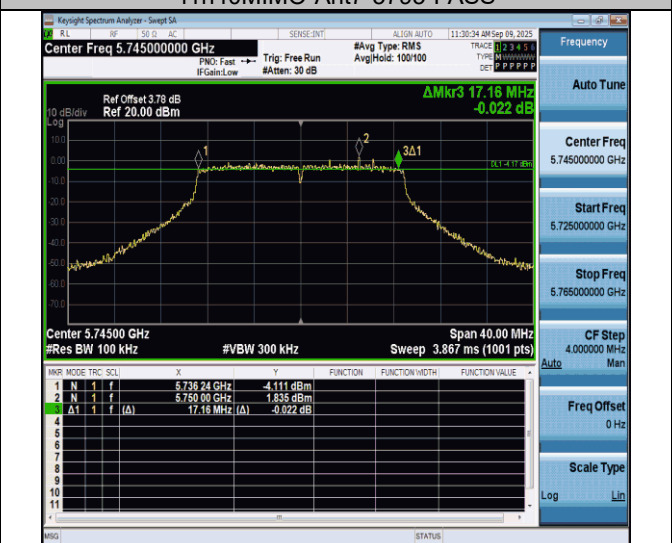
11ac20MIMO-Ant7-5745-PASS
