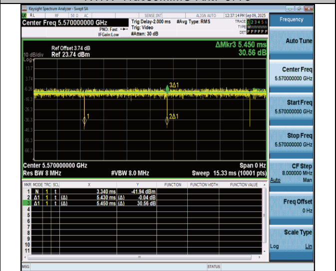
NTNV-11ac160MIMO-Ant7-5570
