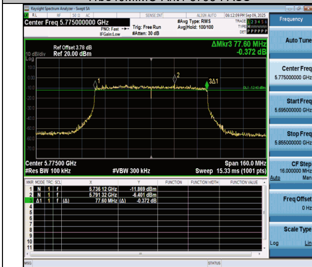
11be80MIMO-Ant4-5775-PASS
