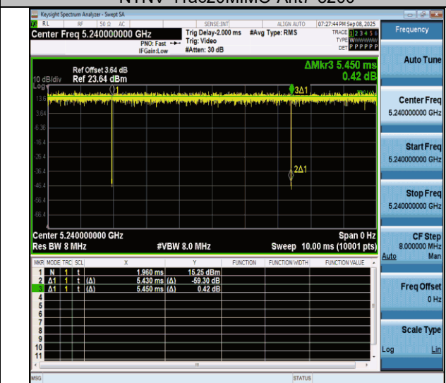
NTNV-11ac20MIMO-Ant7-5240
