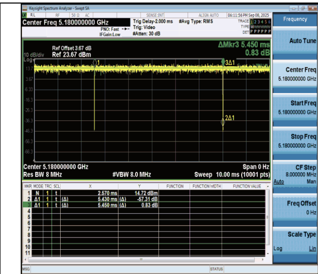
NTNV-11n20MIMO-Ant7-5180
