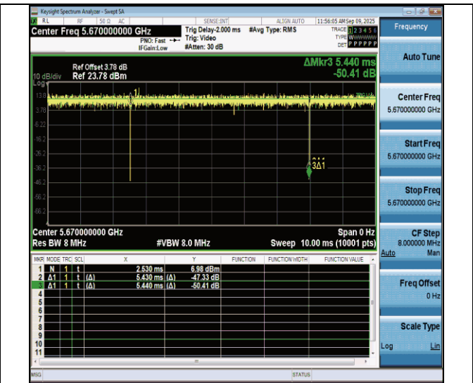
NTNV-11ac40MIMO-Ant7-5670
