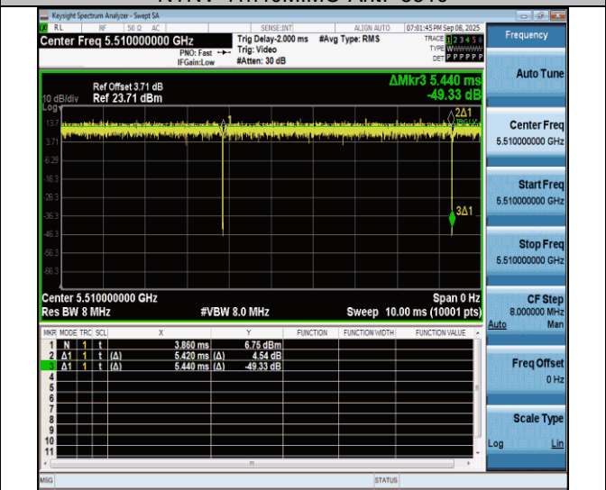
NTNV-11n40MIMO-Ant7-5510
