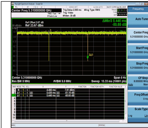
NTNV-11n40MIMO-Ant4-5310
