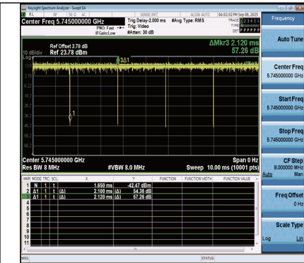
NTNV-11a-CDD-Ant7-5745
