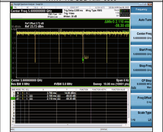
NTVN-11a-CDD-Ant7-5600
