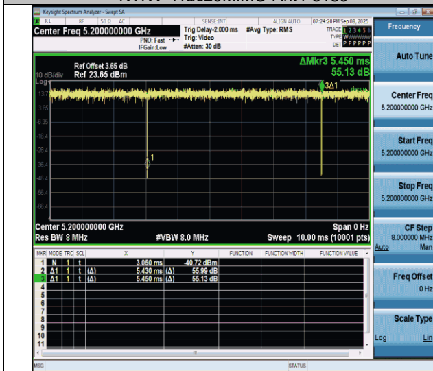
NTNV-11ac20MIMO-Ant4-5200
