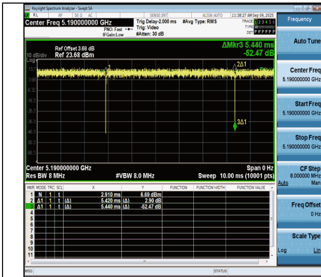
NTNV-11ac40MIMO-Ant4-5190
