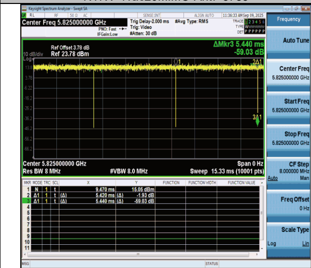
NTNV-11ac20MIMO-Ant7-5825
