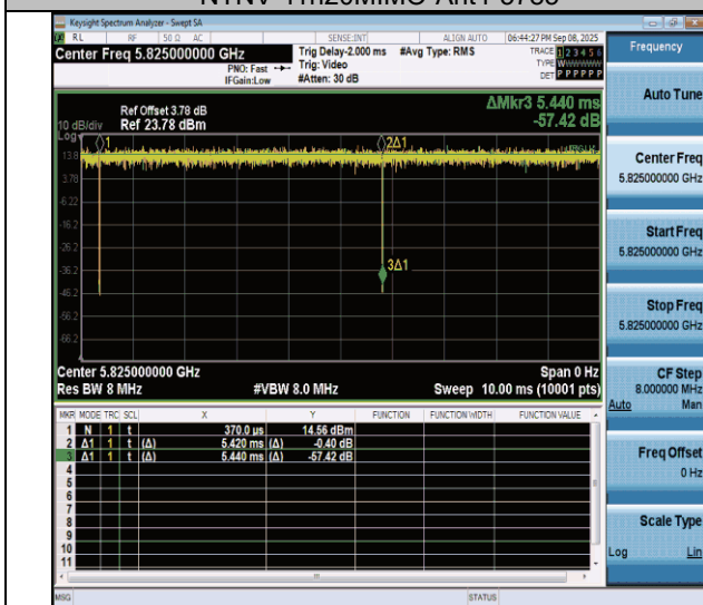
NTNV-11n20MIMO-Ant4-5825
