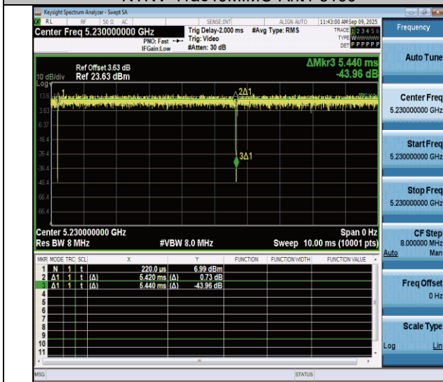
NTNV-11ac40MIMO-Ant4-5230
