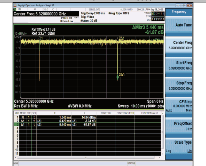
NTNV-11n20MIMO-Ant7-5320
