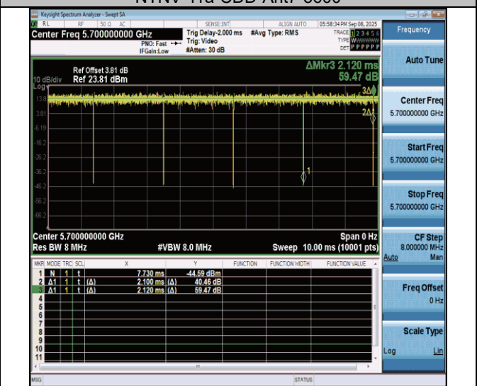
NTVN-11a-CDD-Ant7-5700
