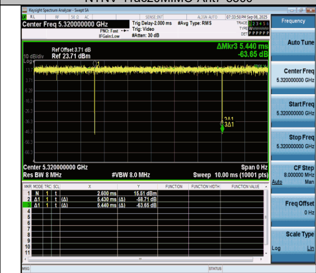
NTNV-11ac20MIMO-Ant7-5320
