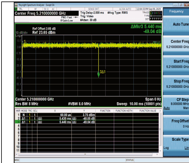
NTNV-11ac80MIMO-Ant4-5210
