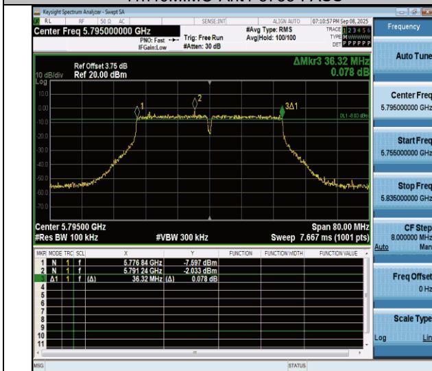
11n40MIMO-Ant4-5795-PASS
