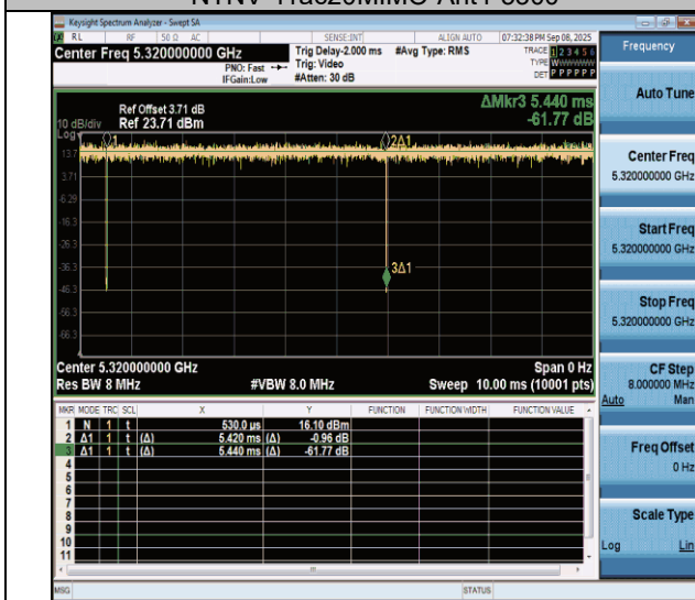
NTNV-11ac20MIMO-Ant4-5320
