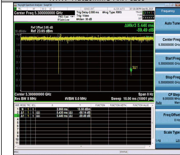
NTNV-11ac20MIMO-Ant4-5300
