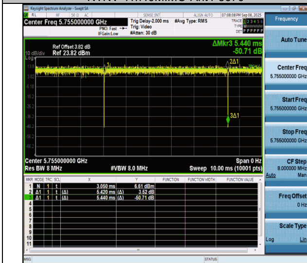
NTNV-11n40MIMO-Ant4-5755
