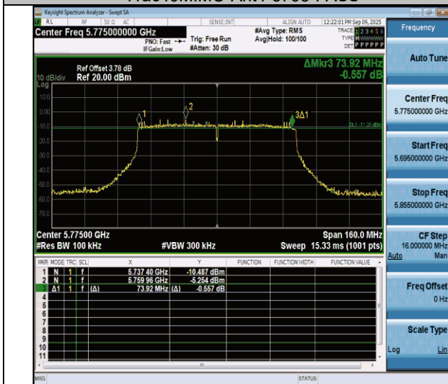
11ac80MIMO-Ant4-5775-PASS
