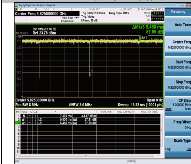
NTNV-11ac20MIMO-Ant4-5825
