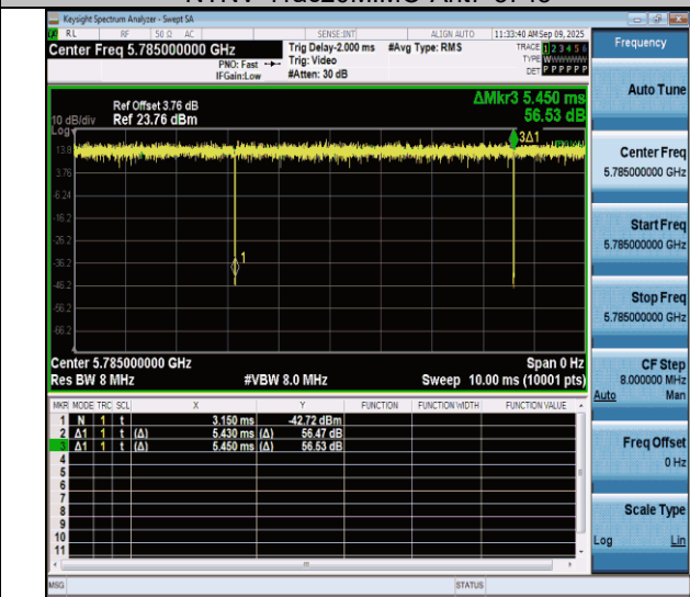
NTNV-11ac20MIMO-Ant7-5785
