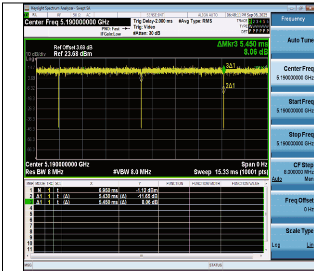
NTNV-11n40MIMO-Ant4-5190
