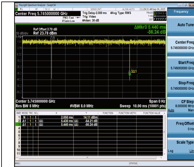
NTNV-11ac20MIMO-Ant4-5745
