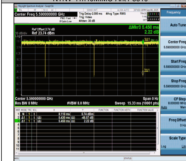
NTNV-11n40MIMO-Ant4-5590
