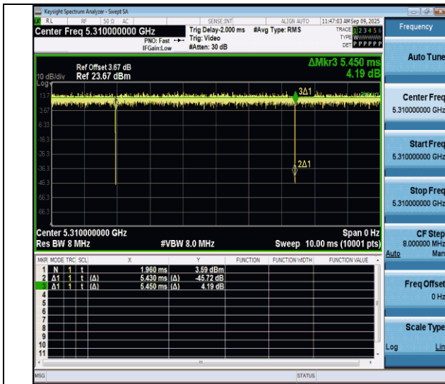
NTNV-11ac40MIMO-Ant4-5310
