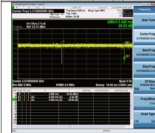
NTNV-11ac160MIMO-Ant4-5570
