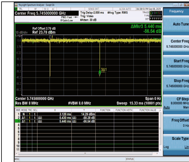
NTNV-11n20MIMO-Ant4-5745
