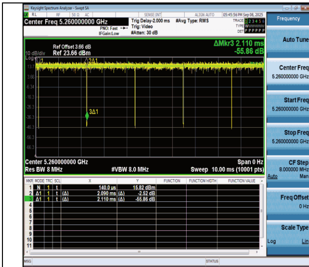
NTVN-11a-CDD-Ant4-5260
