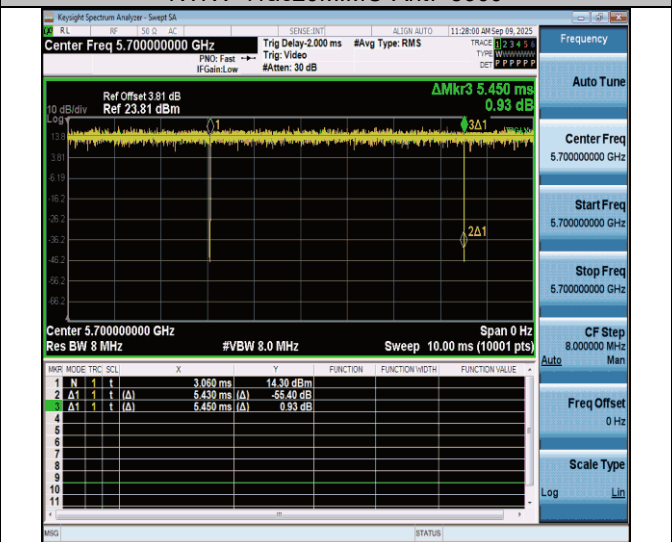
NTNV-11ac20MIMO-Ant7-5700
