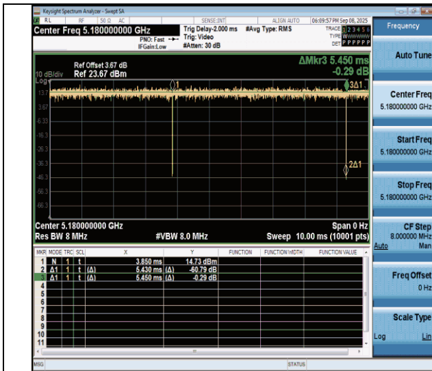
NTNV-11n20MIMO-Ant4-5180
