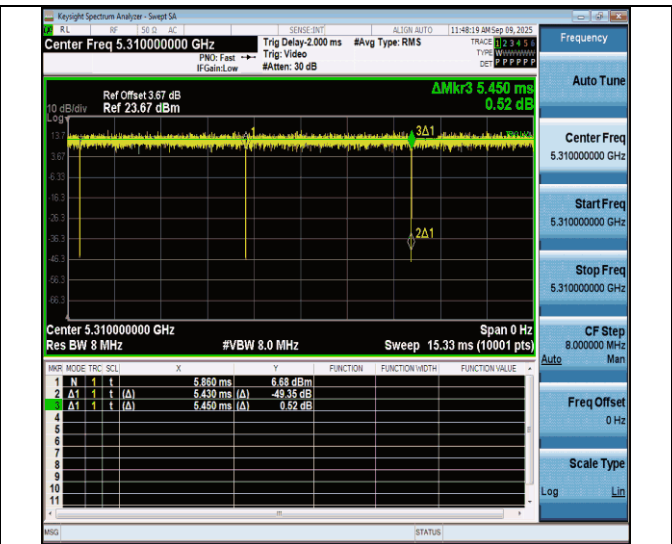
NTNV-11ac40MIMO-Ant7-5310
