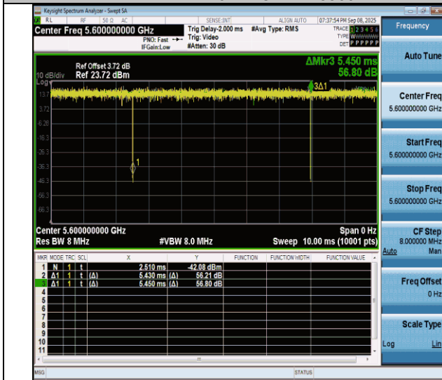
NTNV-11ac20MIMO-Ant4-5600
