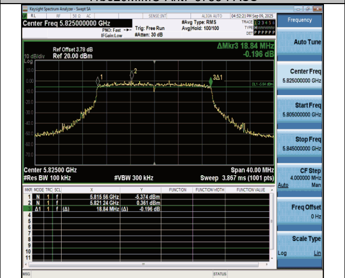
11be20MIMO-Ant7-5825-PASS
