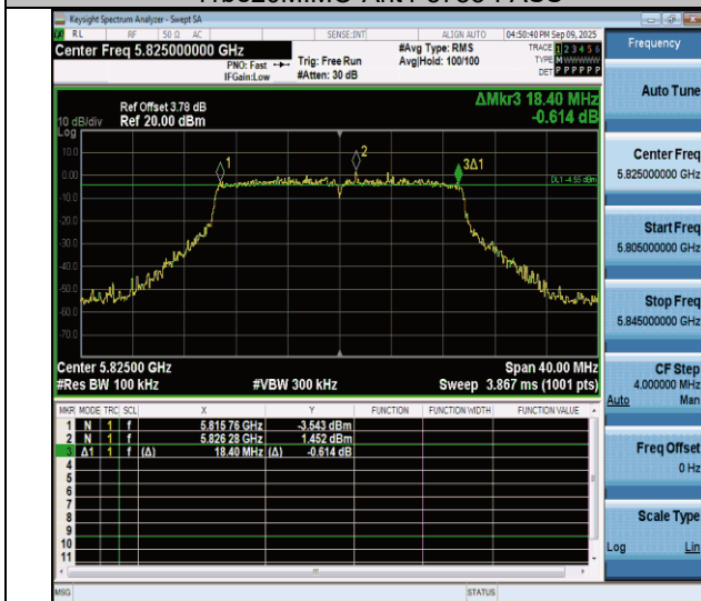
11be20MIMO-Ant4-5825-PASS
