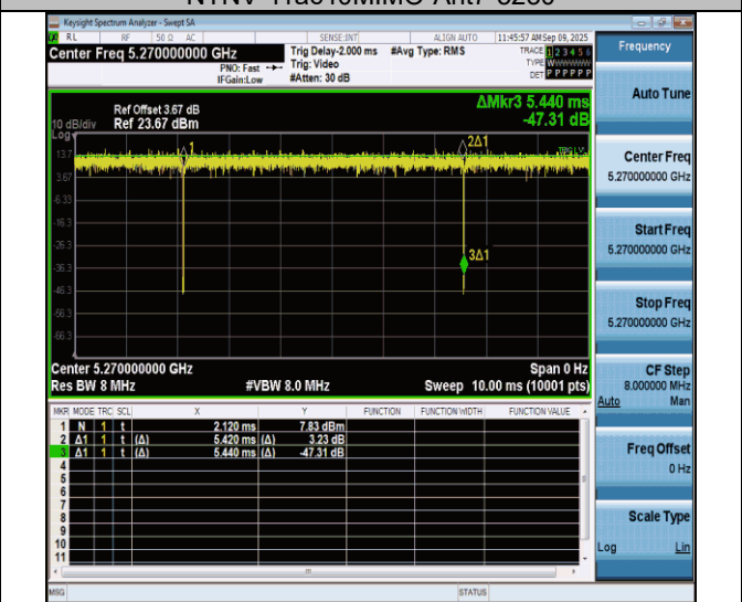
NTNV-11ac40MIMO-Ant7-5270
