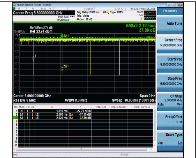
NTVN-11a-CDD-Ant7-5500
