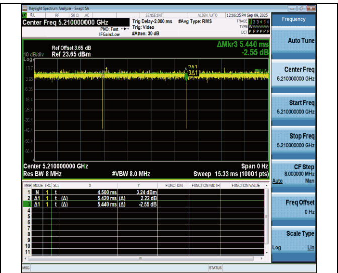
NTNV-11ac80MIMO-Ant7-5210
