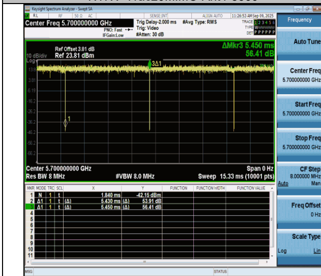
NTNV-11ac20MIMO-Ant4-5700
