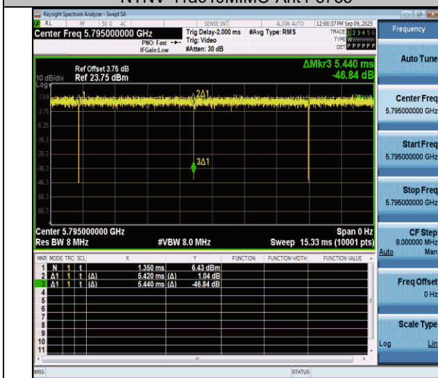
NTNV-11ac40MIMO-Ant4-5795
