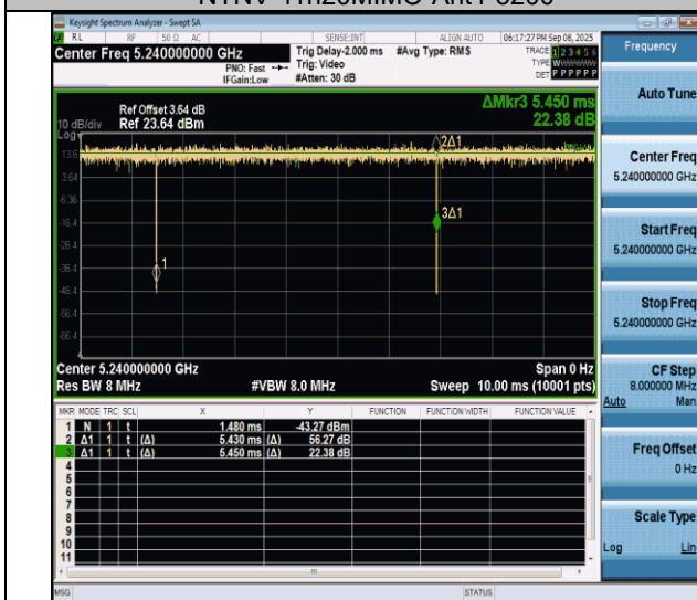
NTNV-11n20MIMO-Ant4-5240
