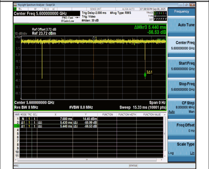
NTNV-11ac20MIMO-Ant7-5600
