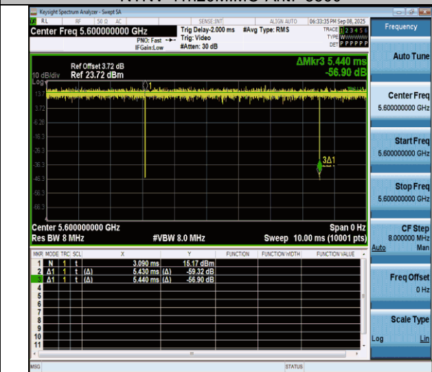
NTNV-11n20MIMO-Ant7-5600
