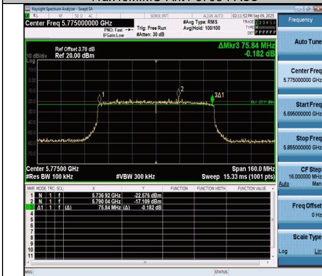
11ax80MIMO-Ant4-5775-PASS
