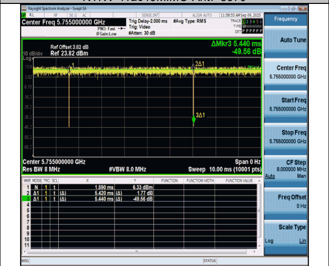
NTNV-11ac40MIMO-Ant7-5755
