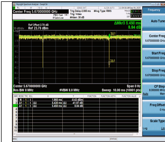
NTNV-11ac40MIMO-Ant4-5670
