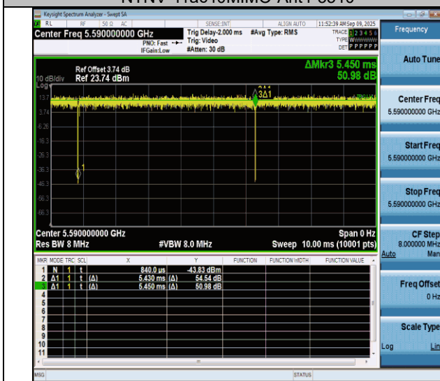
NTNV-11ac40MIMO-Ant4-5590
