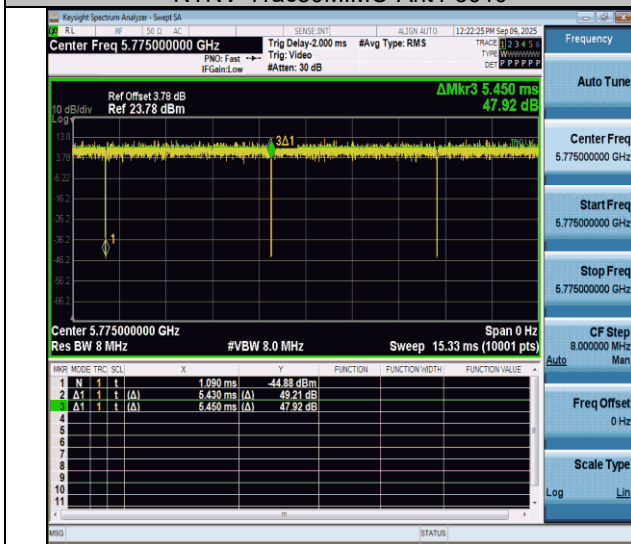
NTNV-11ac80MIMO-Ant4-5775
