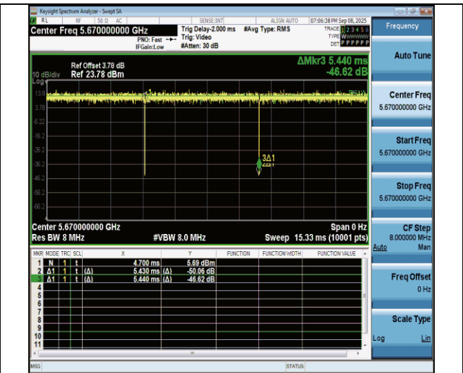
NTNV-11n40MIMO-Ant7-5670
