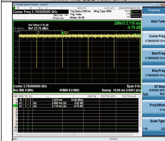
NTNV-11a-CDD-Ant4-5785
