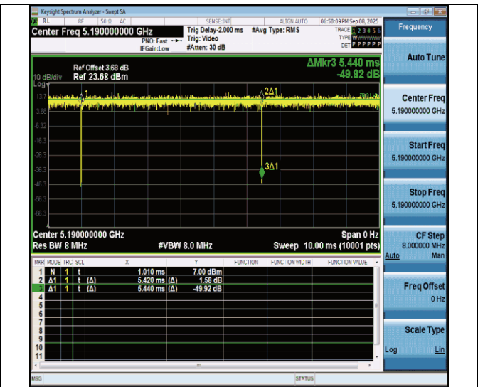
NTNV-11n40MIMO-Ant7-5190
