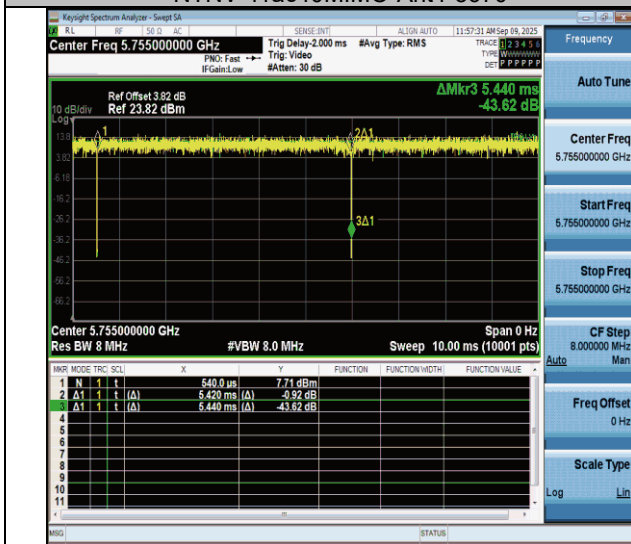
NTNV-11ac40MIMO-Ant4-5755
