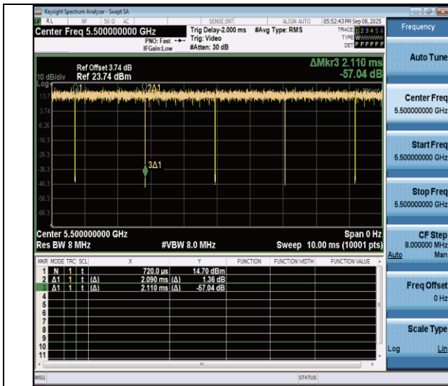
NTVN-11a-CDD-Ant4-5500
