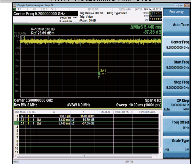
NTNV-11ac20MIMO-Ant7-5200
