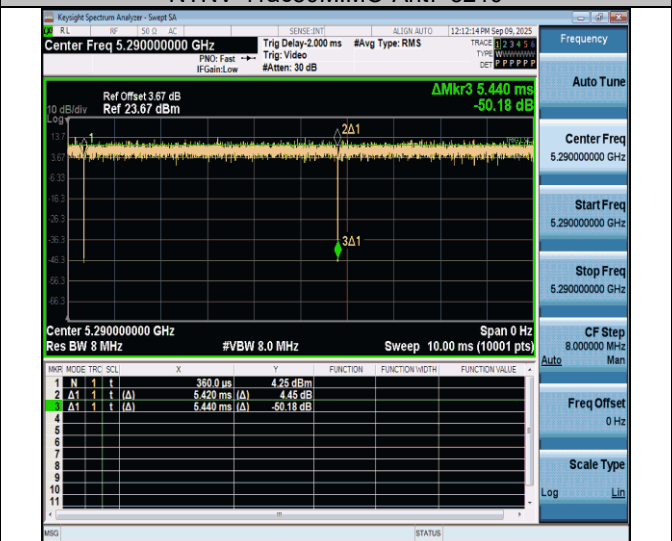
NTNV-11ac80MIMO-Ant7-5290
