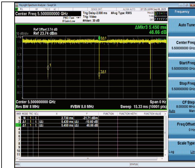
NTNV-11ac20MIMO-Ant4-5500
