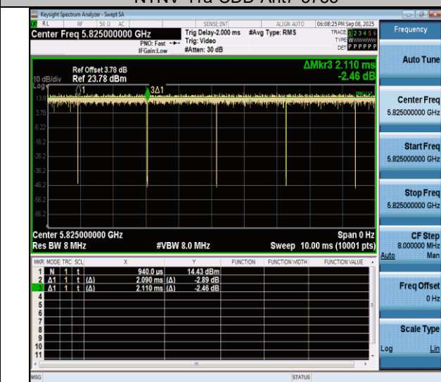
NTNV-11a-CDD-Ant7-5825
