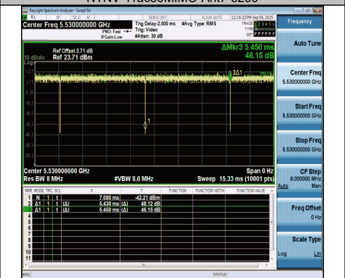
NTNV-11ac80MIMO-Ant7-5530
