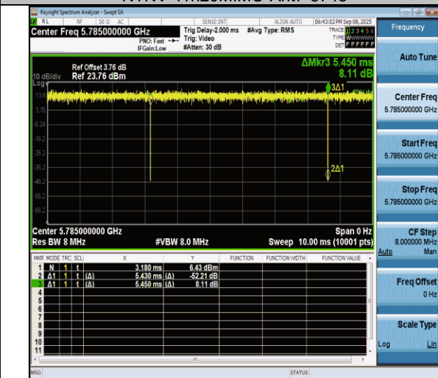
NTNV-11n20MIMO-Ant7-5785
