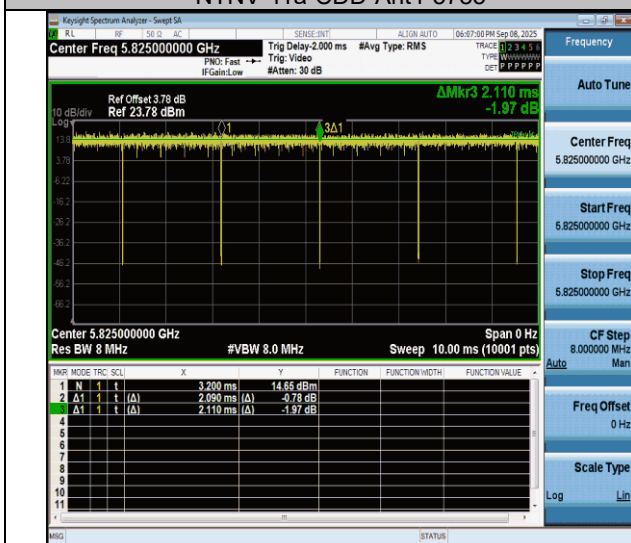
NTNV-11a-CDD-Ant4-5825
