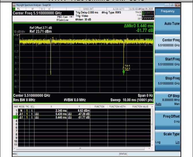
NTNV-11ac40MIMO-Ant7-5510
