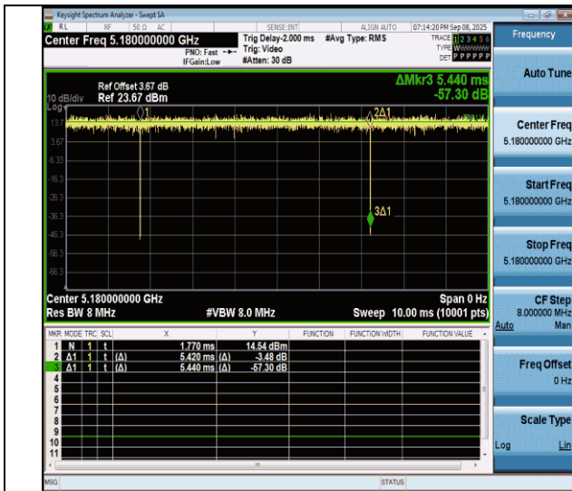
NTNV-11ac20MIMO-Ant4-5180
