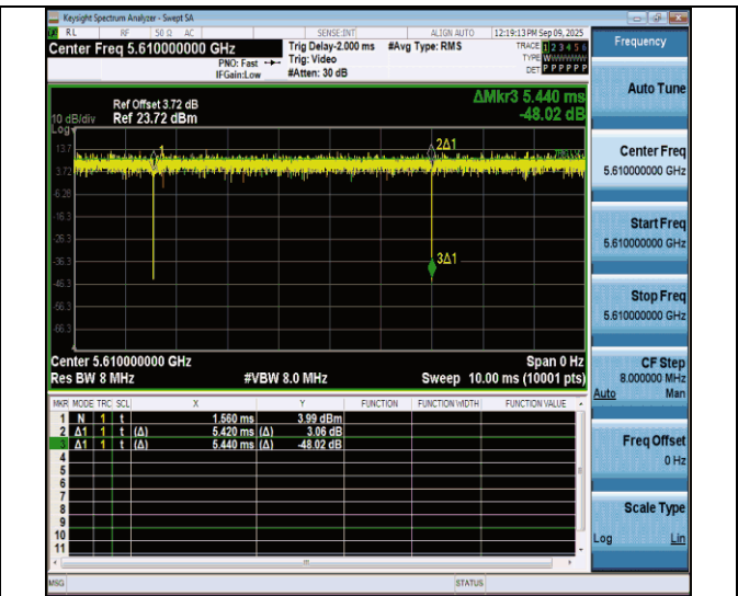
NTNV-11ac80MIMO-Ant7-5610
