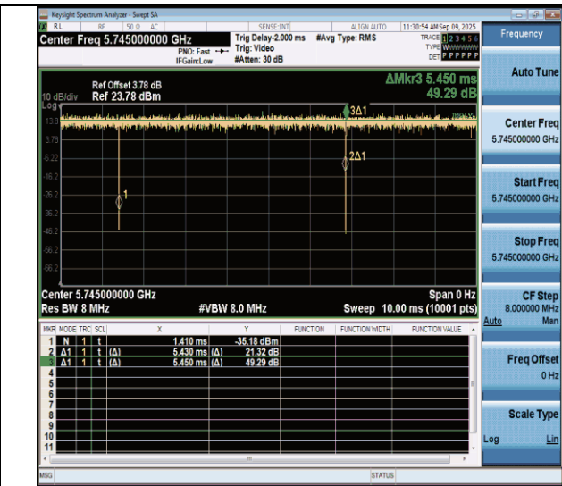
NTNV-11ac20MIMO-Ant7-5745
