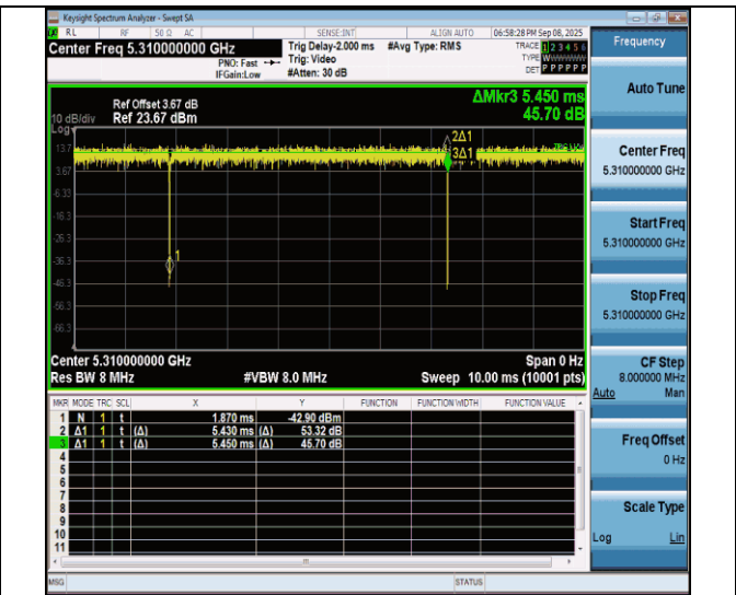
NTNV-11n40MIMO-Ant7-5310
