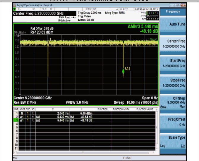
NTNV-11ac40MIMO-Ant7-5230
