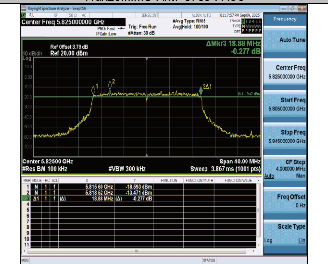
11ax20MIMO-Ant7-5825-PASS
