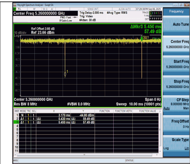
NTNV-11ac20MIMO-Ant7-5260
