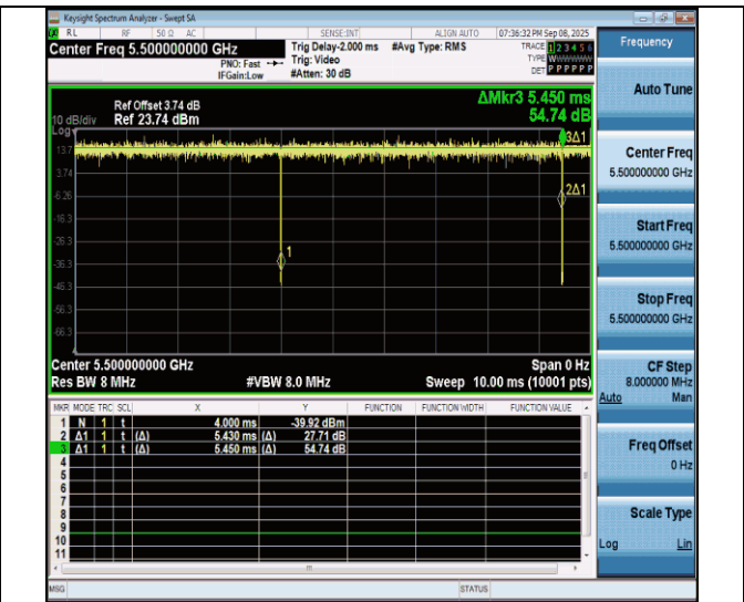
NTNV-11ac20MIMO-Ant7-5500
