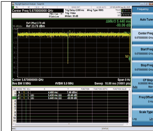
NTNV-11n40MIMO-Ant4-5670
