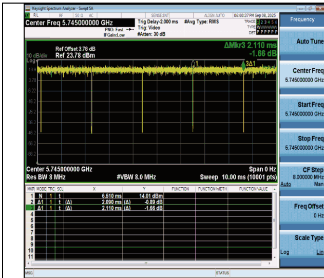
NTNV-11a-CDD-Ant4-5745
