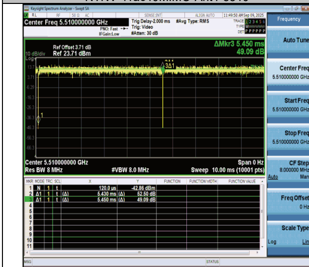
NTNV-11ac40MIMO-Ant4-5510
