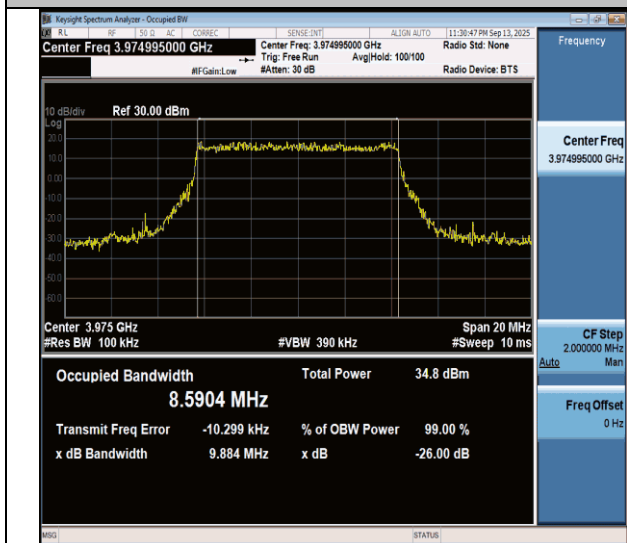
N77(3700-3980)-PC3-30-10-H-DFT-16QAM-Outer_Full-Ant1-PASS
