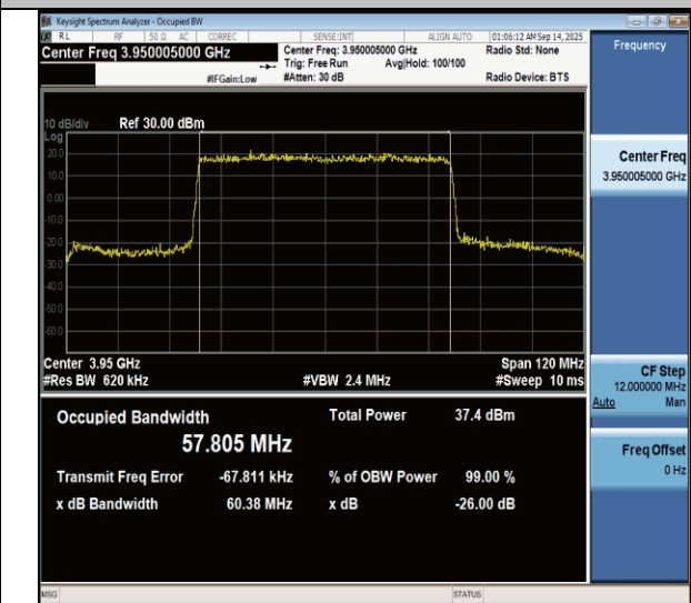
N77(3700-3980)-PC3-30-60-M-CP-64QAM-Outer_Full-Ant1-PASS
