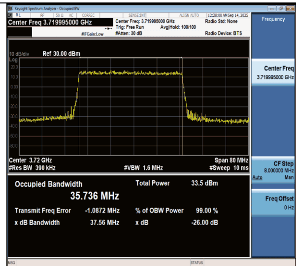
N77(3700-3980)-PC3-30-40-L-DFT-256QAM-Outer_Full-Ant1- PASS
