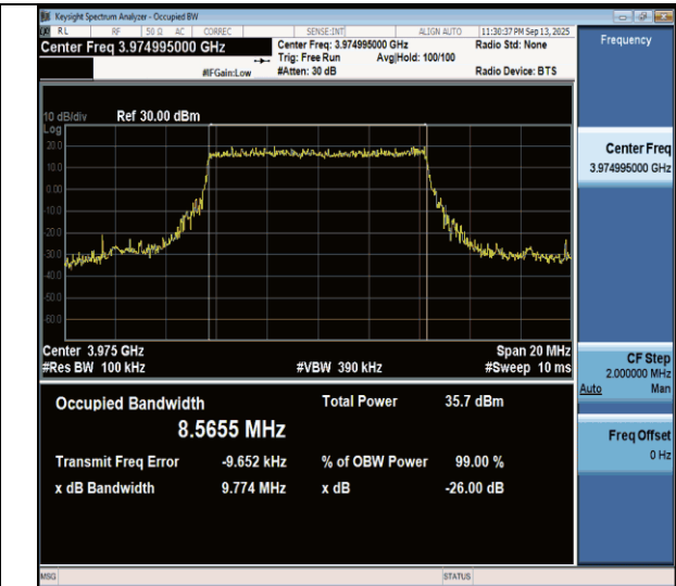
N77(3700-3980)-PC3-30-10-H-DFT-QPSK-Outer_Full-Ant1-PASS
