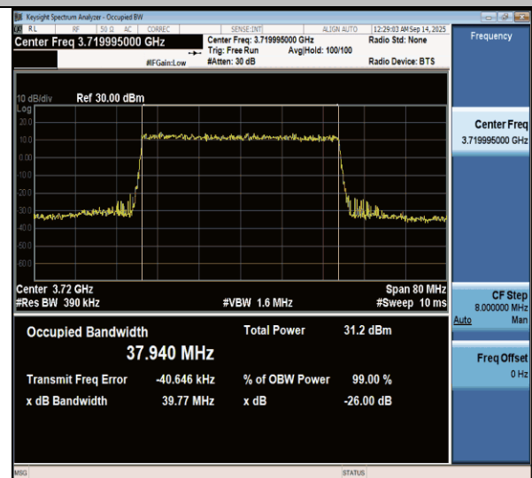
N77(3700-3980)-PC3-30-40-L-CP-256QAM-Outer_Full-Ant1- PASS
