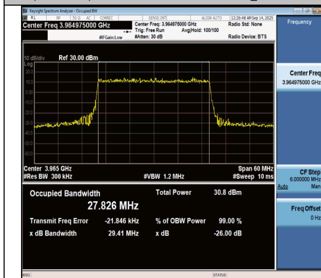
N77(3700-3980)-PC3-30-30-H-CP-256QAM-Outer_Full-Ant1-PASS
