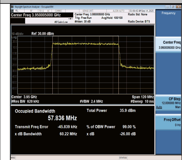
N77(3700-3980)-PC3-30-60-H-DFT-16QAM-Outer_Full-Ant1-PASS
