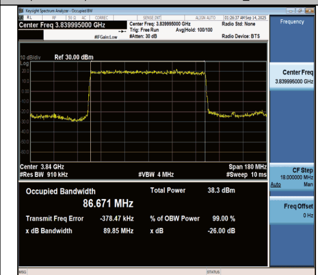
N77(3700-3980)-PC3-30-90-L-CP-64QAM-Outer_Full-Ant1-PASS
