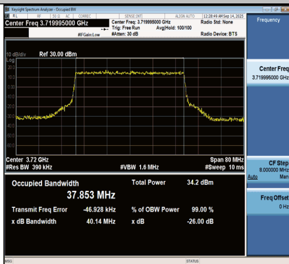
N77(3700-3980)-PC3-30-40-L-CP-QPSK-Outer Full-Ant1-PASS
