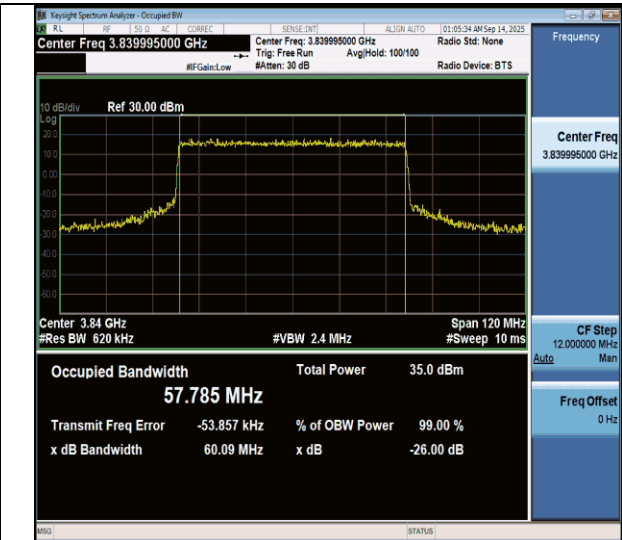
N77(3700-3980)-PC3-30-60-M-CP-64QAM-Outer_Full-Ant1-PASS
