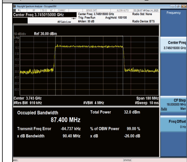
N77(3700-3980)-PC3-30-90-L-CP-256QAM-Outer_Full-Ant1-PASS
