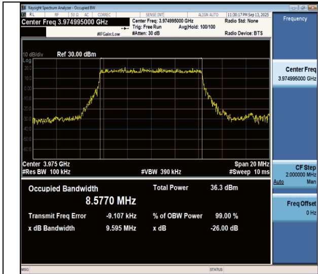
N77(3700-3980)-PC3-30-10-H-DFT-BPSK-Outer_Full-Ant1-PASS
