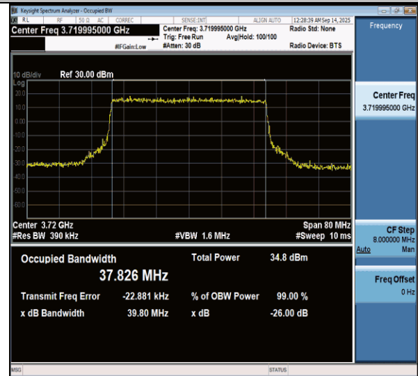
N77(3700-3980)-PC3-30-40-L-CP-16QAM-Outer Full-Ant1-PASS
