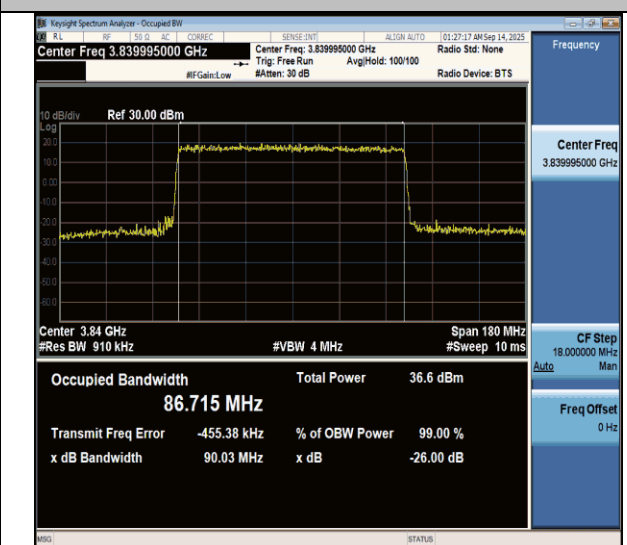
N77(3700-3980)-PC3-30-90-M-DFT-16QAM-Outer_Full-Ant1-PASS
