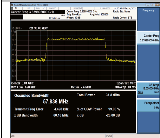
N77(3700-3980)-PC3-30-60-M-CP-256QAM-Outer_Full-Ant1-PASS
