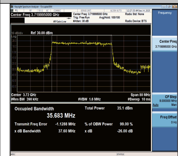
N77(3700-3980)-PC3-30-40-L-DFT-16QAM-Outer_Full-Ant1-PASS
