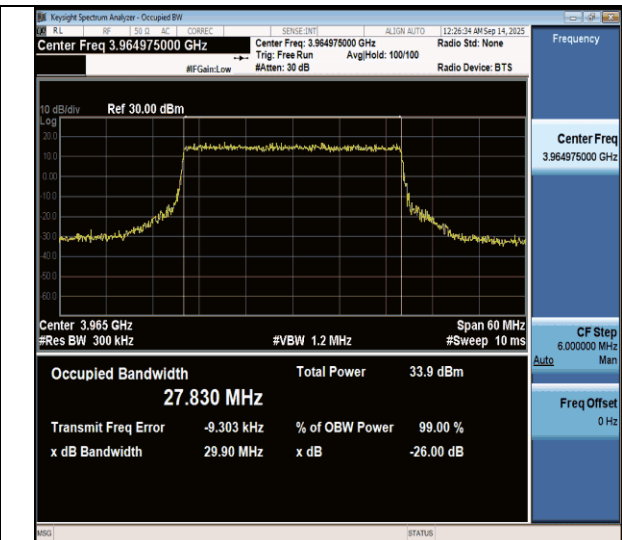
N77(3700-3980)-PC3-30-30-H-CP-64QAM-Outer_Full-Ant1-PASS
