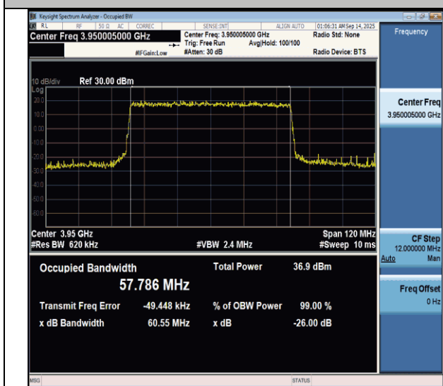
N77(3700-3980)-PC3-30-60-M-CP-256QAM-Outer_Full-Ant1-PASS
