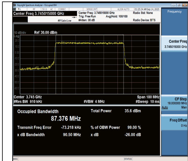
N77(3700-3980)-PC3-30-90-L-CP-16QAM-Outer_Full-Ant1-PASS
