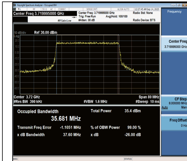
N77(3700-3980)-PC3-30-40-L-DFT-64QAM-Outer_Full-Ant1- PASS
