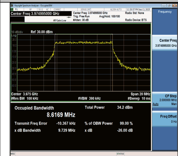
N77(3700-3980)-PC3-30-10-H-DFT-64QAM-Outer_Full-Ant1-PASS
