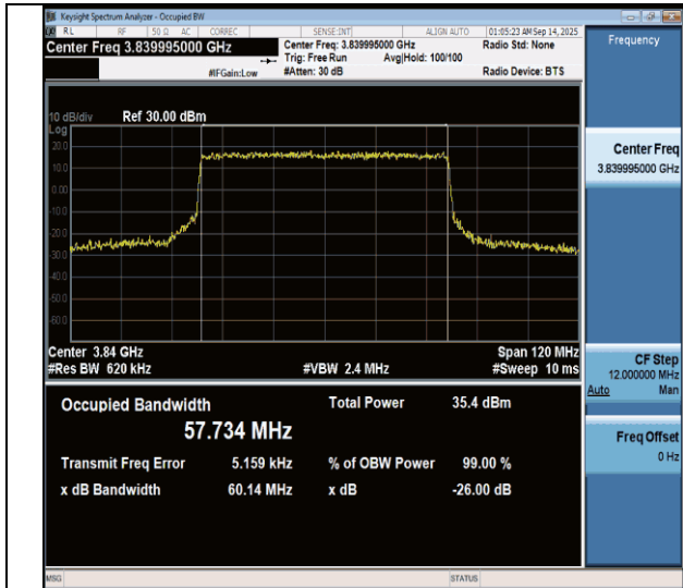
N77(3700-3980)-PC3-30-60-M-CP-16QAM-Outer_Full-Ant1-PASS
