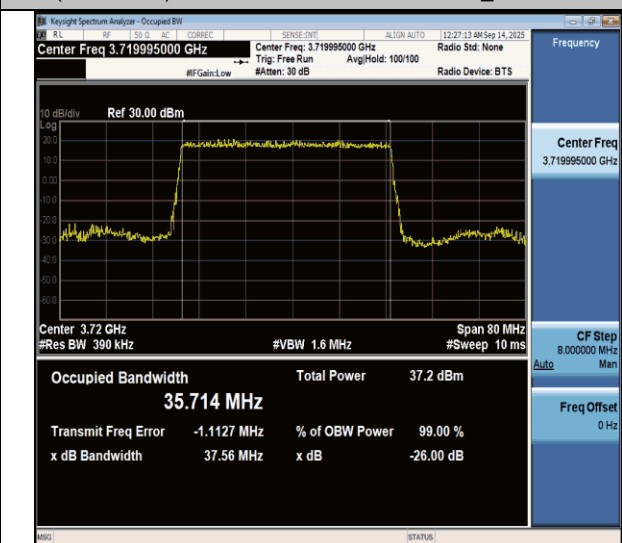
N77(3700-3980)-PC3-30-30-H-CP-64QAM-Outer_Full-Ant1-PASS
