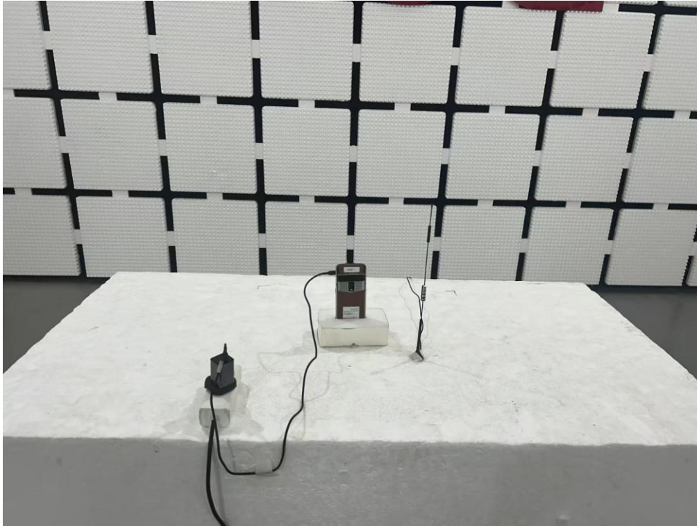
Field Strength of Spurious Radiation – 1000MHz to 18000MHz
