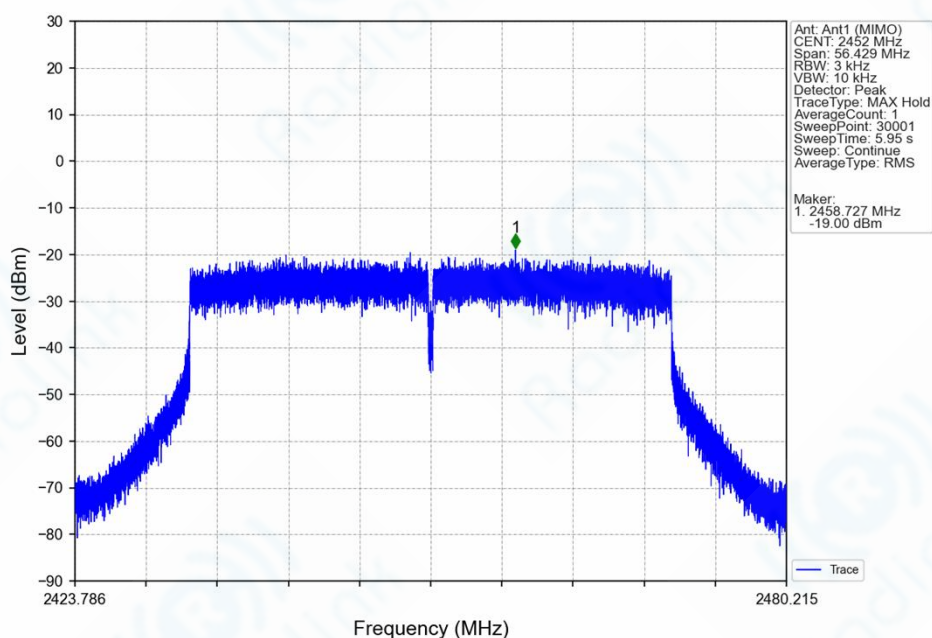
802.11ax(HEW40)_HCH_2452MHz_SU_/_Ant1 (MIMO)_NTNV
