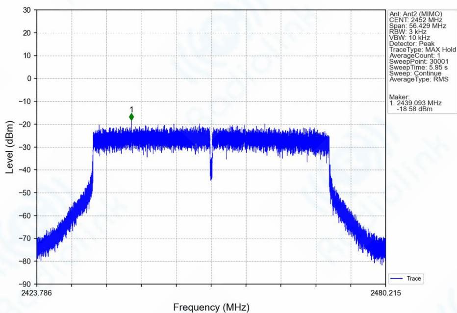
802.11ax(HEW40)_HCH_2452MHz_SU_/_MIMO_NTNV
