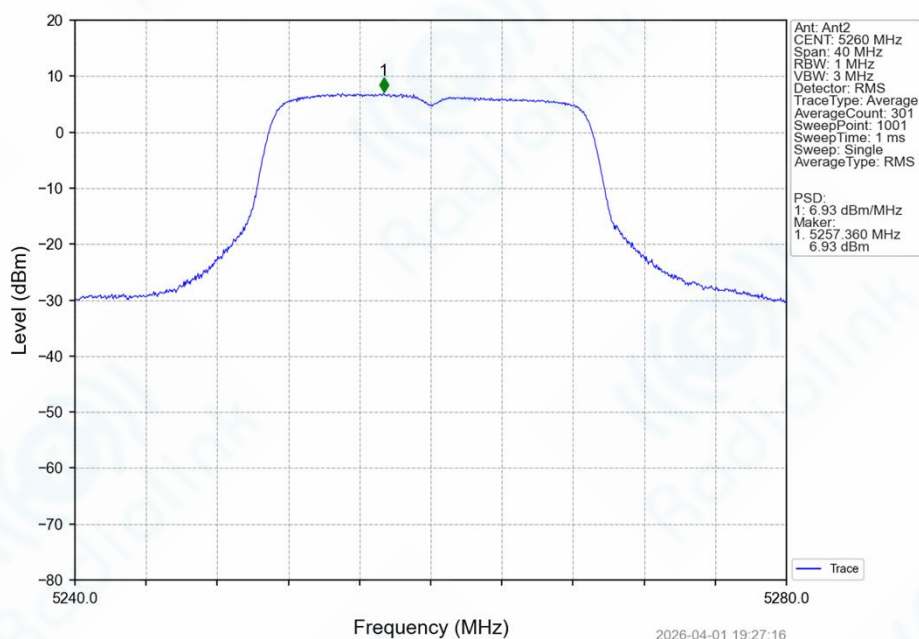
802.11n(HT20)_LCH_5260MHz_MIMO_NTNV
