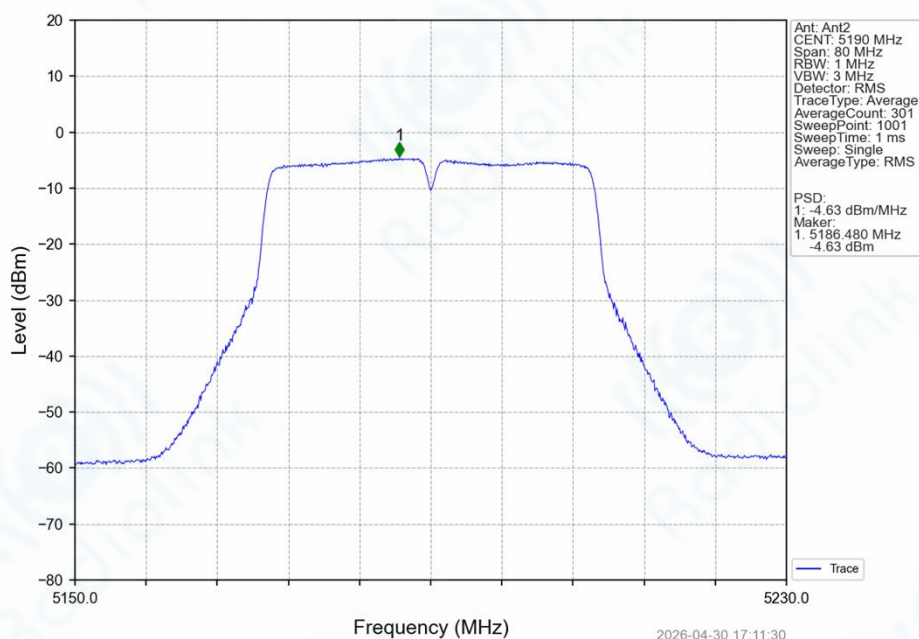
802.11ac(VHT40)_LCH_5190MHz_MIMO_NTNV
