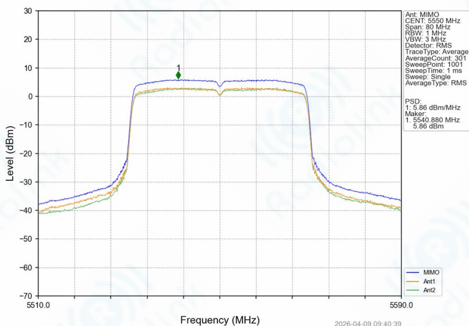
802.11ax(HEW40)_MCH_5550MHz_SU / MIMO_NTNV
