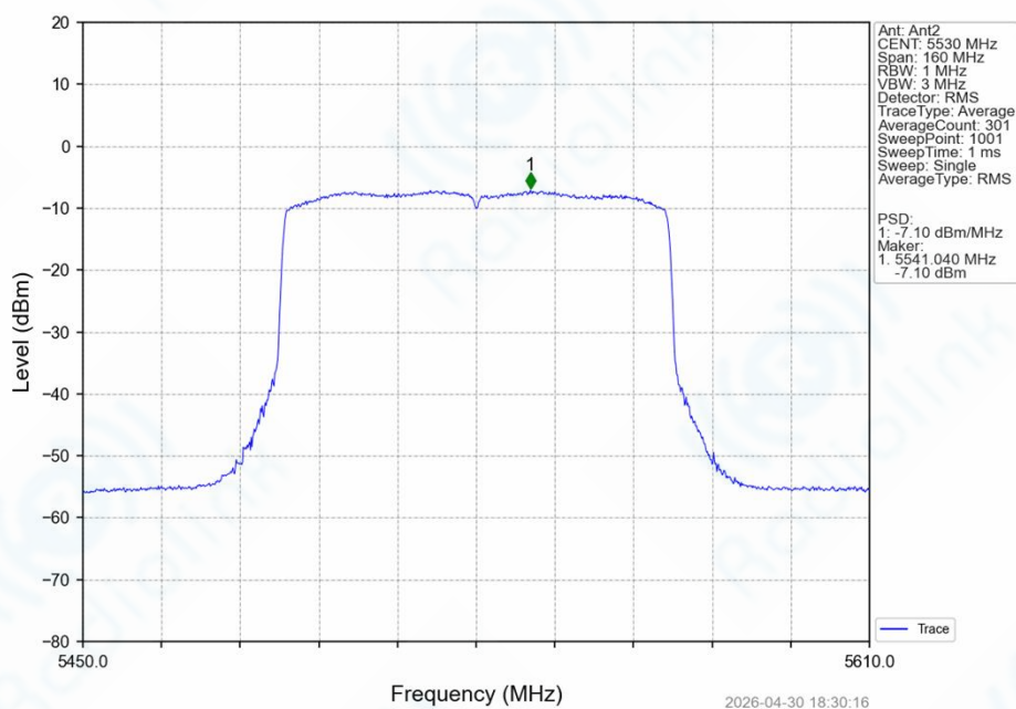
802.11ax(HEW80)_LCH_5530MHz_SU_/_MIMO_NTNV
