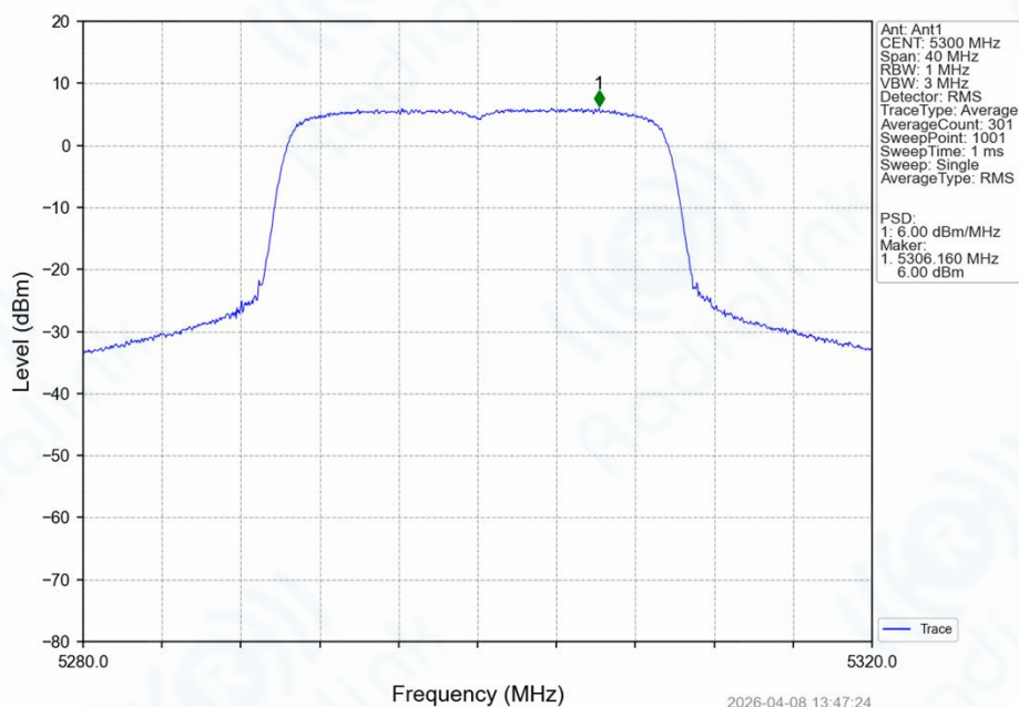
802.11ax(HEW20)_MCH_5300MHz_SU / _Ant1_NTNV
