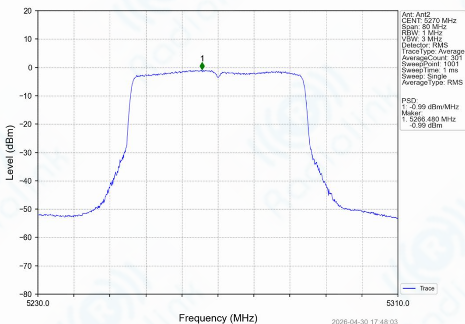
802.11ax(HEW40)_LCH_5270MHz_SU_/_Ant2_NTNV
