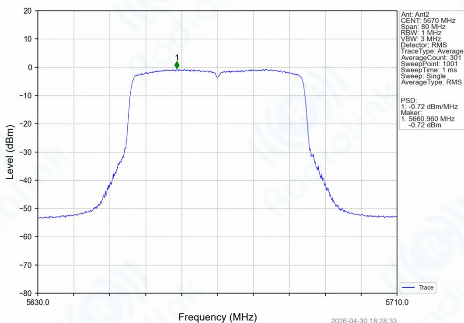
802.11ax(HEW40)_HCH_5670MHz_SU / Ant2_NTNV
