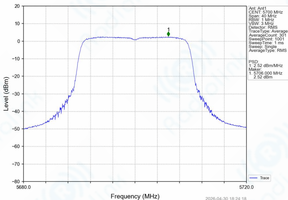
802.11ax(HEW20)_HCH_5700MHz_SU_/_Ant1_NTNV
