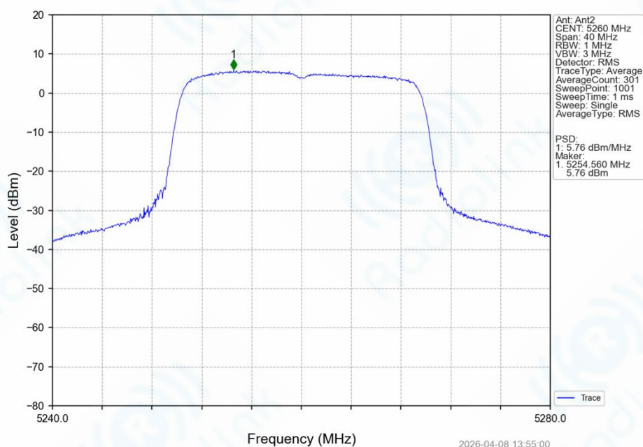
802.11ax(HEW20)_LCH_5260MHz_SU_ / _Ant2_NTNV
