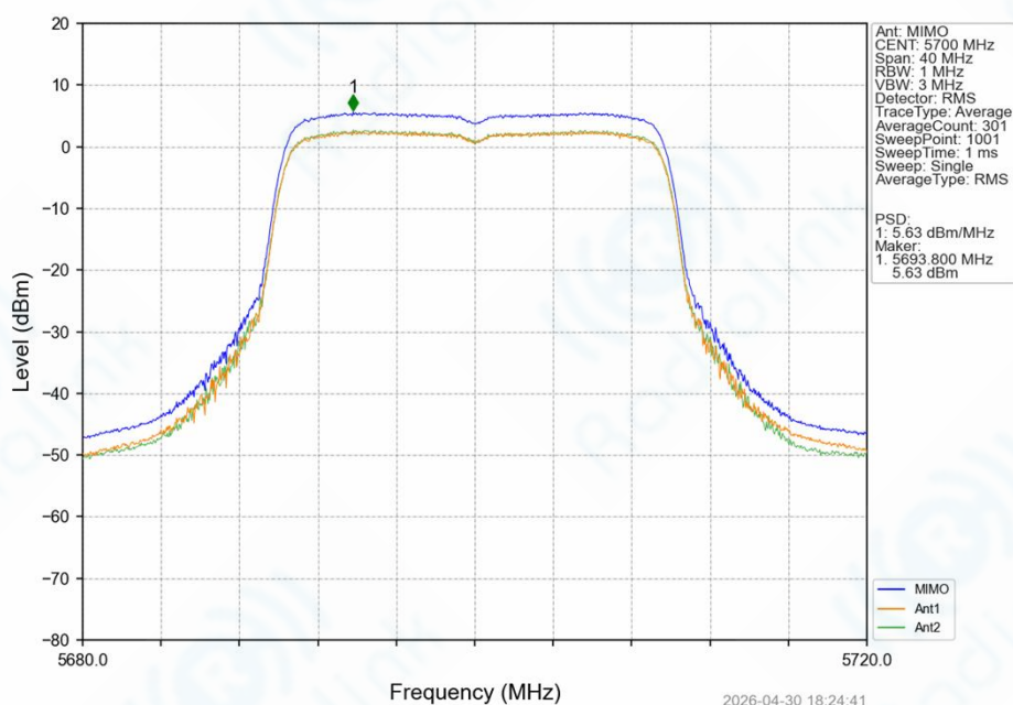
802.11ax(HEW20)_HCH_5700MHz_SU_/_MIMO_NTNV
