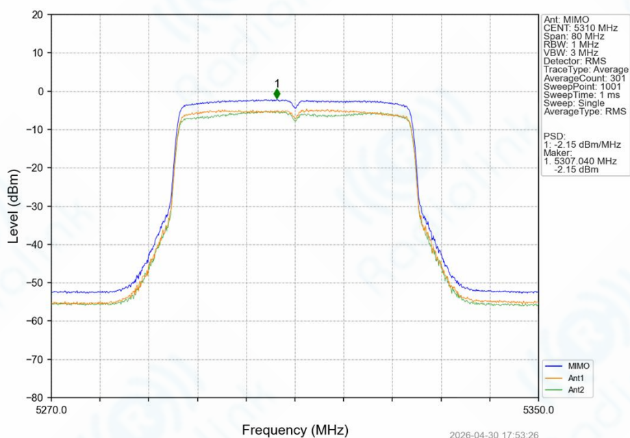
802.11ax(HEW40)_HCH_5310MHz_SU_/_MIMO_NTNV
