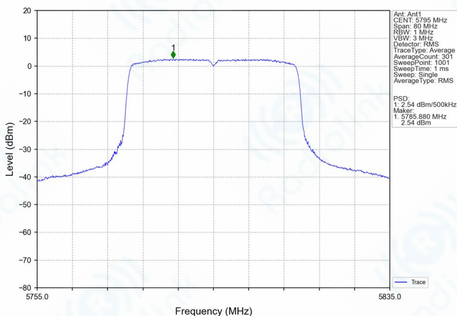
802.11ax(HEW40)_HCH_5795MHz_SU / _Ant1_NTNV
