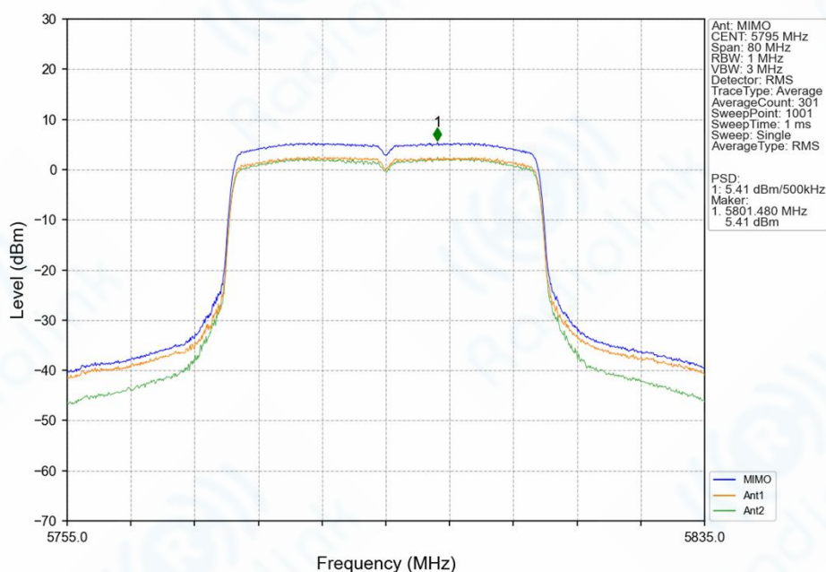
802.11ax(HEW40)_HCH_5795MHz_SU_/_MIMO_NTNV
