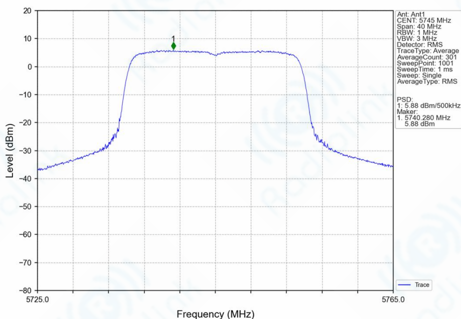
802.11ax(HEW20)_LCH_5745MHz_SU / Ant1_NTNV
