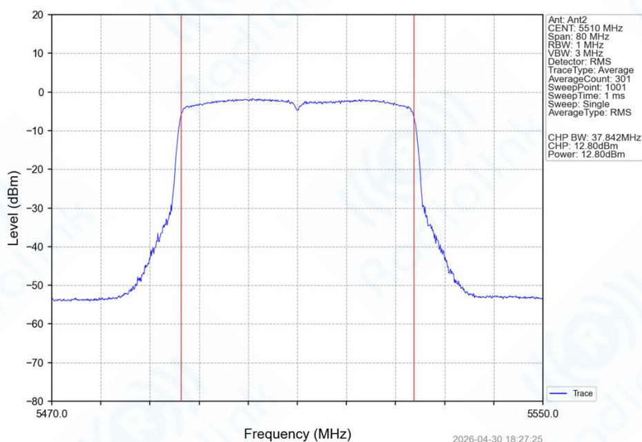
802.11ax(HEW40)_LCH_5510MHz_SU_ / _Ant2_NTNV
