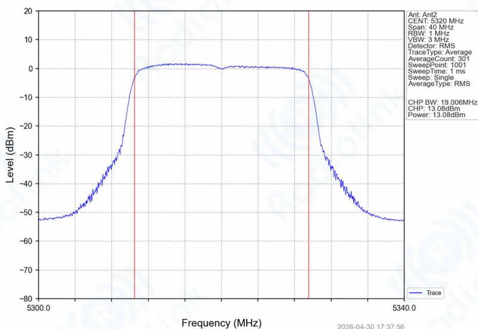
802.11ax(HEW20)_HCH_5320MHz_SU_ / Ant2_NTNV
