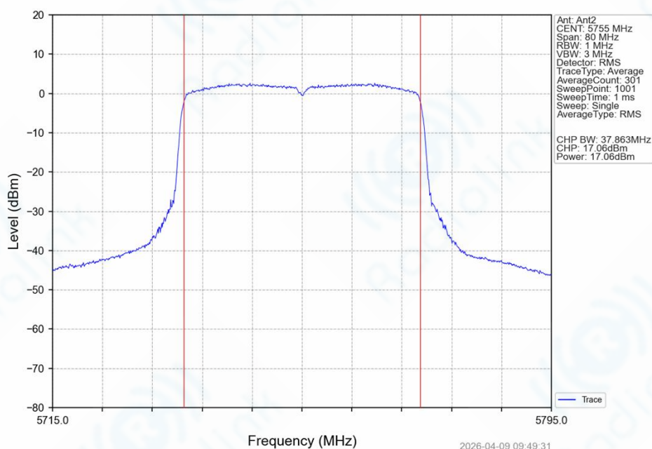
802.11ax(HEW40)_LCH_5755MHz_SU_ / _Ant2_NTNV
