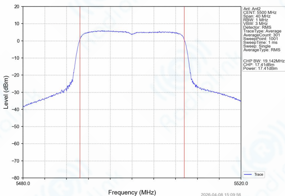
802.11ax(HEW20)_LCH_5500MHz_SU_/_Ant2_NTNV
