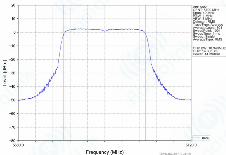
802.11ax(HEW20)_HCH_5700MHz_SU_ / _Ant2_NTNV
