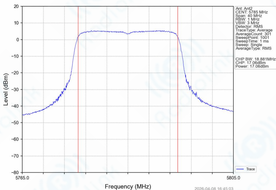
802.11ax(HEW20)_MCH_5785MHz_SU / Ant2 NTN
