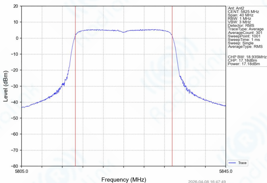
802.11ax(HEW20)_HCH_5825MHz_SU_/_Ant2_NTNV
