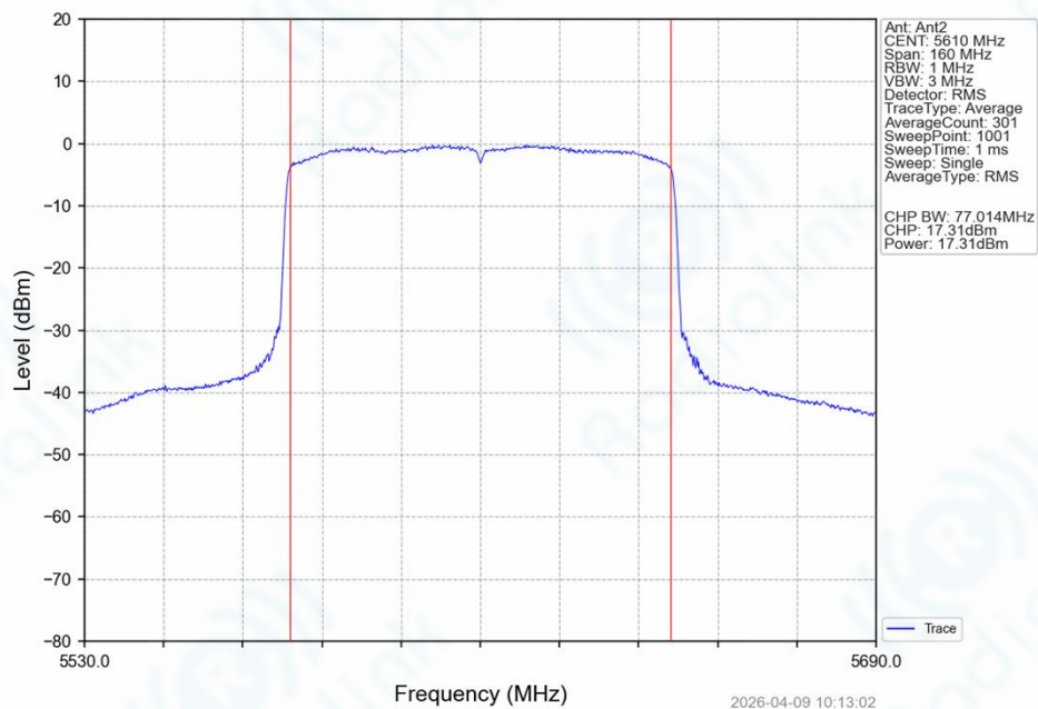
802.11ax(HEW80)_HCH_5610MHz_SU_ / _Ant2_NTNV
