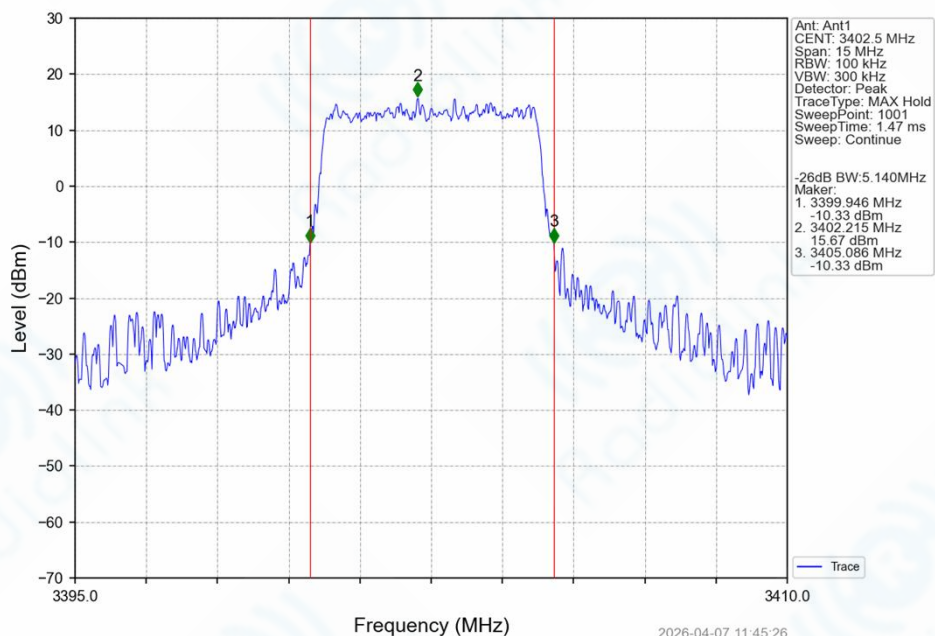
Band42_5MHz_16QAM_LCH_3402.5MHz_RB_25_0_NTNV
