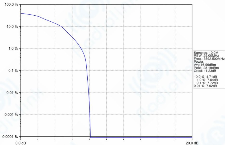
Band42_15MHz_16QAM_HCH_3592.5MHz_RB_75_0_NTNV
