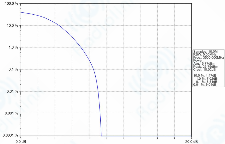
Band42_5MHz_64QAM_MCH_3500MHz_RB_25_0_NTNV
