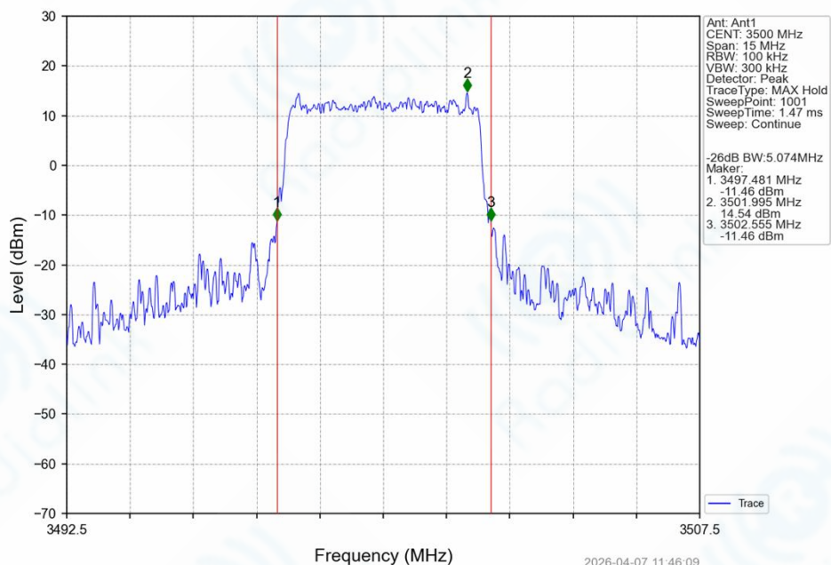
Band42_5MHz_64QAM_MCH_3500MHz_RB_25_0_NTNV
