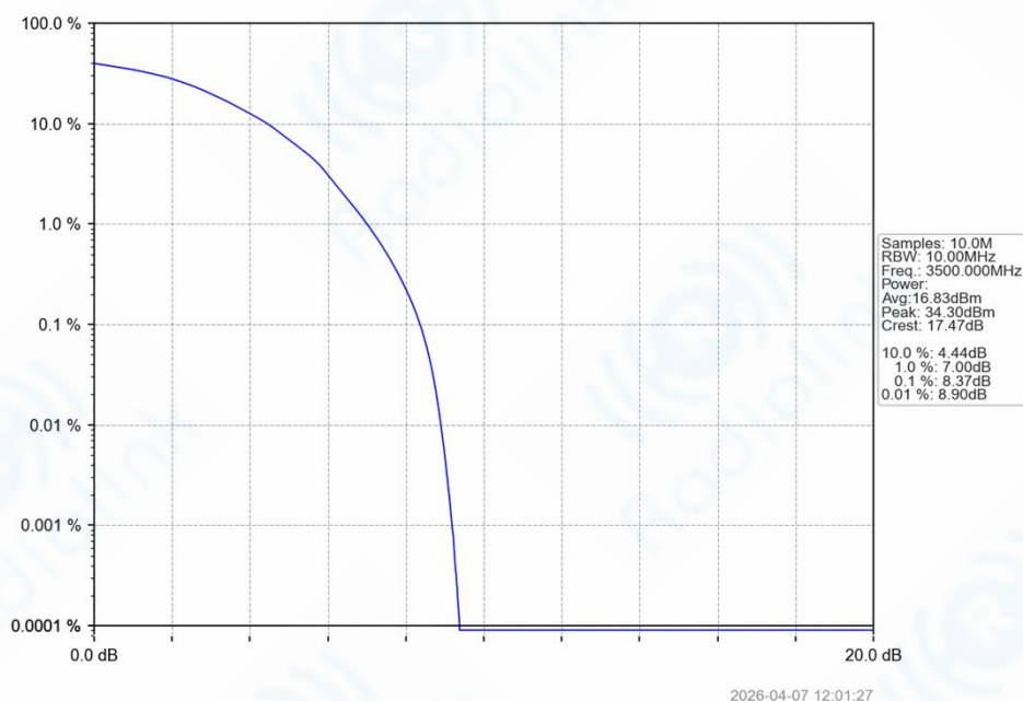
Band42_10MHz_64QAM_MCH_3500MHz_RB_50_0_NTNV
