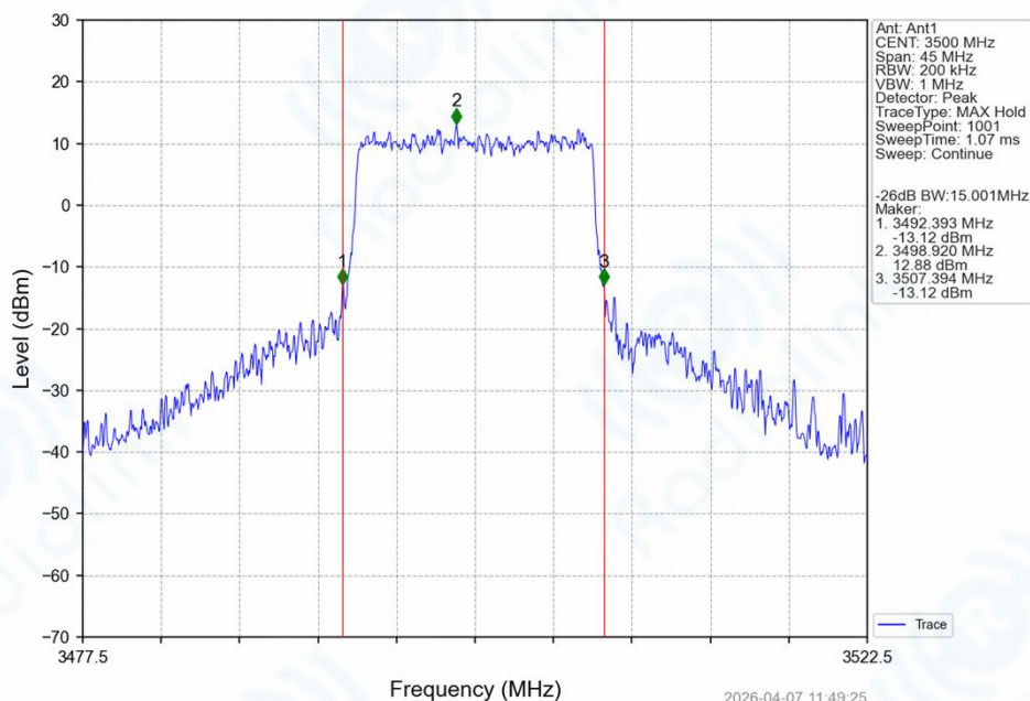
Band42_15MHz_64QAM_MCH_3500MHz_RB_75_0_NTNV
