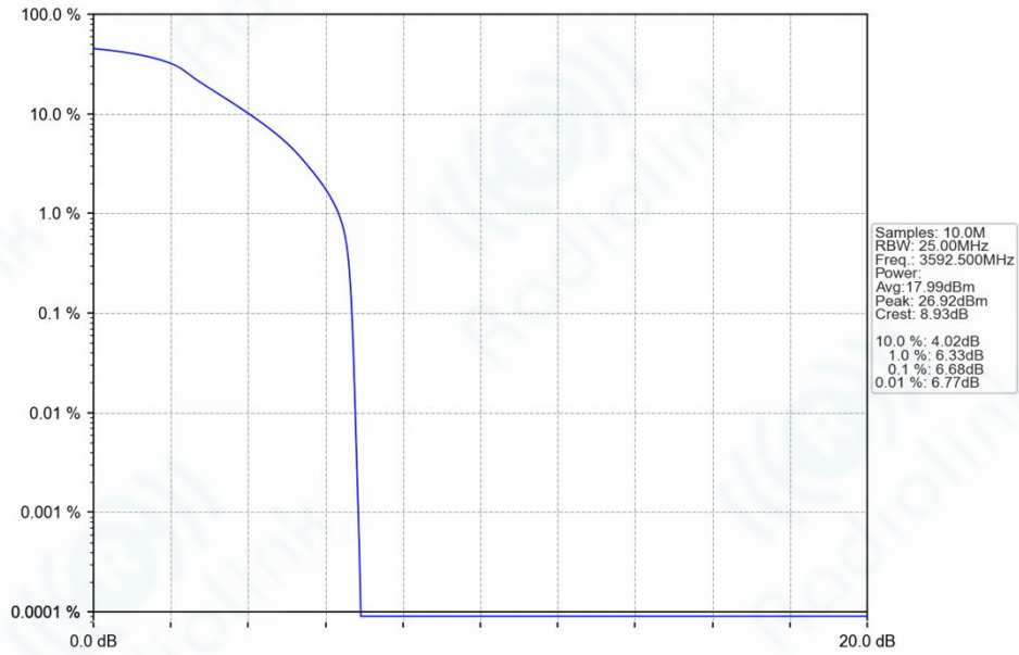
Band42_15MHz_QPSK_HCH_3592.5MHz_RB_75_0_NTNV
