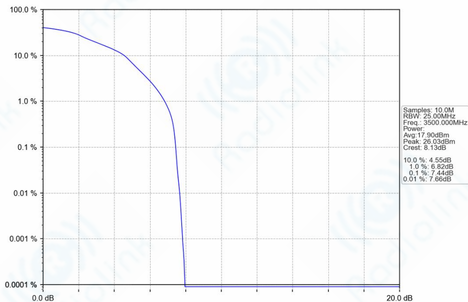
Band42_15MHz_16QAM_MCH_3500MHz_RB_75_0_NTNV
