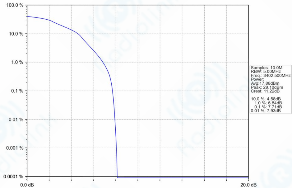
Band42_5MHz_16QAM_LCH_3402.5MHz_RB_25_0_NTNV
