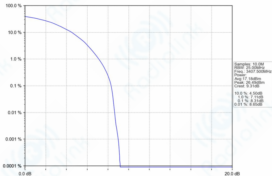
Band42_15MHz_64QAM_LCH_3407.5MHz_RB_75_0_NTNV
