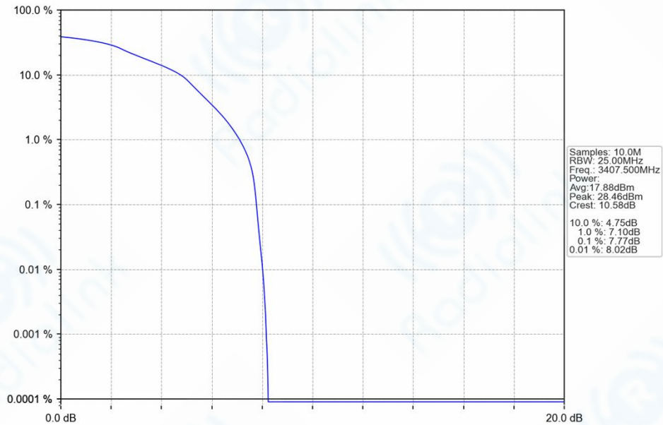
Band42_15MHz_16QAM_LCH_3407.5MHz_RB_75_0_NTNV
