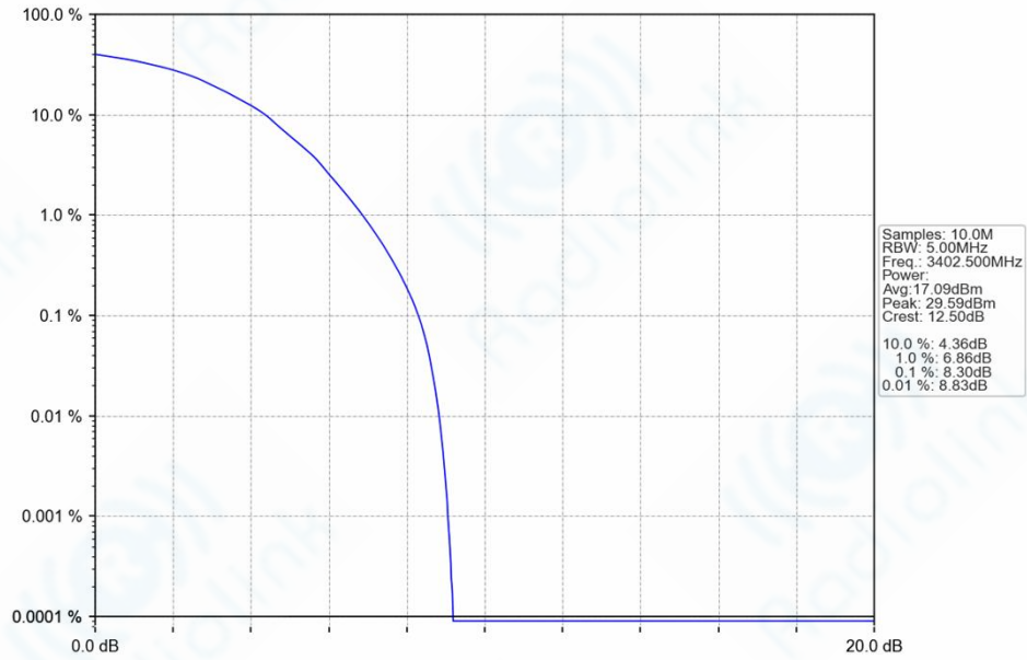
Band42_5MHz_64QAM_LCH_3402.5MHz_RB_25_0_NTNV
