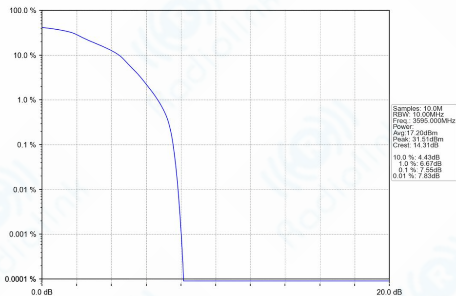
Band42_10MHz_16QAM_HCH_3595MHz_RB_50_0_NTNV
