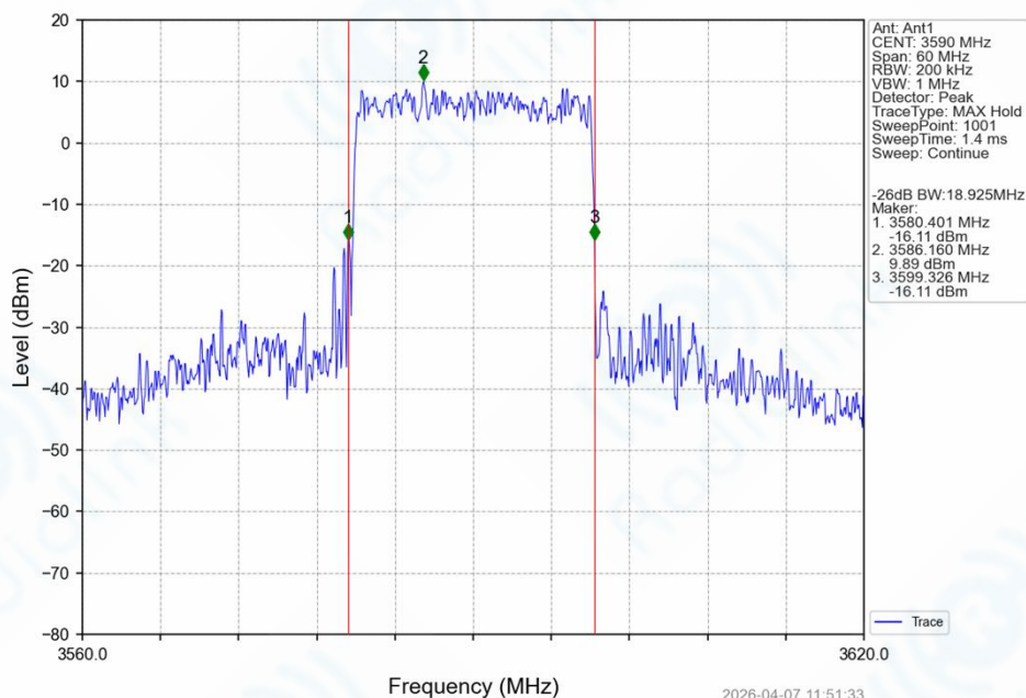
Band42_20MHz_64QAM_HCH_3590MHz_RB_100_0_NTNV
