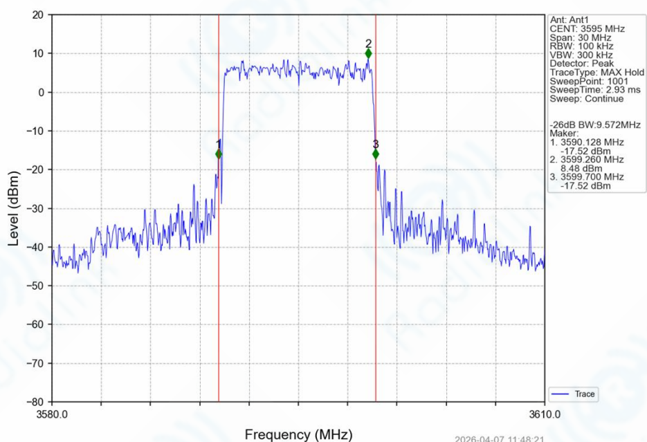
Band42_10MHz_64QAM_HCH_3595MHz_RB_50_0_NTNV
