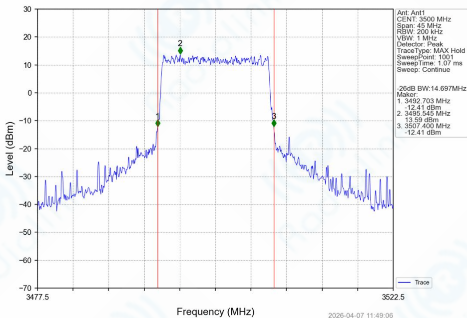
Band42_15MHz_QPSK_MCH_3500MHz_RB_75_0_NTNV
