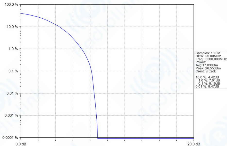
Band42_15MHz_64QAM_MCH_3500MHz_RB_75_0_NTNV
