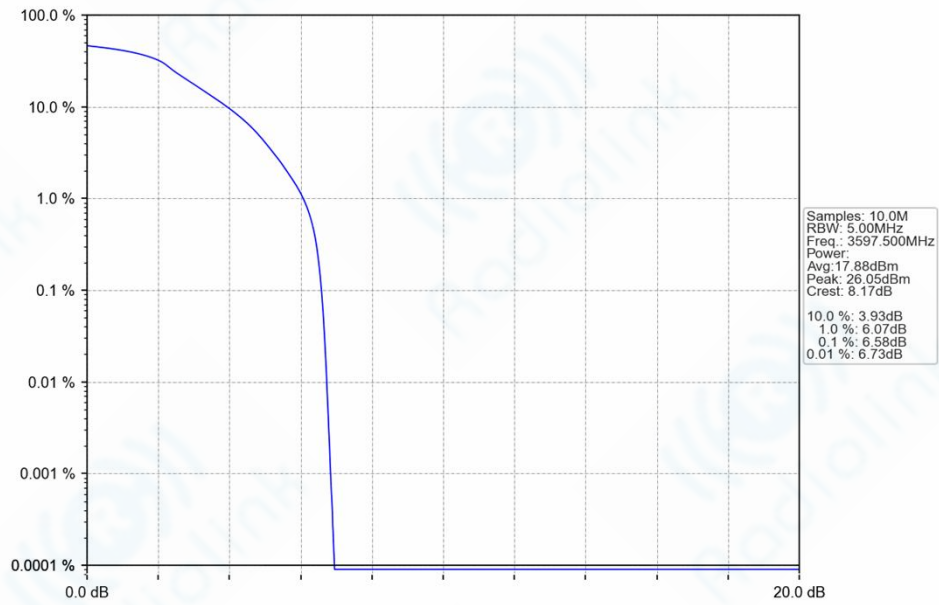
Band42_5MHz_QPSK_HCH_3597.5MHz_RB_25_0_NTNV
