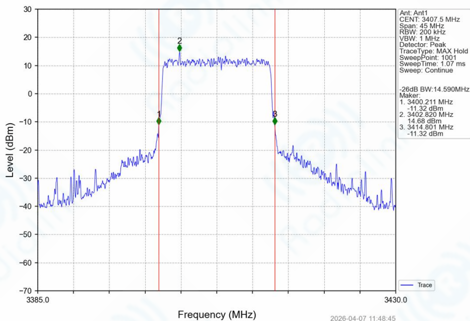
Band42_15MHz_16QAM_LCH_3407.5MHz_RB_75_0_NTNV
