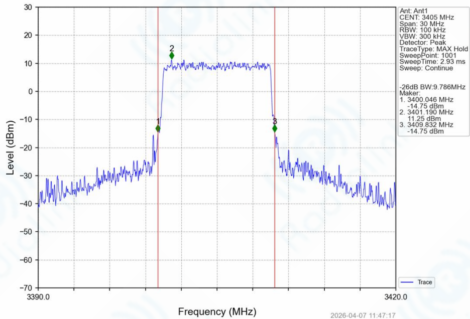
Band42_10MHz_64QAM_LCH_3405MHz_RB_50_0_NTNV
