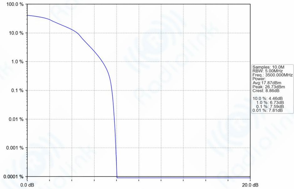
Band42_5MHz_16QAM_MCH_3500MHz_RB_25_0_NTNV
