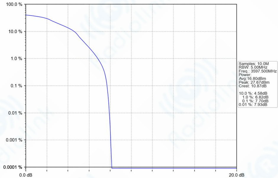
Band42_5MHz_16QAM_HCH_3597.5MHz_RB_25_0_NTNV
