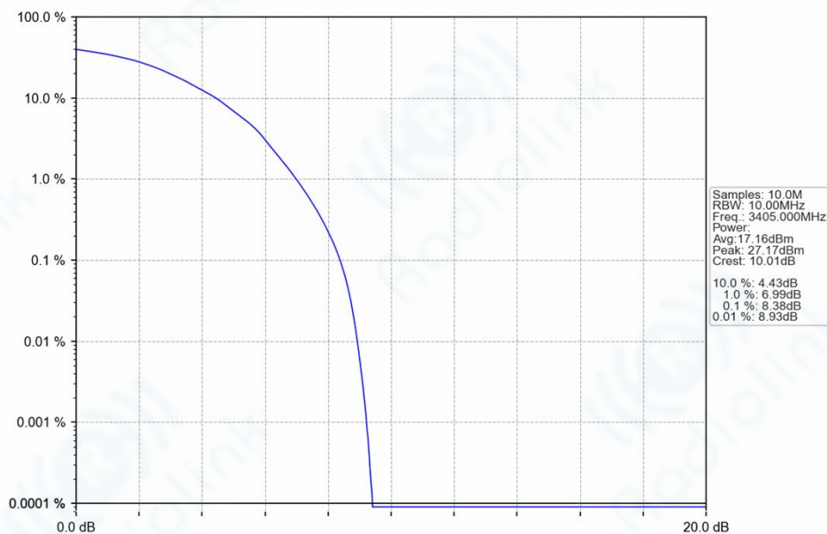
Band42_10MHz_64QAM_LCH_3405MHz_RB_50_0_NTNV
