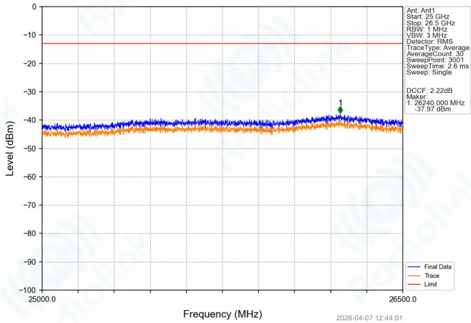
Band42_10MHz_16QAM_HCH_3595MHz_RB_1_0_NTNV
