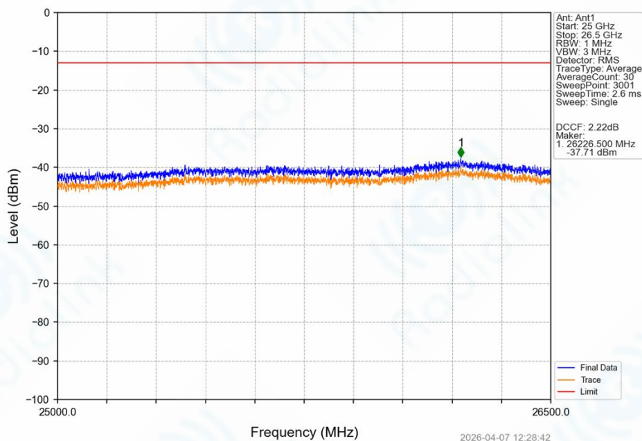
Band42_5MHz_QPSK_MCH_3500MHz_RB_1_0_NTNV
