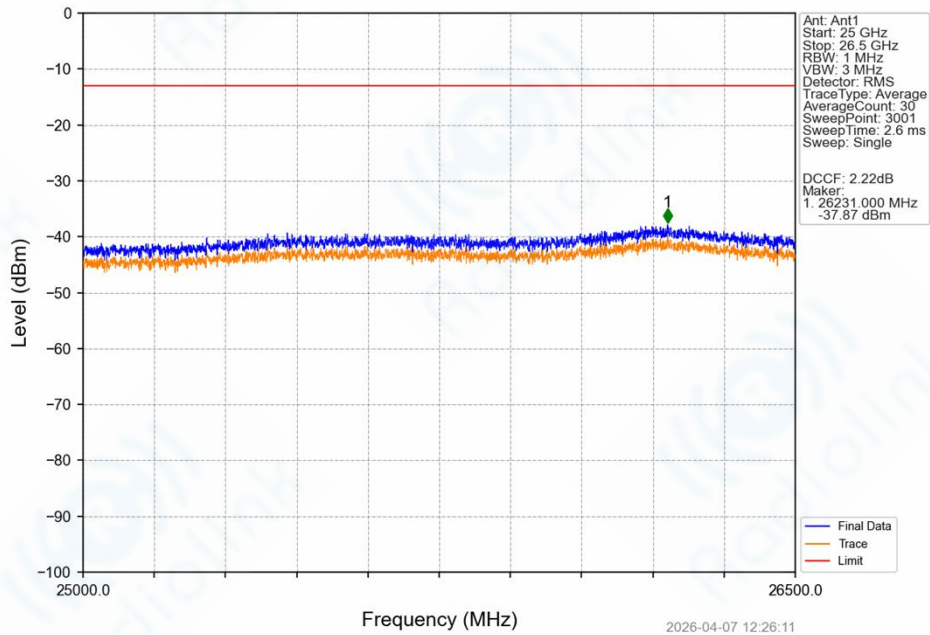
Band42_5MHz_16QAM_LCH_3402.5MHz_RB_25_0_NTNV
