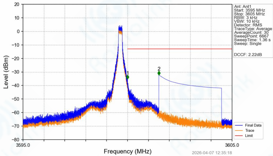
Band42_5MHz_64QAM_HCH_3597.5MHz_RB_1_24_NTNV
