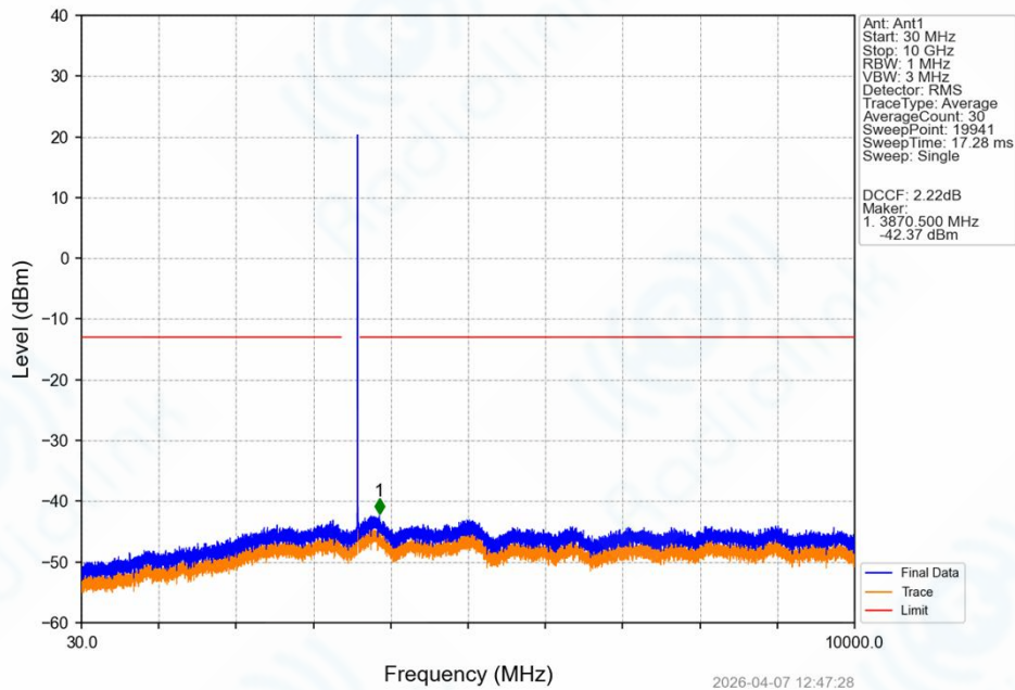
Band42_10MHz_16QAM_HCH_3595MHz_RB_1_0_NTNV
