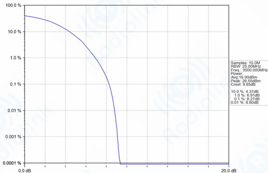
Band42_20MHz_64QAM_MCH_3500MHz_RB_100_0_NTNV
