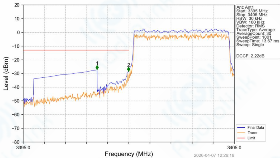
Band42_5MHz_16QAM_LCH_3402.5MHz_RB_25_0_NTNV
