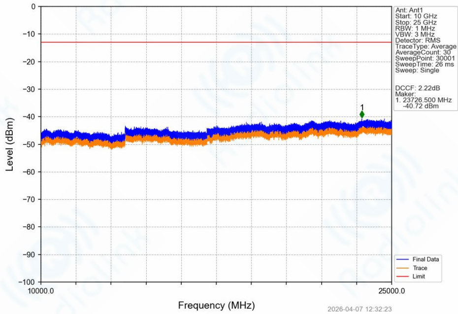
Band42_5MHz_16QAM_HCH_3597.5MHz_RB_1_0_NTNV
