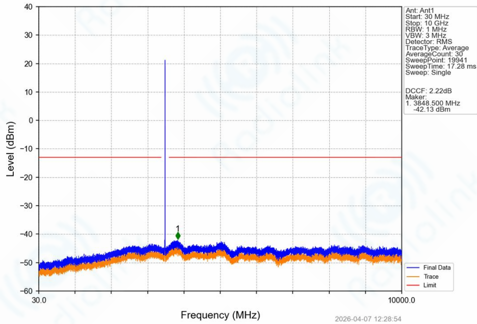
Band42_5MHz_16QAM_MCH_3500MHz_RB_1_0_NTNV
