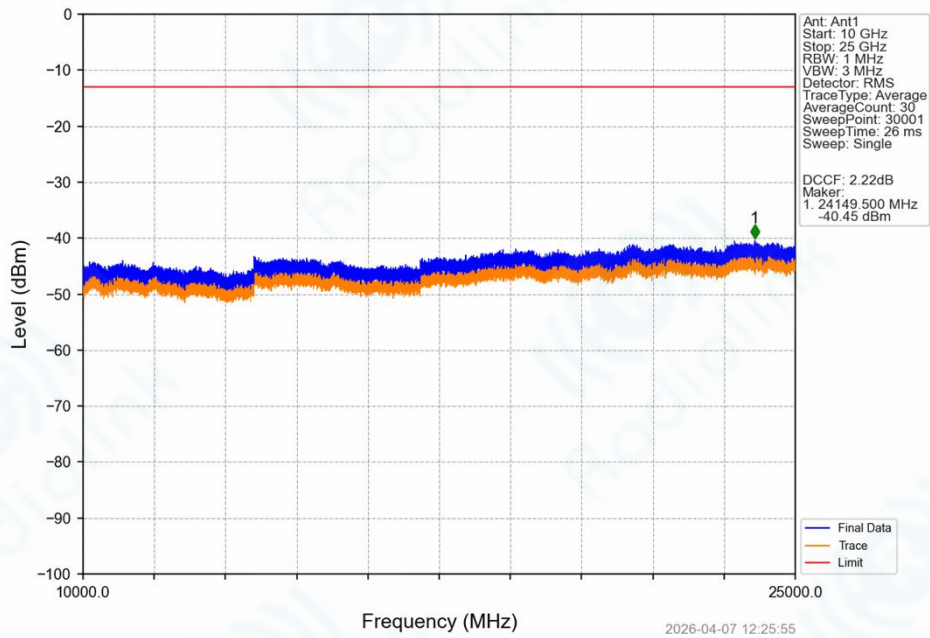
Band42_5MHz_16QAM_LCH_3402.5MHz_RB_1_0_NTNV
