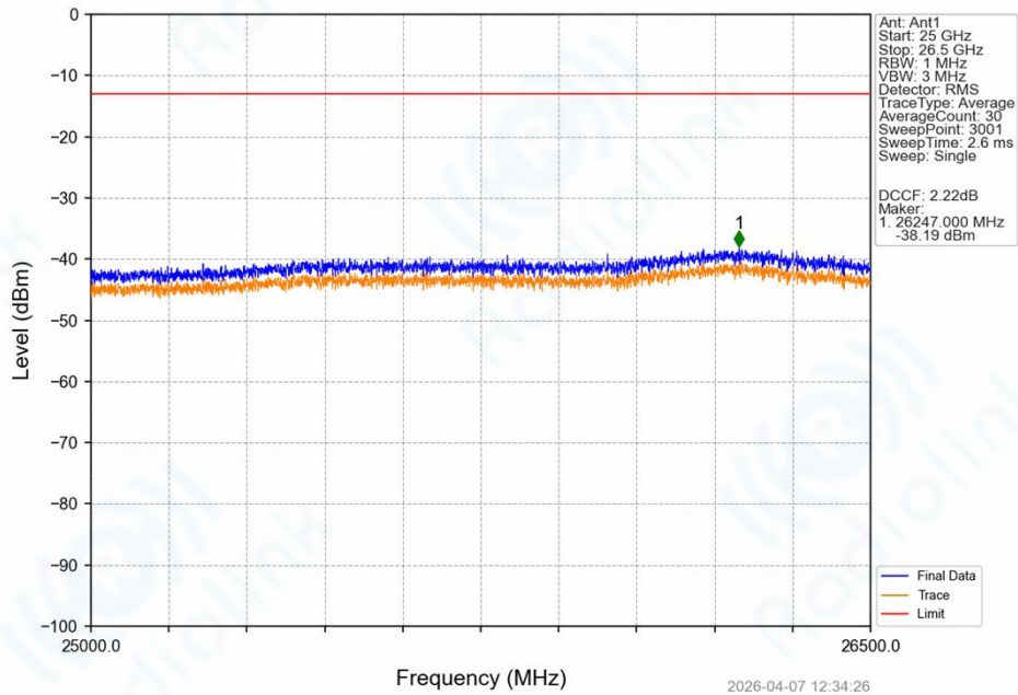
Band42_5MHz_64QAM_HCH_3597.5MHz_RB_1_24_NTNV
