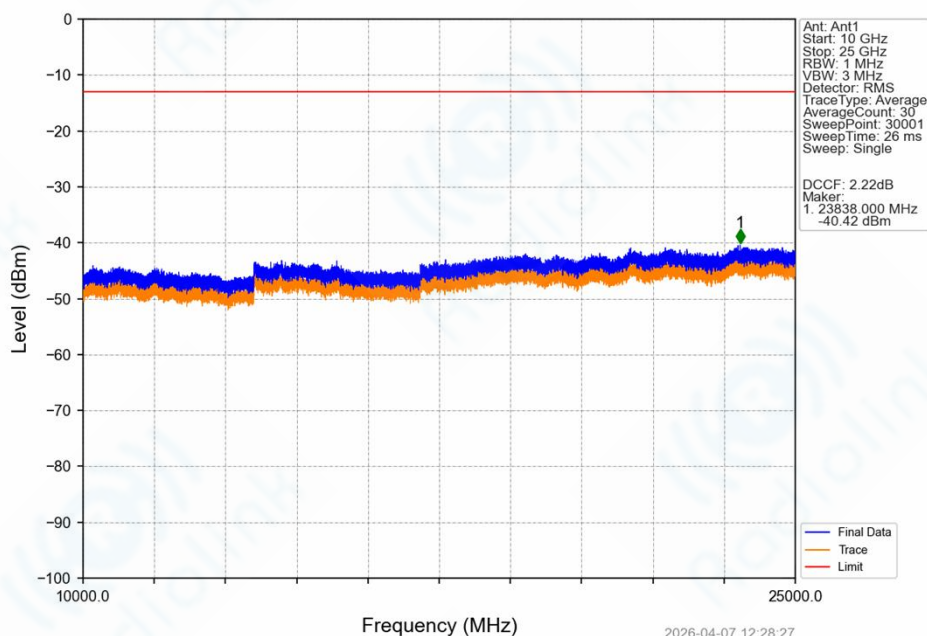
Band42_5MHz_QPSK_MCH_3500MHz_RB_1_0_NTNV
