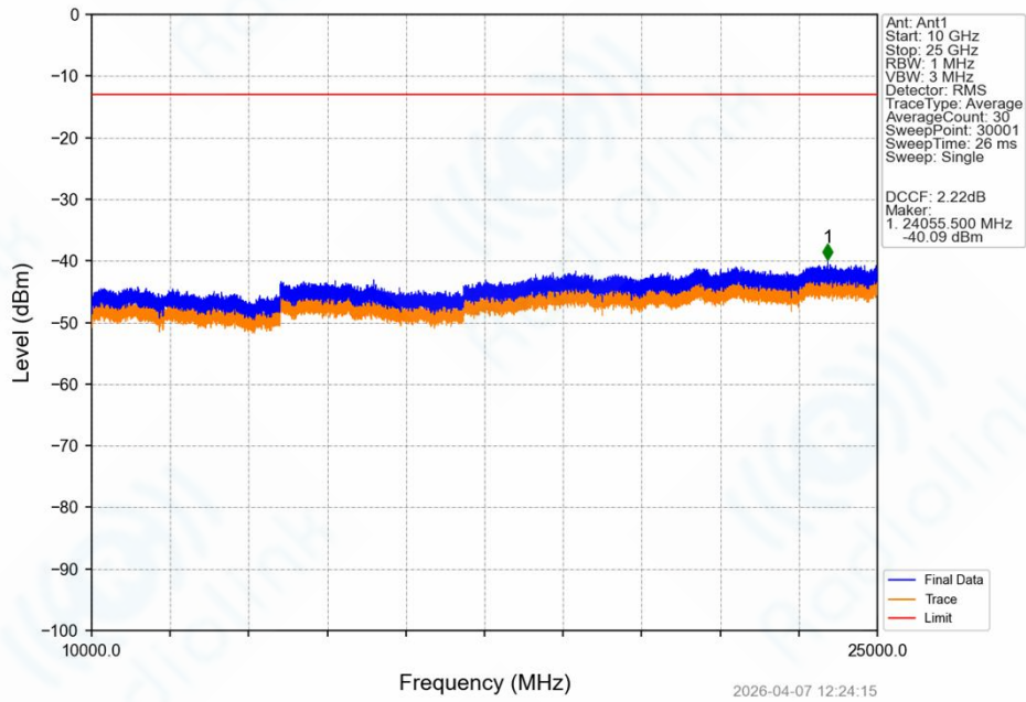
Band42_5MHz_QPSK_LCH_3402.5MHz_RB_1_0_NTNV
