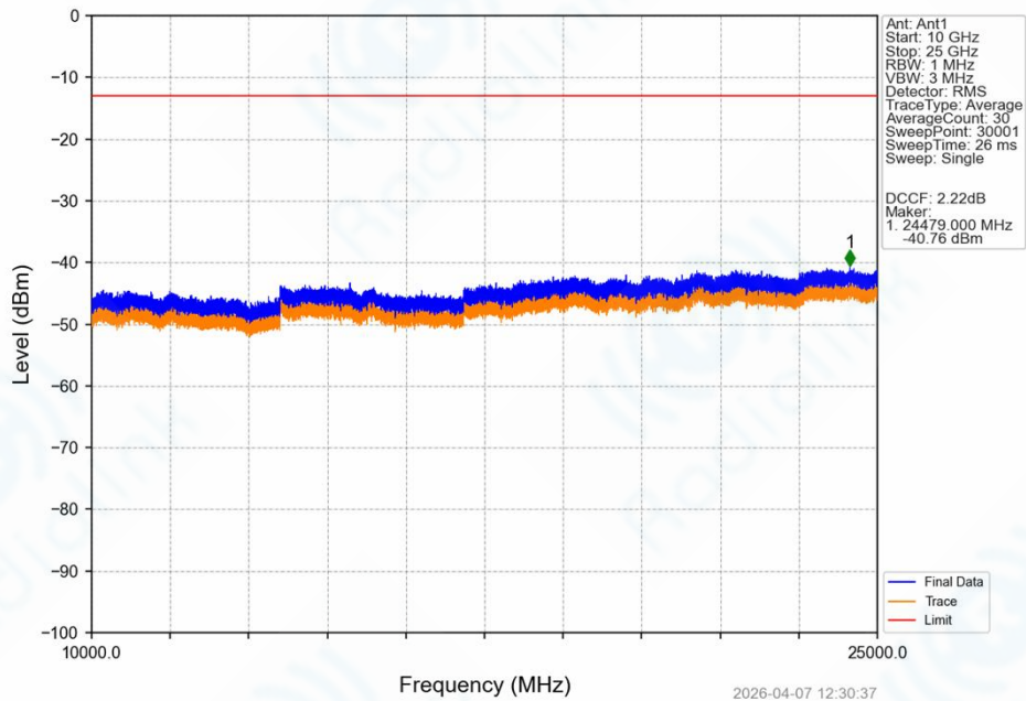
Band42_5MHz_QPSK_HCH_3597.5MHz_RB_1_0_NTNV
