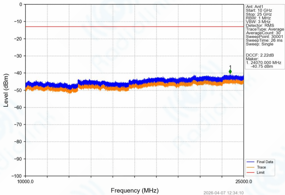
Band42_5MHz_64QAM_HCH_3597.5MHz_RB_1_0_NTNV
