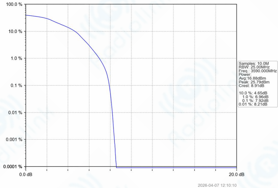
Band42_20MHz_16QAM_HCH_3590MHz_RB_100_0_NTNV
