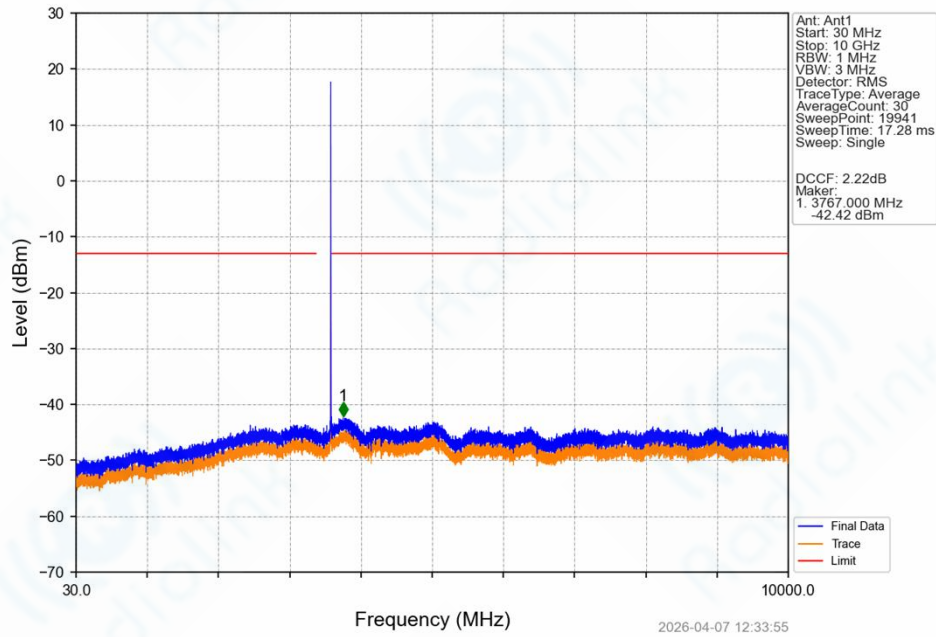
Band42_5MHz_64QAM_HCH_3597.5MHz_RB_1_0_NTNV
