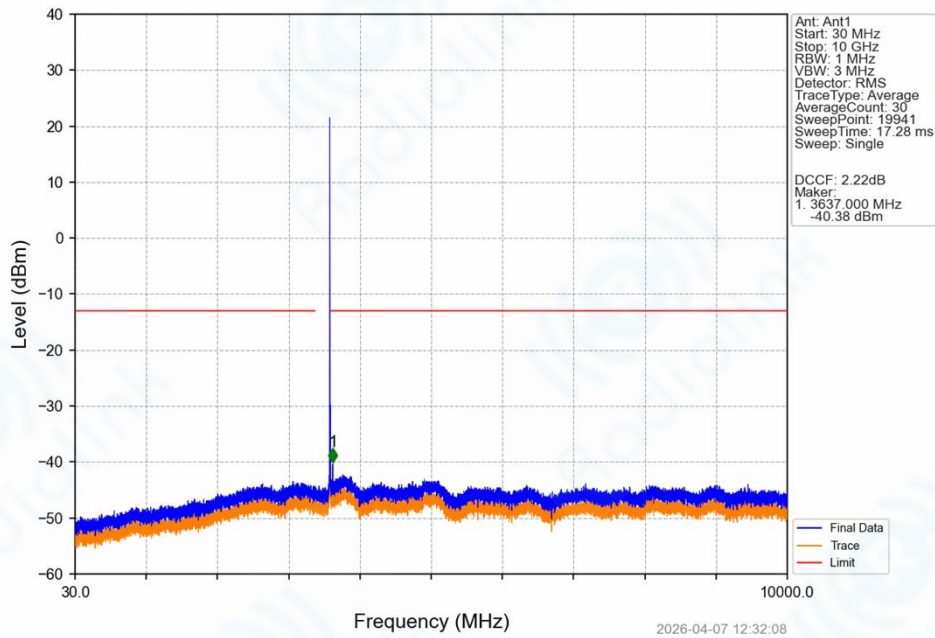
Band42_5MHz_16QAM_HCH_3597.5MHz_RB_1_0_NTNV
