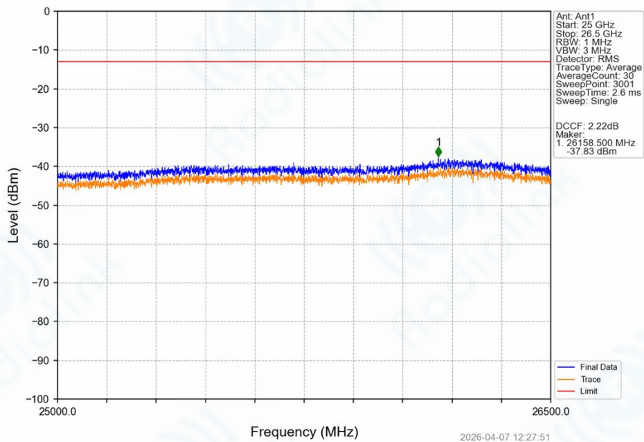
Band42_5MHz_64QAM_LCH_3402.5MHz_RB_1_0_NTNV
