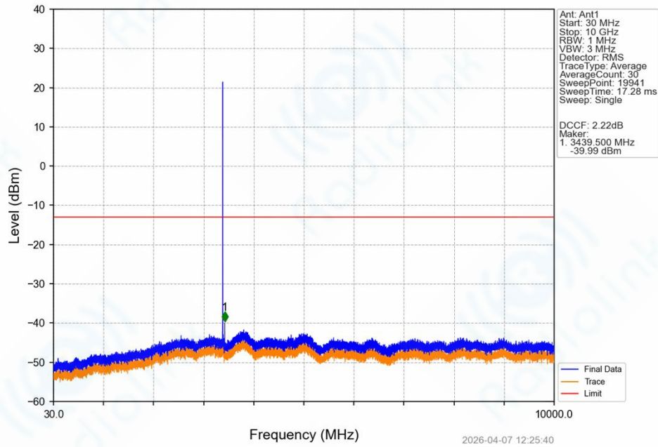
Band42_5MHz_16QAM_LCH_3402.5MHz_RB_1_0_NTNV
