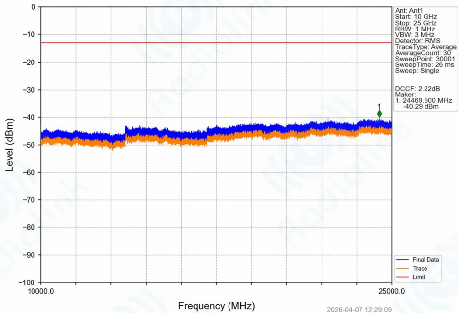
Band42_5MHz_16QAM_MCH_3500MHz_RB_1_0_NTNV
