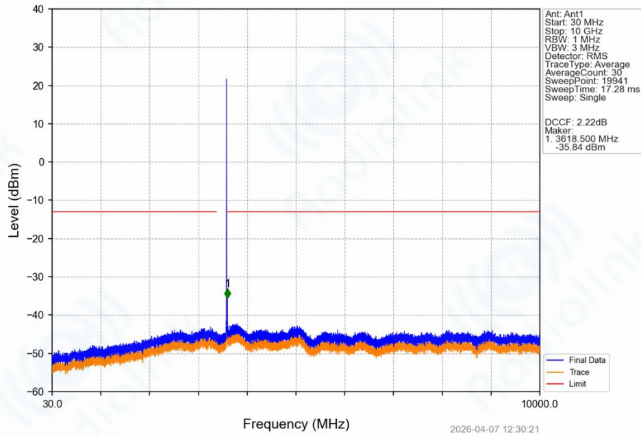
Band42_5MHz_QPSK_HCH_3597.5MHz_RB_1_0_NTNV
