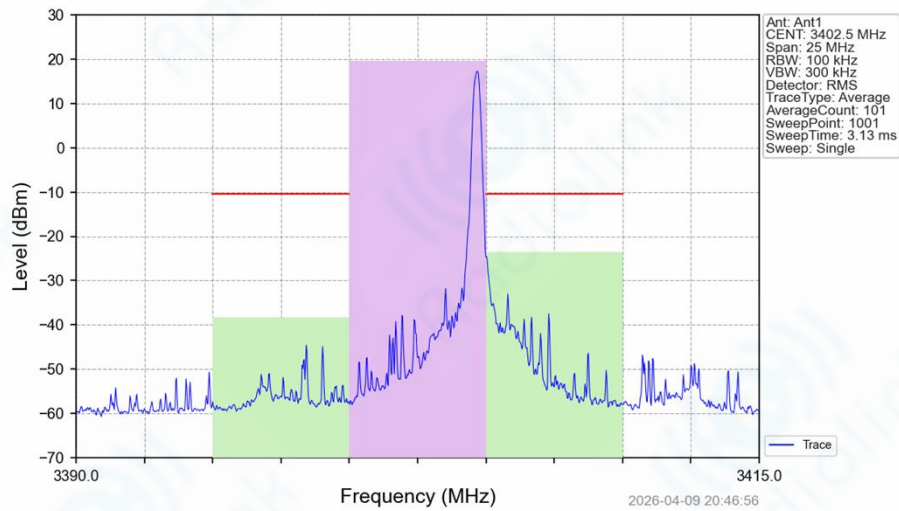
Band42_5MHz_16QAM_LCH_3402.5MHz_RB_1_24_NTNV
