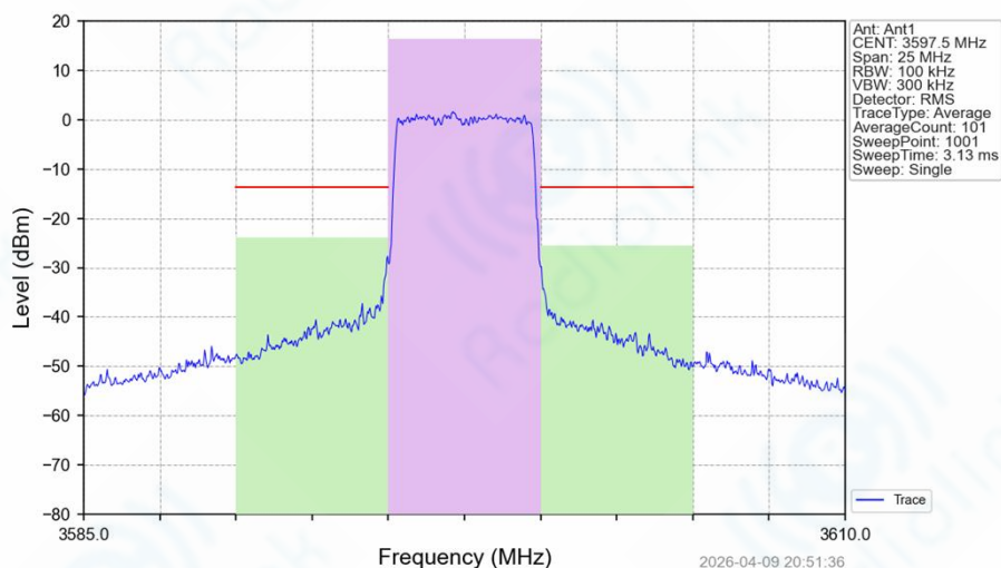
Band42_5MHz_64QAM_HCH_3597.5MHz_RB_25_0_NTNV
