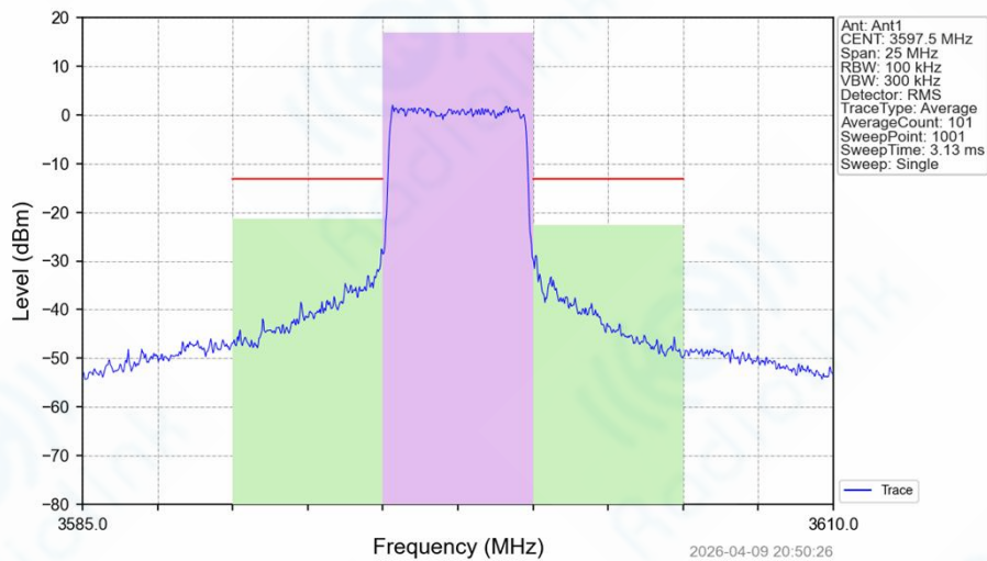
Band42_5MHz_16QAM_HCH_3597.5MHz_RB_25_0_NTNV
