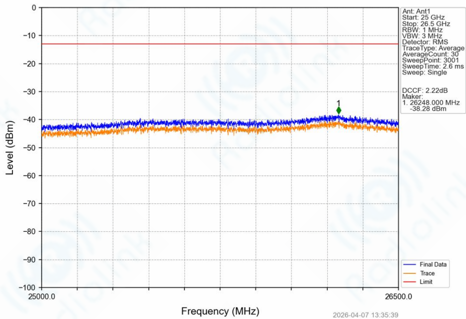
Band42_20MHz_64QAM_HCH_3590MHz_RB_1_99_NTNV
