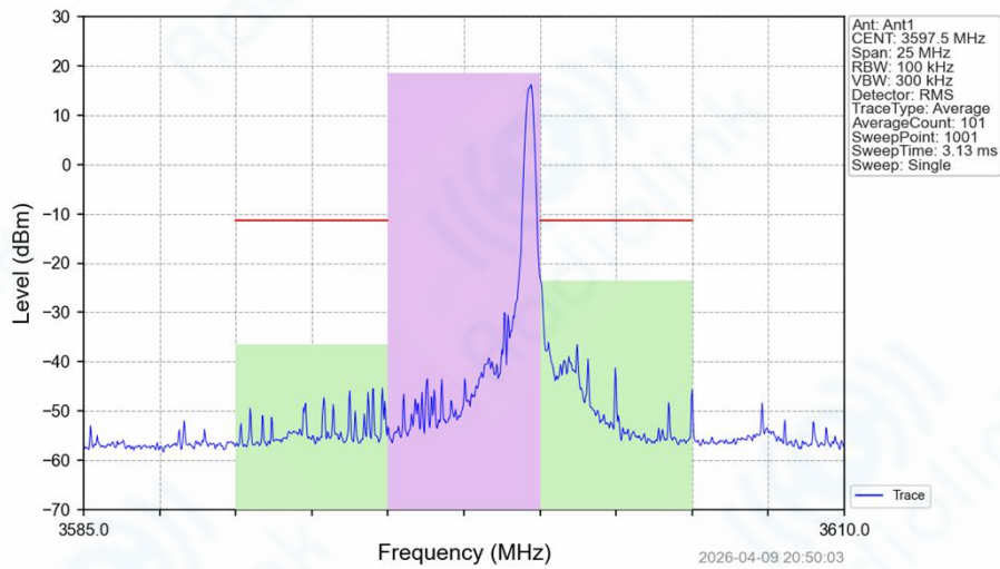
Band42_5MHz_16QAM_HCH_3597.5MHz_RB_1_24_NTNV
