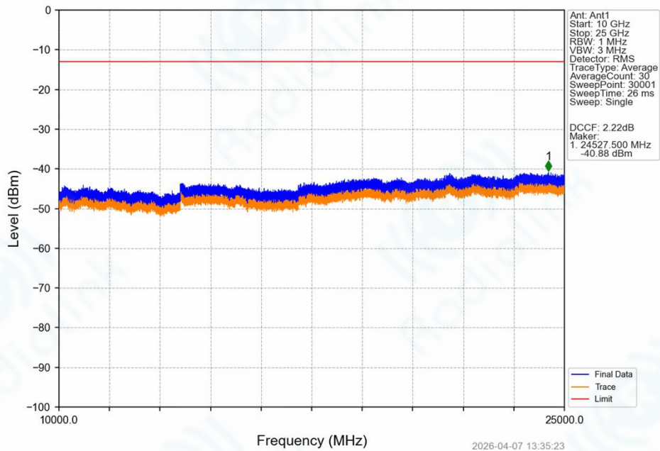
Band42_20MHz_64QAM_HCH_3590MHz_RB_1_0_NTNV
