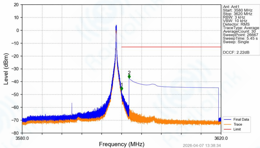
Band42_20MHz_64QAM_HCH_3590MHz_RB_1_99_NTNV
