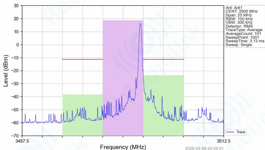
Band42_5MHz_64QAM_MCH_3500MHz_RB_1_24_NTNV
