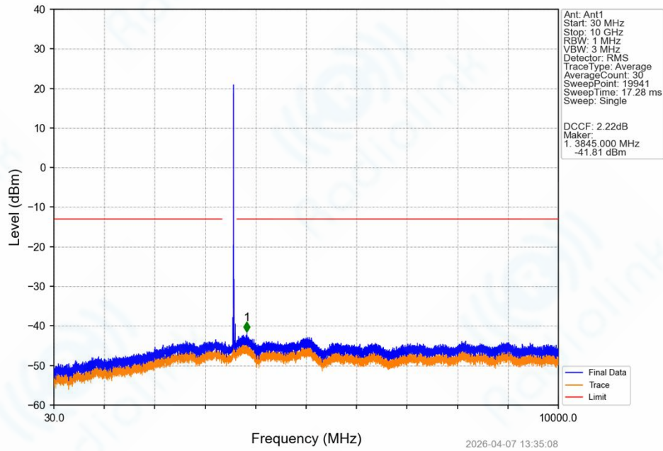
Band42_20MHz_64QAM_HCH_3590MHz_RB_1_0_NTNV
