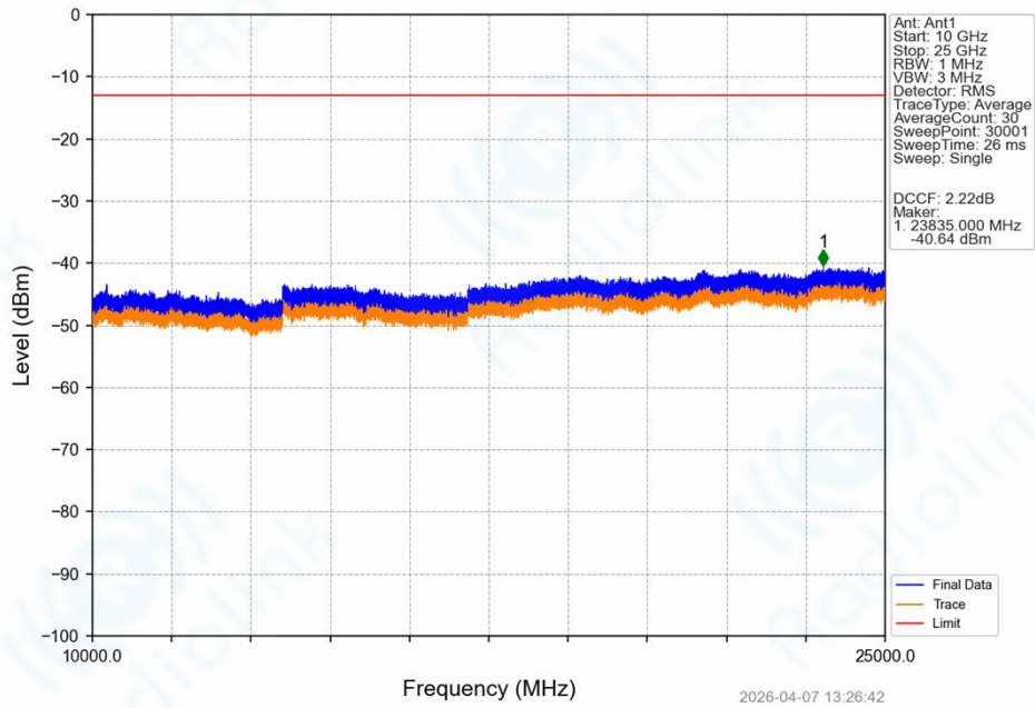
Band42_20MHz_64QAM_MCH_3500MHz_RB_1_0_NTNV
