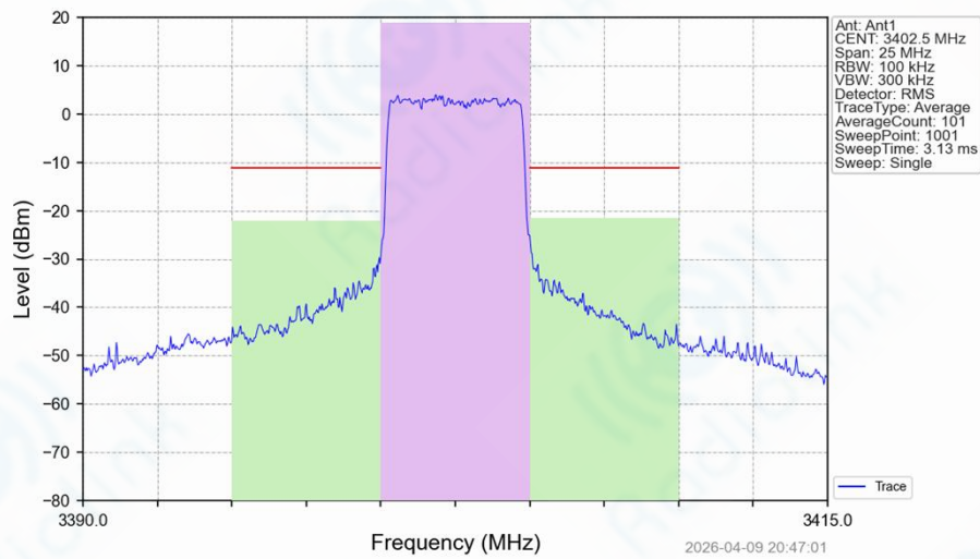
Band42_5MHz_16QAM_LCH_3402.5MHz_RB_25_0_NTNV
