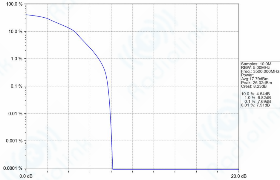
Band42a_5MHz_16QAM_MCH_3500MHz_RB_25_0_NTNV
