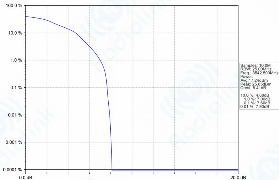
Band42a_15MHz_16QAM_HCH_3542.5MHz_RB_75_0_NTNV
