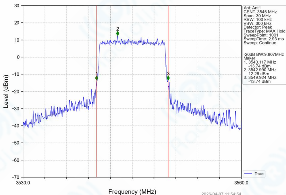
Band42a_10MHz_64QAM_HCH_3545MHz_RB_50_0_NTNV
