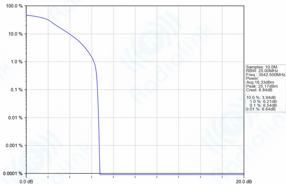
Band42a_15MHz_QPSK_HCH_3542.5MHz_RB_75_0_NTNV
