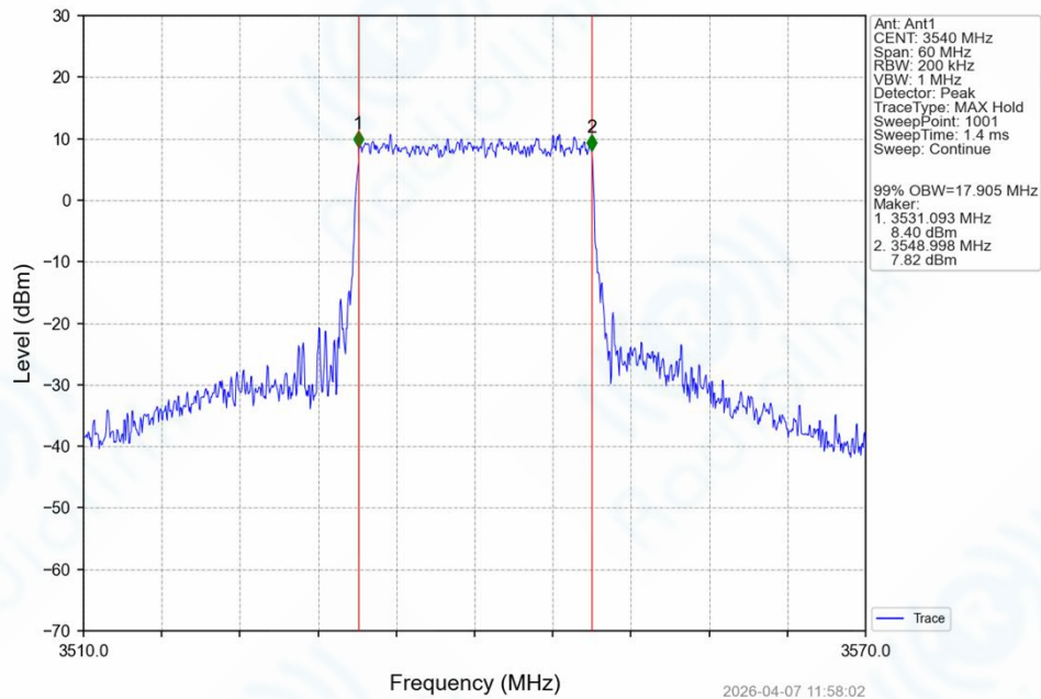
Band42a_20MHz_64QAM_HCH_3540MHz_RB_100_0_NTNV
