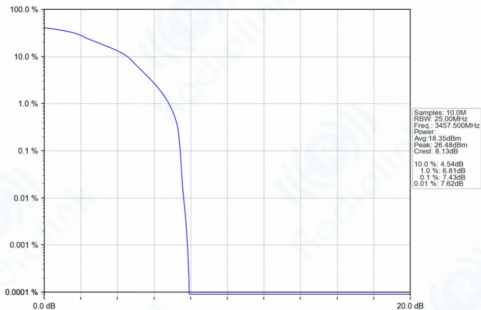
Band42a_15MHz_16QAM_LCH_3457.5MHz_RB_75_0_NTNV
