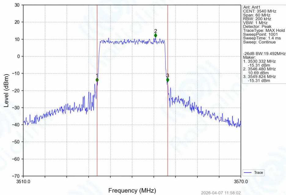
Band42a_20MHz_64QAM_HCH_3540MHz_RB_100_0_NTNV
