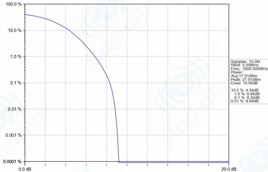
Band42a_5MHz_64QAM_MCH_3500MHz_RB_25_0_NTNV
