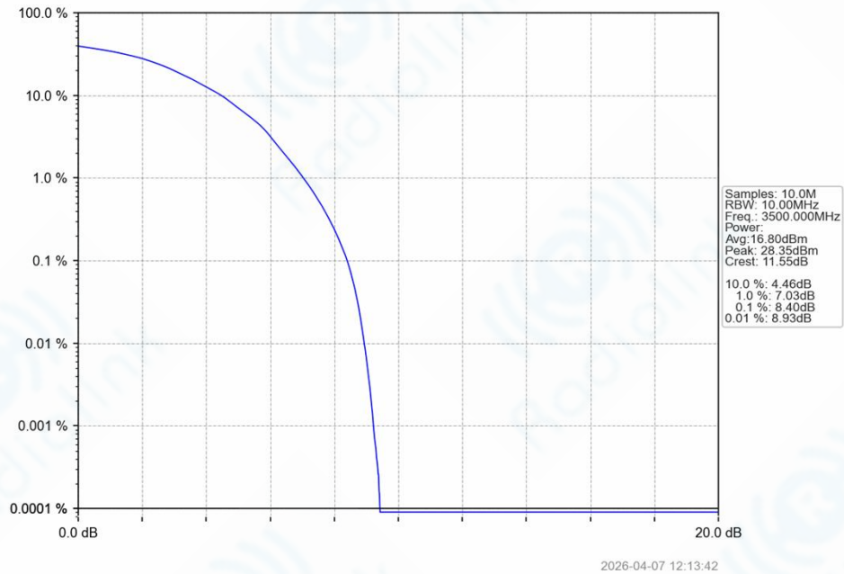
Band42a_10MHz_64QAM_MCH_3500MHz_RB_50_0_NTNV
