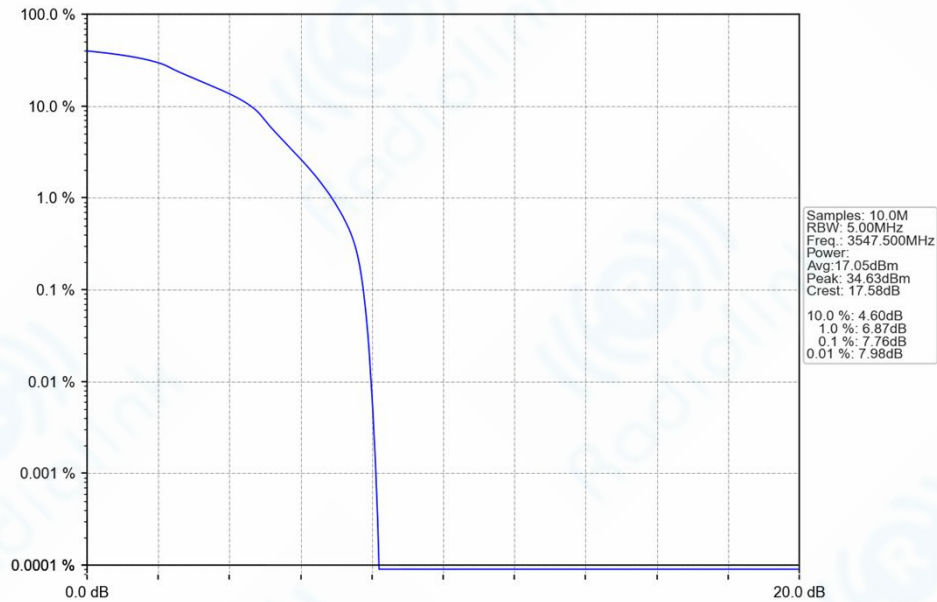
Band42a_5MHz_16QAM_HCH_3547.5MHz_RB_25_0_NTNV
