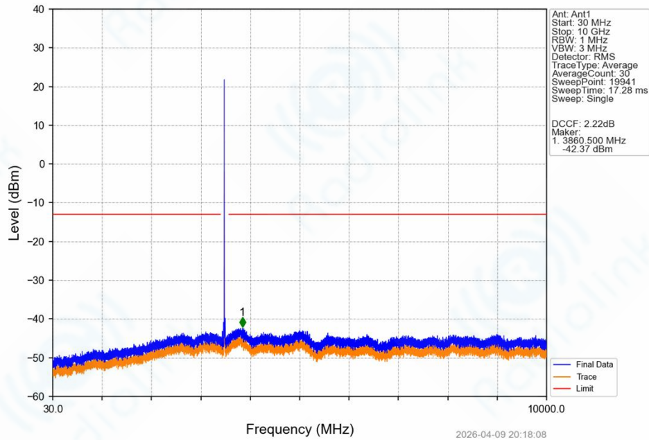
Band42a_15MHz_16QAM_MCH_3500MHz_RB_1_0_NTNV
