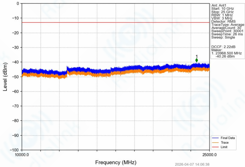
Band42a_10MHz_64QAM_LCH_3455MHz_RB_1_0_NTNV
