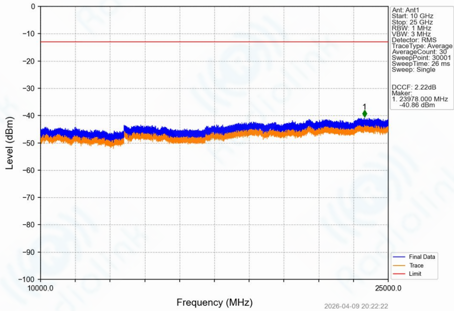
Band42a_15MHz_16QAM_HCH_3542.5MHz_RB_1_0_NTNV
