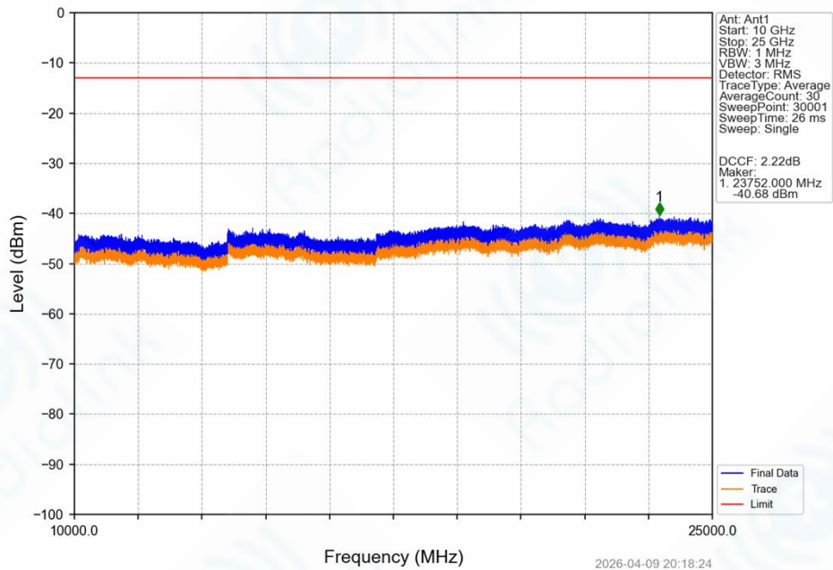
Band42a_15MHz_16QAM_MCH_3500MHz_RB_1_0_NTNV
