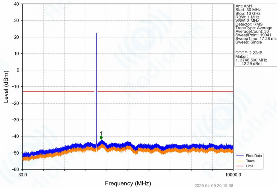
Band42a_15MHz_QPSK_HCH_3542.5MHz_RB_1_0_NTNV
