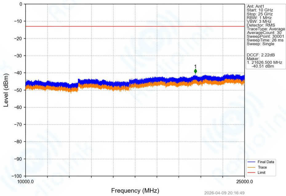
Band42a_15MHz_64QAM_LCH_3457.5MHz_RB_1_0_NTNV
