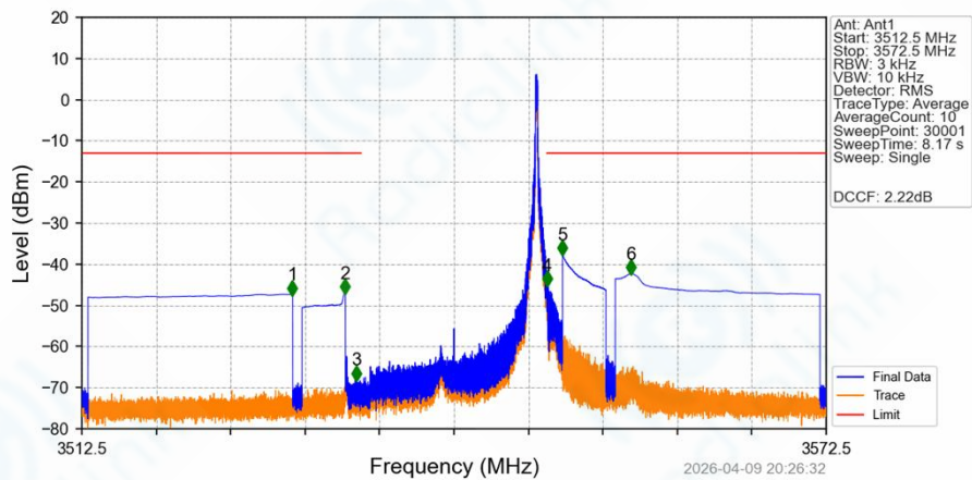
Band42a_15MHz_64QAM_HCH_3542.5MHz_RB_1_74_NTNV
