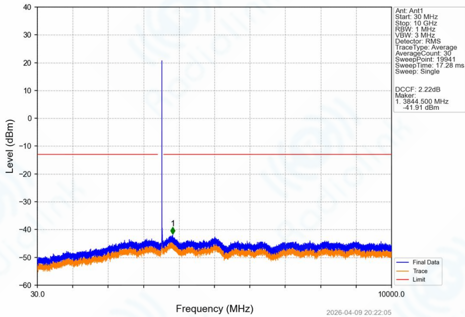
Band42a_15MHz_16QAM_HCH_3542.5MHz_RB_1_0_NTNV
