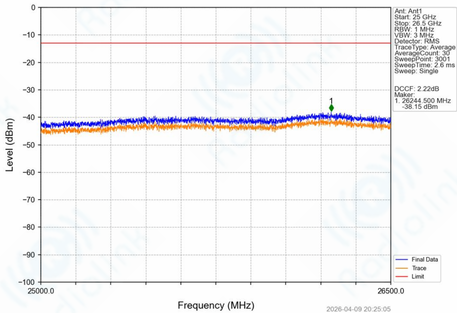
Band42a_15MHz_64QAM_HCH_3542.5MHz_RB_1_74_NTNV
