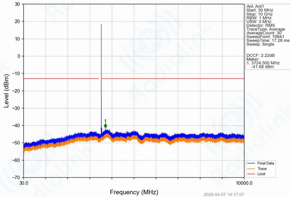
Band42a_10MHz_64QAM_HCH_3545MHz_RB_1_0_NTNV
