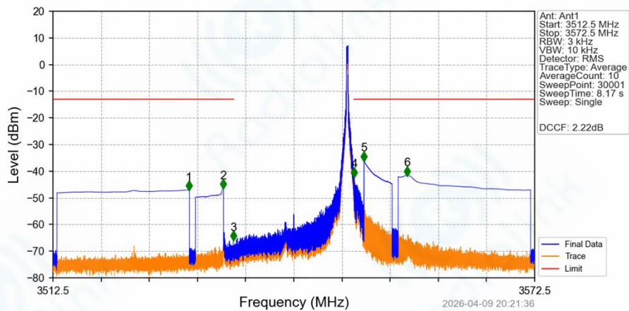
Band42a_15MHz_QPSK_HCH_3542.5MHz_RB_1_74_NTNV
