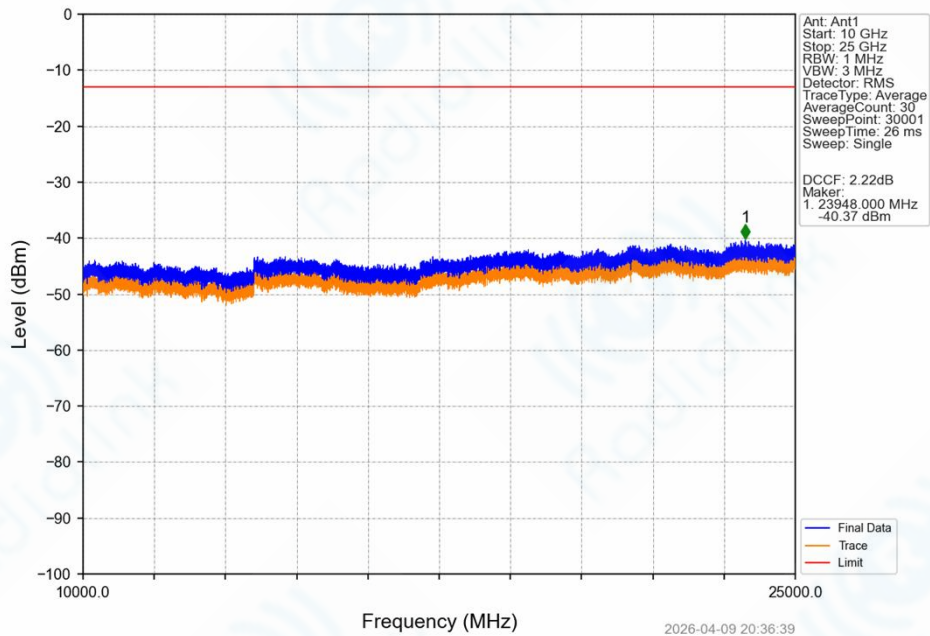
Band42a_20MHz_16QAM_MCH_3500MHz_RB_1_0_NTNV
