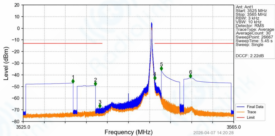
Band42a_10MHz_64QAM_HCH_3545MHz_RB_1_49_NTNV
