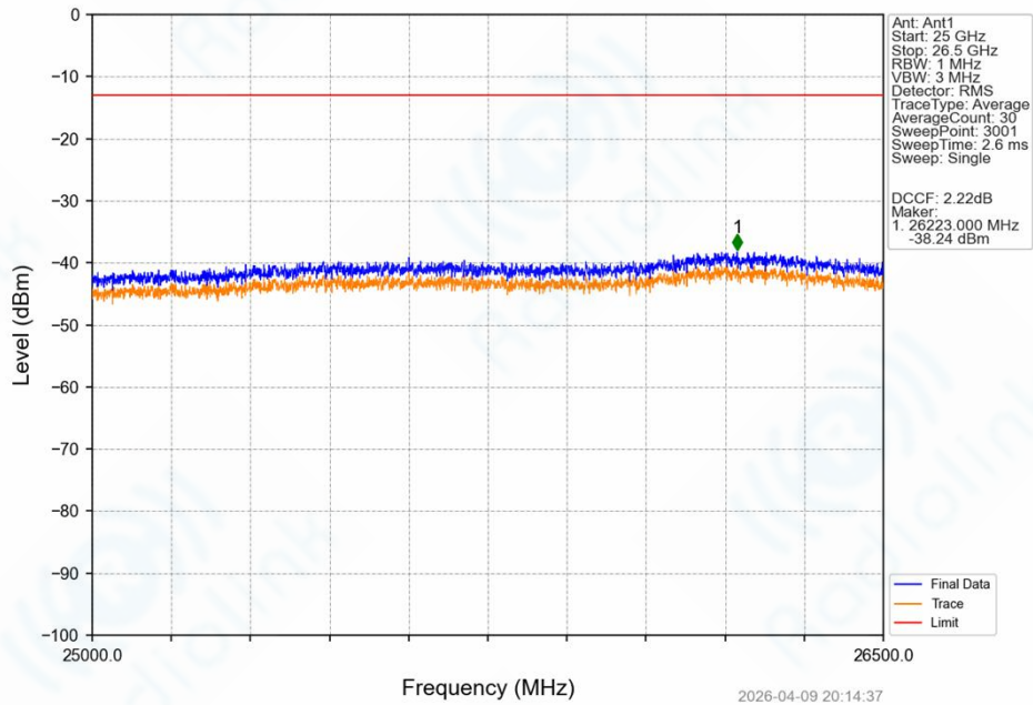
Band42a_15MHz_16QAM_LCH_3457.5MHz_RB_75_0_NTNV
