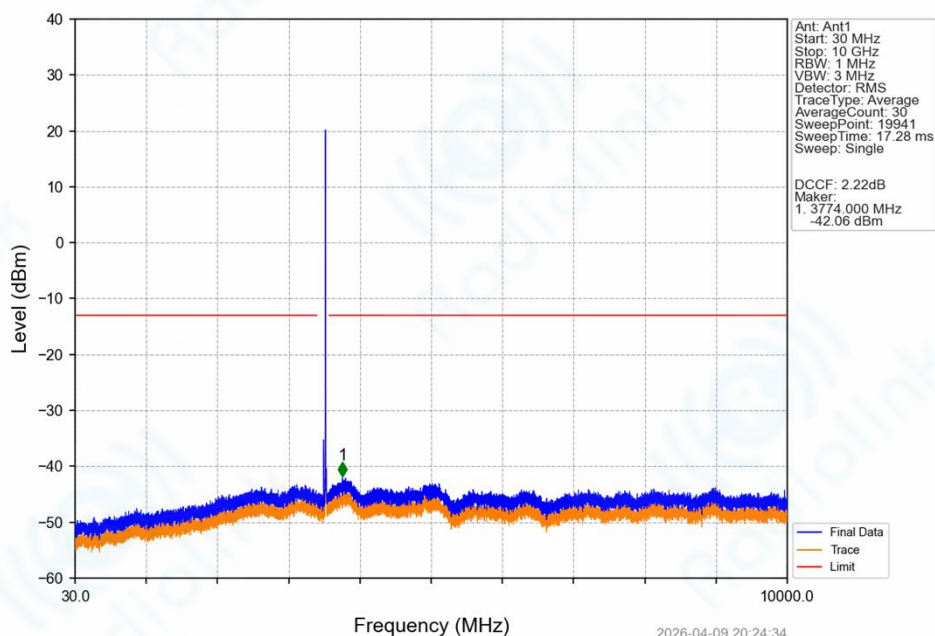
Band42a_15MHz_64QAM_HCH_3542.5MHz_RB_1_0_NTNV
