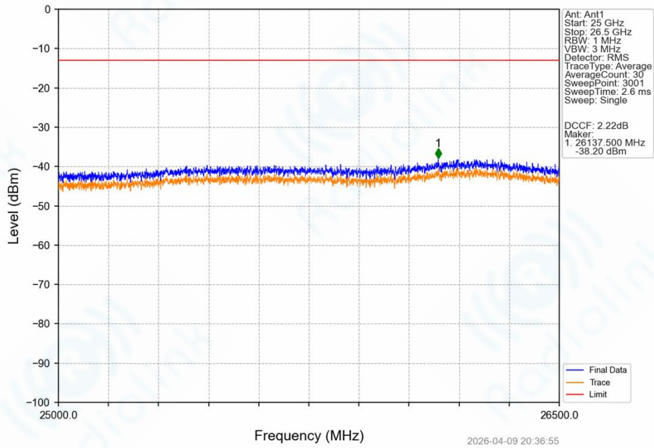
Band42a_20MHz_16QAM_HCH_3540MHz_RB_1_0_NTNV
