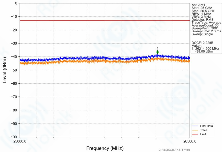
Band42a_10MHz_64QAM_HCH_3545MHz_RB_1_49_NTNV
