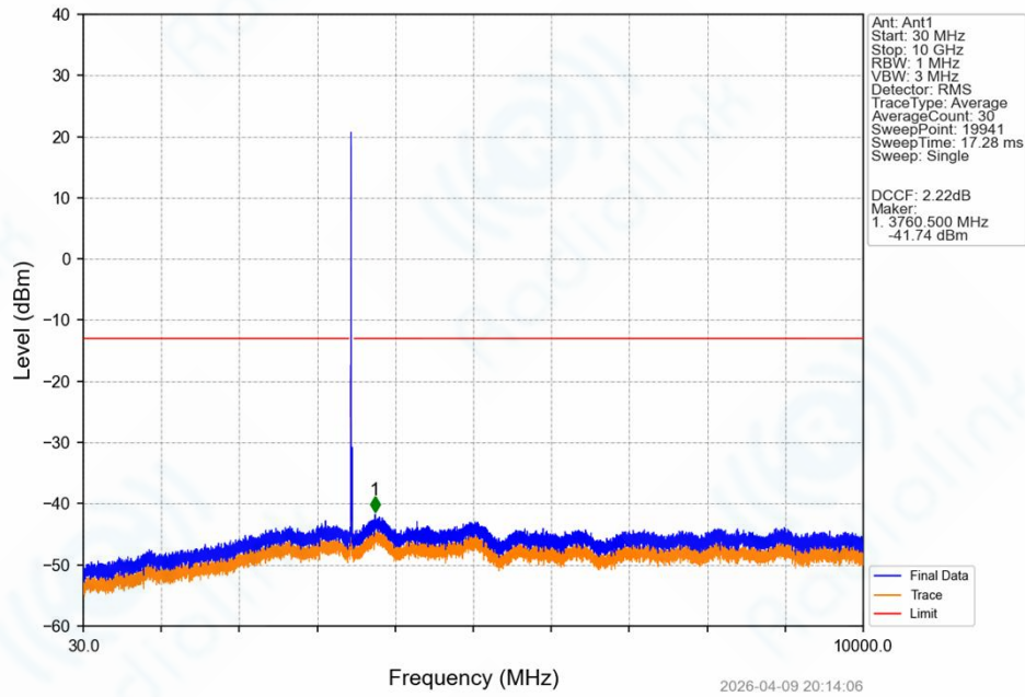
Band42a_15MHz_16QAM_LCH_3457.5MHz_RB_1_0_NTNV
