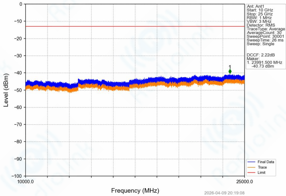
Band42a_15MHz_64QAM_MCH_3500MHz_RB_1_0_NTNV
