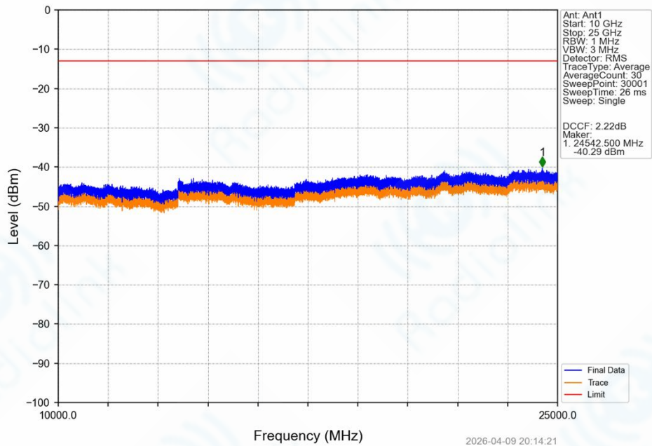
Band42a_15MHz_16QAM_LCH_3457.5MHz_RB_1_0_NTNV
