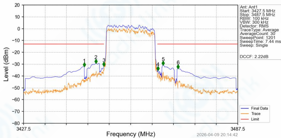
Band42a_15MHz_16QAM_LCH_3457.5MHz_RB_75_0_NTNV
