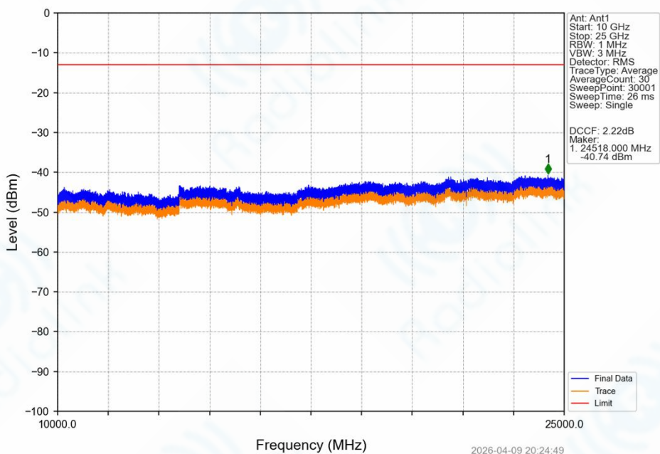
Band42a_15MHz_64QAM_HCH_3542.5MHz_RB_1_0_NTNV
