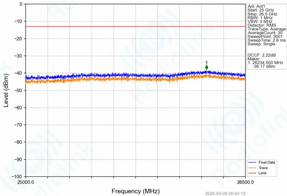
Band42a_20MHz_64QAM_HCH_3540MHz_RB_1_99_NTNV
