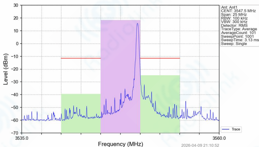
Band42a_5MHz_64QAM_HCH_3547.5MHz_RB_1_24_NTNV
