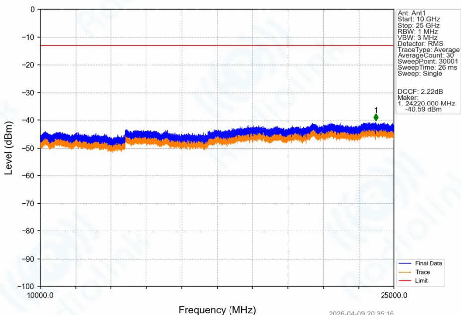
Band42a_20MHz_64QAM_LCH_3460MHz_RB_1_0_NTNV
