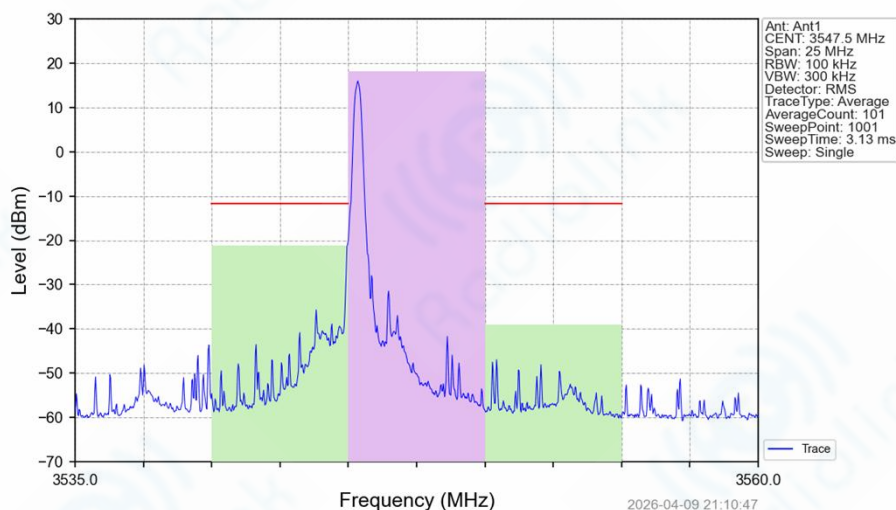
Band42a_5MHz_64QAM_HCH_3547.5MHz_RB_1_0_NTNV
