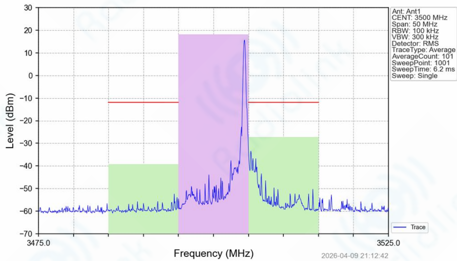
Band42a_10MHz_64QAM_MCH_3500MHz_RB_1_49_NTNV
