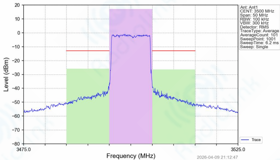
Band42a_10MHz_64QAM_MCH_3500MHz_RB_50_0_NTNV
