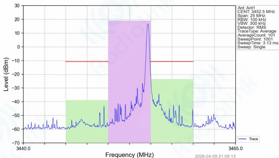
Band42a_5MHz_64QAM_LCH_3452.5MHz_RB_1_24_NTV
