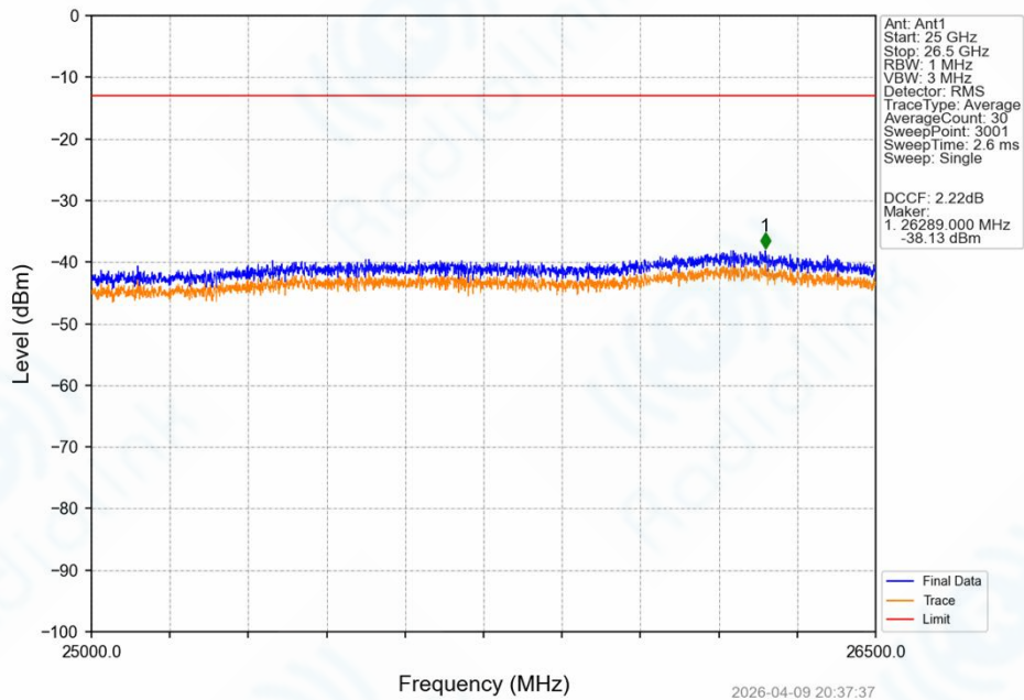
Band42a_20MHz_64QAM_MCH_3500MHz_RB_1_0_NTNV
