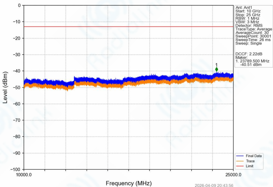
Band42a_20MHz_64QAM_HCH_3540MHz_RB_1_0_NTNV
