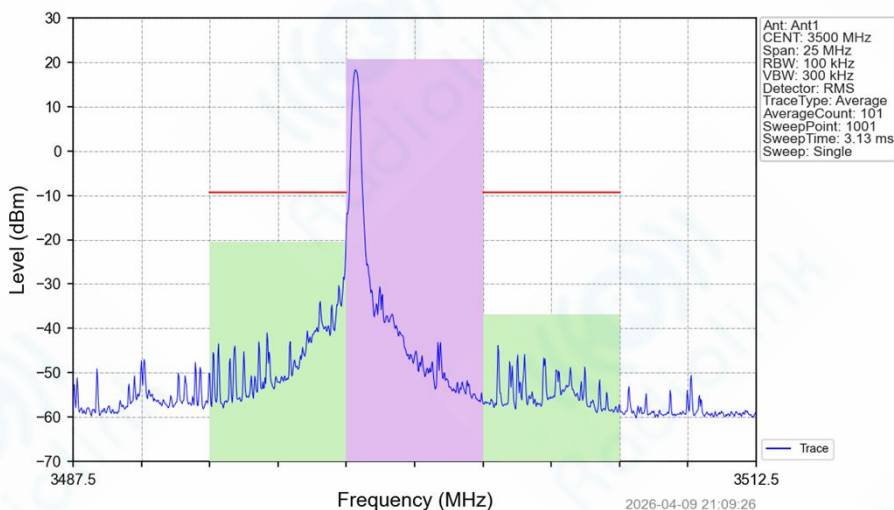
Band42a_5MHz_QPSK_MCH_3500MHz_RB_1_0_NTNV
