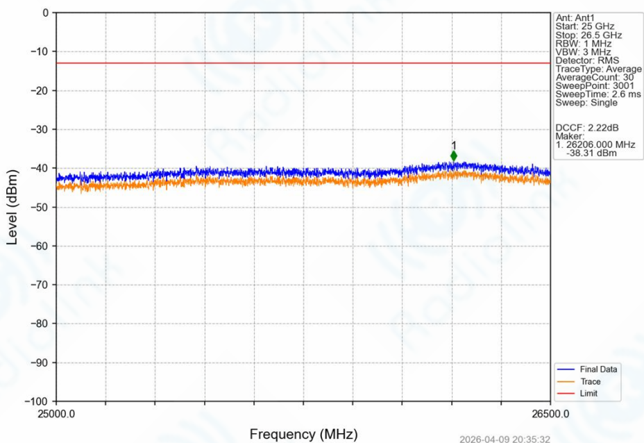
Band42a_20MHz_64QAM_LCH_3460MHz_RB_1_0_NTNV
