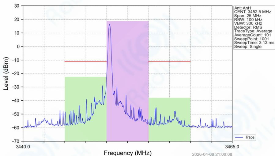
Band42a_5MHz_64QAM_LCH_3452.5MHz_RB_1_0_NTV
