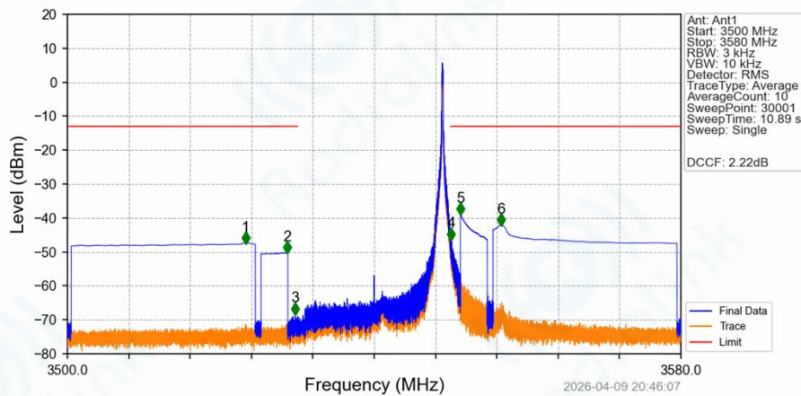
Band42a_20MHz_64QAM_HCH_3540MHz_RB_1_99_NTNV
