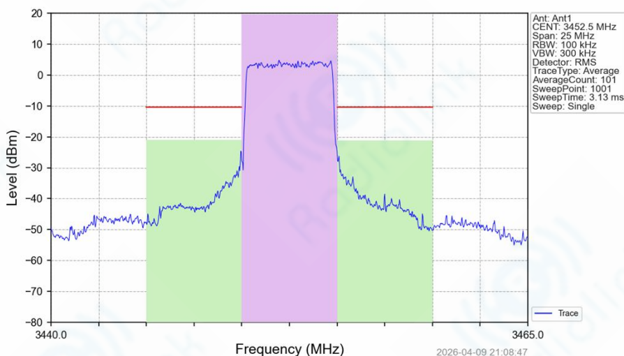
Band42a_5MHz_QPSK_LCH_3452.5MHz_RB_25_0_NTNV
