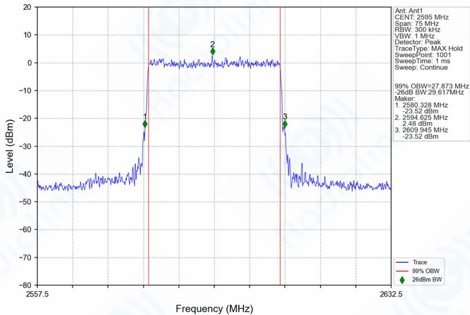
n38_30kHz_SISO_NTNV_30MHz_CP-OFDM_256_QAM_2595MHz_Outer_Full_Ant1
