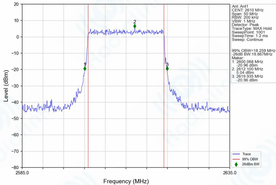
n38_30kHz_SISO_NTNV_20MHz_CP-OFDM QPSK_2610MHz_Outer_Full_Ant1
