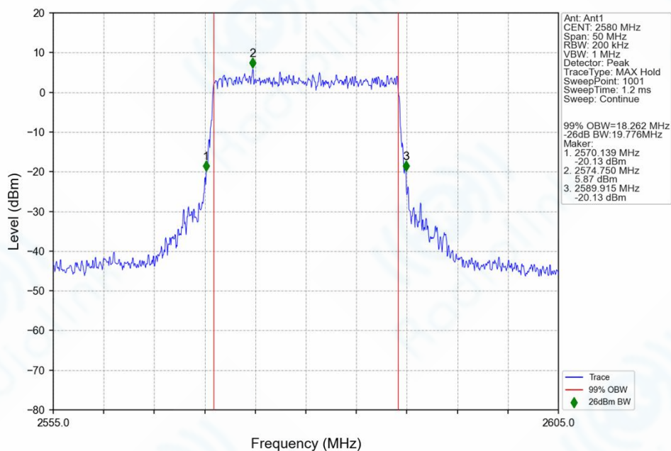
n38_30kHz_SISO_NTNV_20MHz_CP-OFDM_64_QAM_2580MHz_Outer_Full_Ant1
