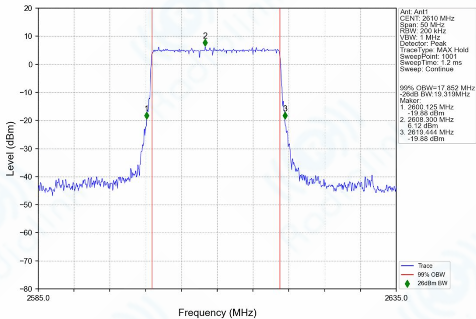
n38_30kHz_SISO_NTNV_20MHz_DFT-s-OFDM_64_QAM_2610MHz_Outer_Full_Ant1
