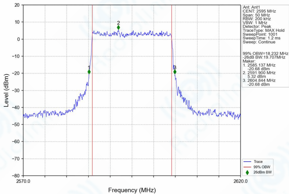
n38_30kHz_SISO_NTNV_20MHz_CP-OFDM_16_QAM_2595MHz_Outer_Full_Ant1
