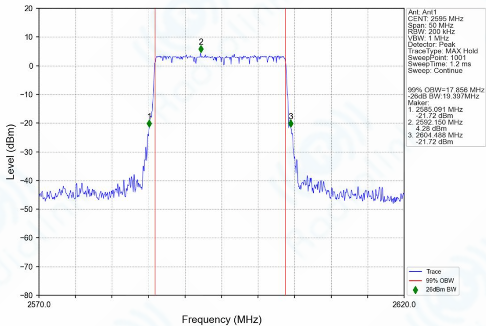
n38_30kHz_SISO_NTNV_20MHz_DFT-s-OFDM_256 QAM_2595MHz_Outer_Full_Ant1
