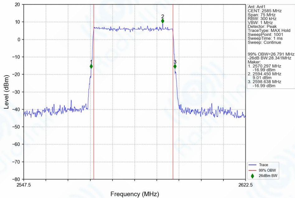
n38_30kHz_SISO_NTNV_30MHz_DFT-s-OFDM QPSK_2585MHz_Outer_Full_Ant1
