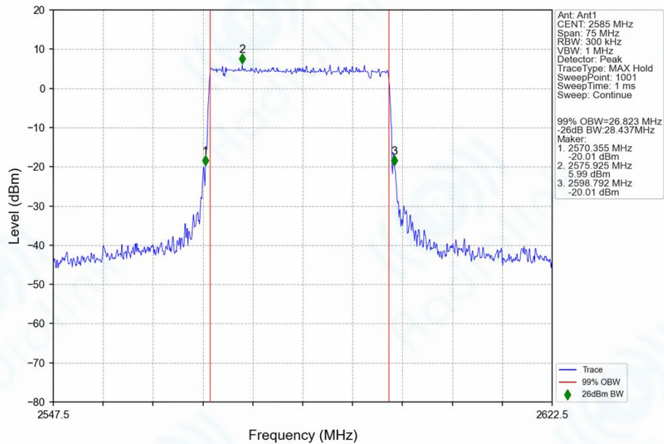
n38_30kHz_SISO_NTNV_30MHz_DFT-s-OFDM_64_QAM_2585MHz_Outer_Full_Ant1
