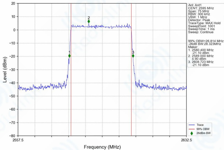
n38_30kHz_SISO_NTNV_30MHz_DFT-s-OFDM_256 QAM_2595MHz_Outer_Full_Ant1
