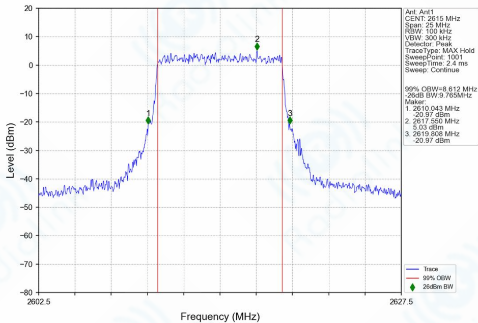
n38_30kHz_SISO_NTNV_10MHz_CP-OFDM_64_QAM_2615MHz_Outer_Full_Ant1
