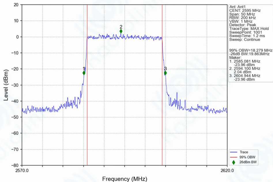
n38_30kHz_SISO_NTNV_20MHz_CP-OFDM_256_QAM_2595MHz_Outer_Full_Ant1
