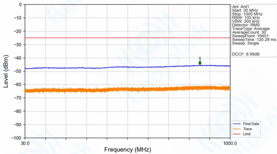
n41_30kHz_SISO_NTNV_90MHz_CP-OFDM_QPSK_2644.98MHz_Edge_1RB_Right_Ant1
