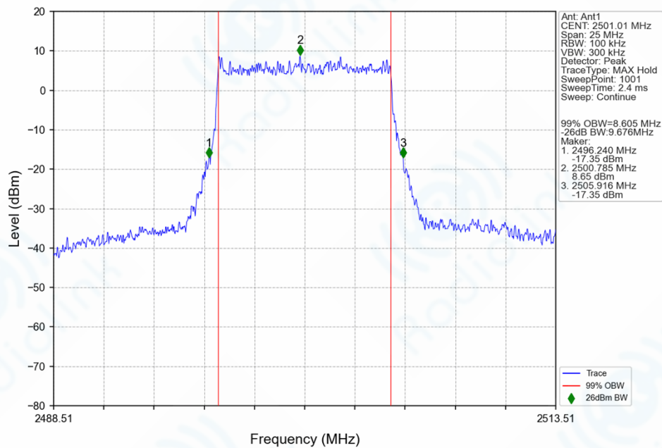
n41_30kHz_SISO_NTNV_10MHz_DFT-s-OFDM_64_QAM_2501.01MHz_Outer_Full_Ant1
