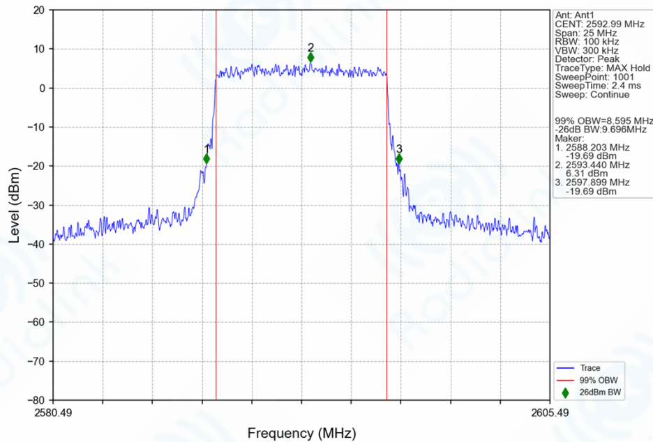
n41_30kHz_SISO_NTNV_10MHz_CP-OFDM_256_QAM_2592.99MHz_Outer_Full_Ant1
