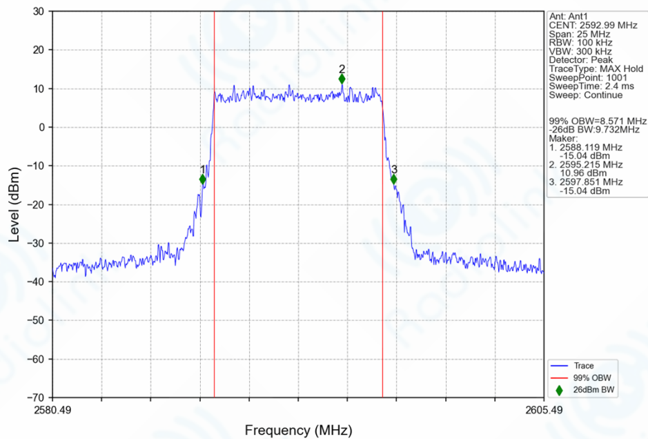
n41_30kHz_SISO_NTNV_10MHz_DFT-s-OFDM_16_QAM_2592.99MHz_Outer_Full_Ant1
