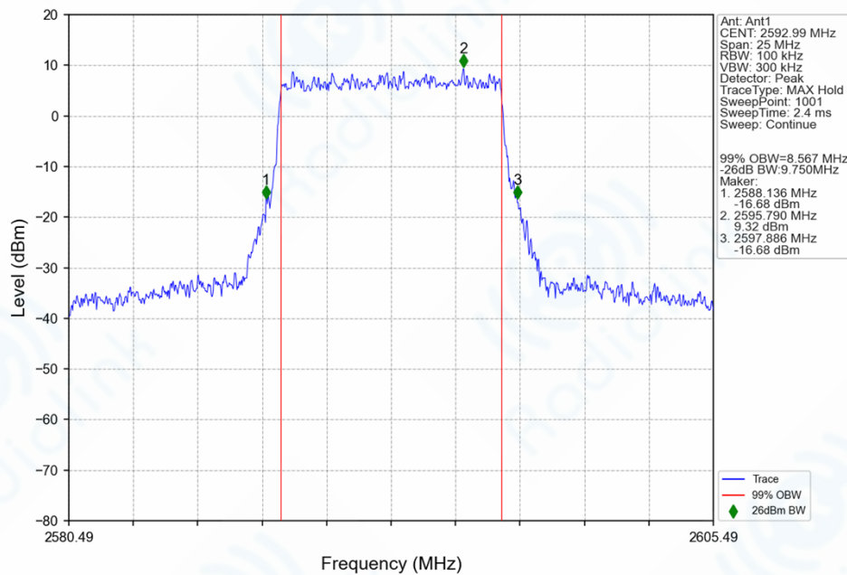
n41_30kHz_SISO_NTNV_10MHz_DFT-s-OFDM_256_QAM_2592.99MHz_Outer_Full_Ant1
