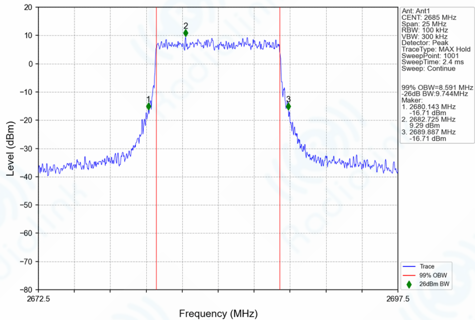
n41_30kHz_SISO_NTNV_10MHz_CP-OFDM_64_QAM_2685MHz_Outer_Full_Ant1
