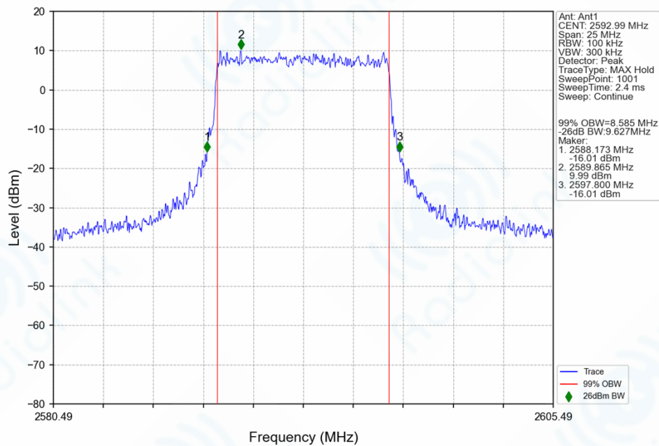
n41_30kHz_SISO_NTNV_10MHz_CP-OFDM_16_QAM_2592.99MHz_Outer_Full_Ant1
