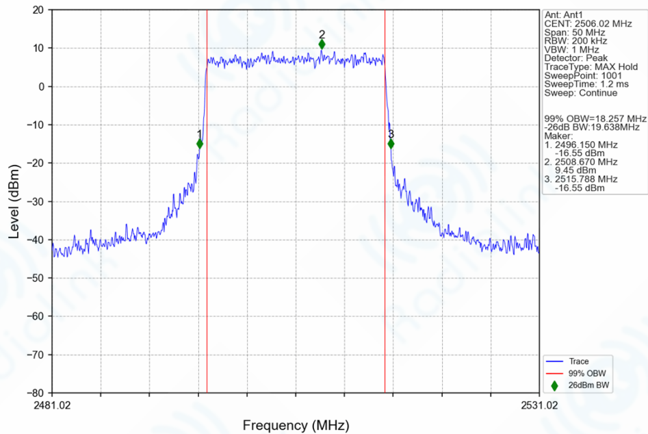
n41_30kHz_SISO_NTNV_20MHz_CP-OFDM_64_QAM_2506.02MHz_Outer_Full_Ant1
