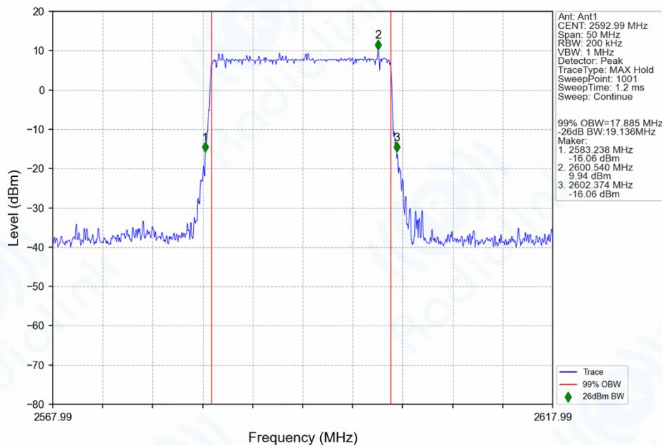
n41_30kHz_SISO_NTNV_20MHz_DFT-s-OFDM_256_QAM_2592.99MHz_Outer_Full_Ant1
