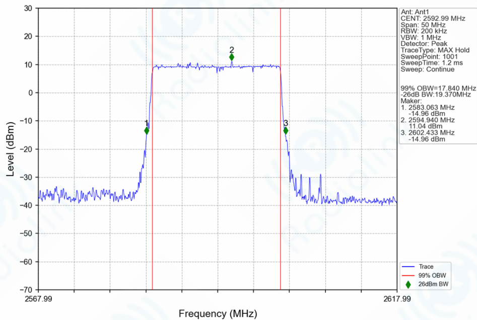
n41_30kHz_SISO_NTNV_20MHz_DFT-s-OFDM_16_QAM_2592.99MHz_Outer_Full_Ant1
