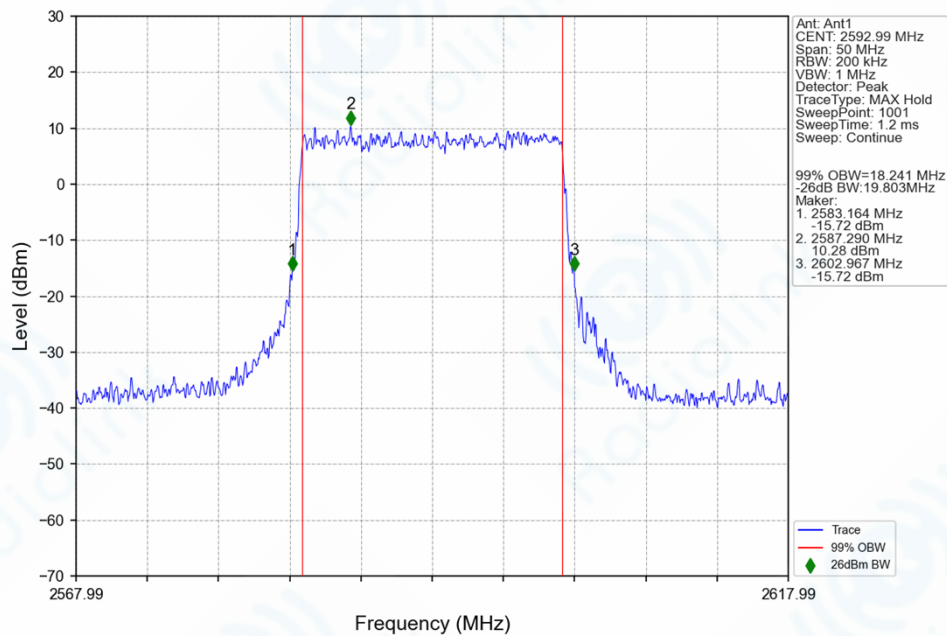
n41_30kHz_SISO_NTNV_20MHz_CP-OFDM_16_QAM_2592.99MHz_Outer_Full_Ant1
