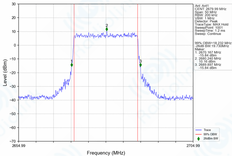
n41_30kHz_SISO_NTNV_20MHz_CP-OFDM_64_QAM_2679.99MHz_Outer_Full_Ant1
