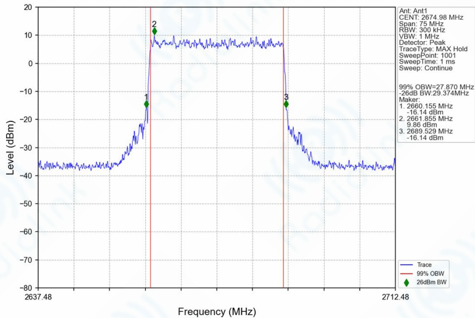
n41_30kHz_SISO_NTNV_30MHz_CP-OFDM_64_QAM_2674.98MHz_Outer_Full_Ant1
