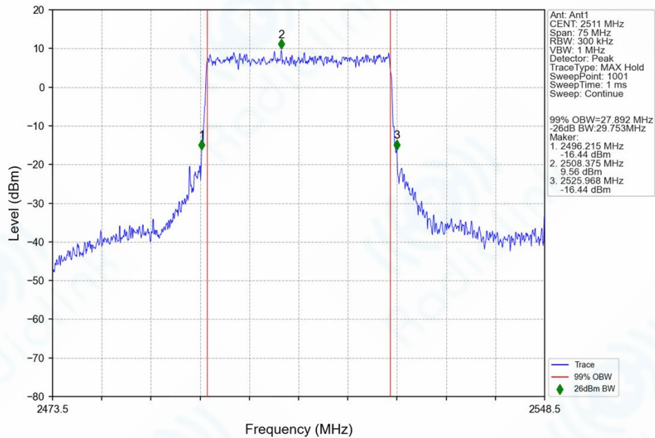
n41_30kHz_SISO_NTNV_30MHz_CP-OFDM_64_QAM_2511MHz_Outer_Full_Ant1
