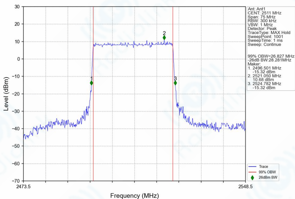
n41_30kHz_SISO_NTNV_30MHz_DFT-s-OFDM_64_QAM_2511MHz_Outer_Full_Ant1
