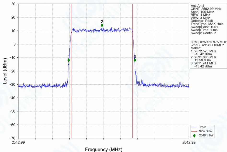
n41_30kHz_SISO_NTNV_40MHz_DFT-s-OFDM_256_QAM_2592.99MHz_Outer_Full_Ant1
