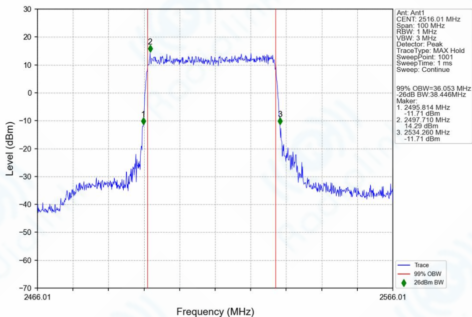
n41_30kHz_SISO_NTNV_40MHz_DFT-s-OFDM_64_QAM_2516.01MHz_Outer_Full_Ant1
