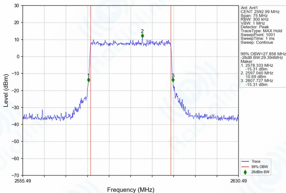
n41_30kHz_SISO_NTNV_30MHz_CP-OFDM_16_QAM_2592.99MHz_Outer_Full_Ant1
