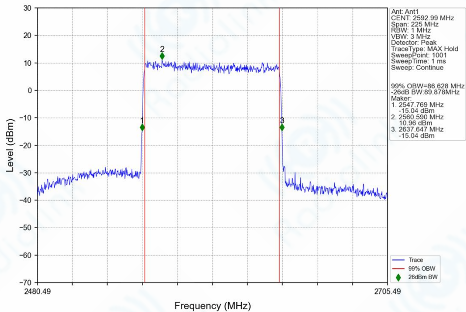
n41_30kHz_SISO_NTNV_90MHz_DFT-s-OFDM_16_QAM_2592.99MHz_Outer_Full_Ant1
