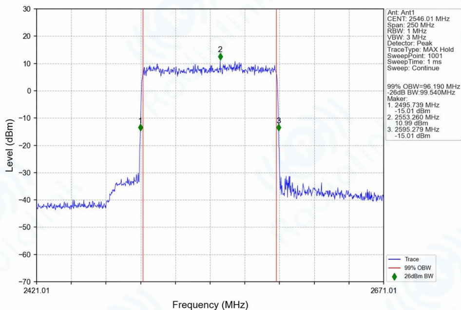
n41_30kHz_SISO_NTNV_100MHz_DFT-s-OFDM QPSK_2546.01MHz_Outer_Full_Ant1
