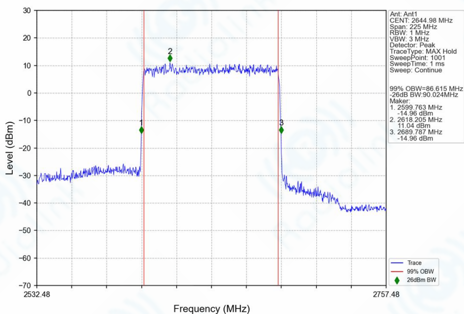
n41_30kHz_SISO_NTNV_90MHz_DFT-s-OFDM_64_QAM_2644.98MHz_Outer_Full_Ant1
