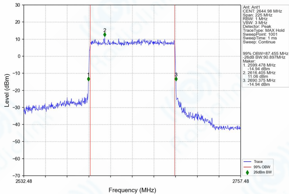
n41_30kHz_SISO_NTNV_90MHz_CP-OFDM_64_QAM_2644.98MHz_Outer_Full_Ant1
